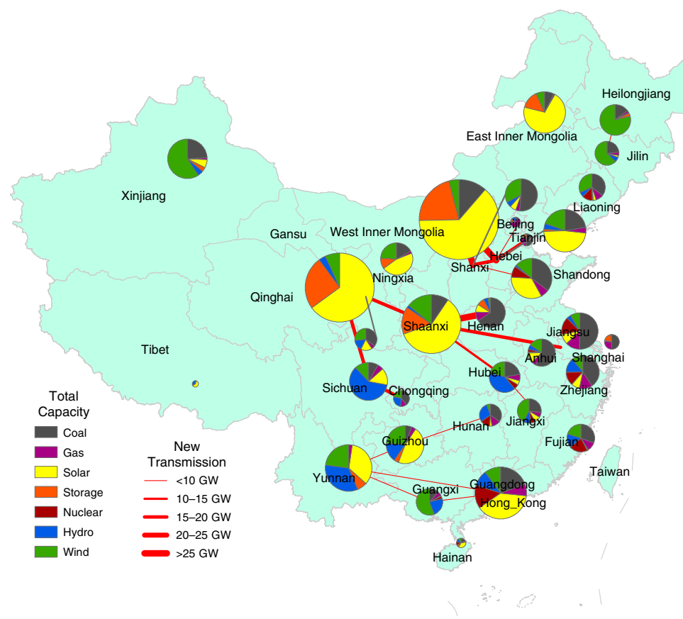
Fig. 6 Provincial total capacity mix and new transmission lines required by 2030 under the R scenario. The pie charts show the total power capacity mix in each province, and the red lines show the new interprovincial transmission lines to bring electricity from resource centers to demand centers. Source data are provided as a Source Data file.
