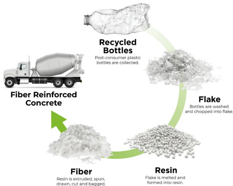
Figure 3.4: Manufacturing process of PSI FIBERSTRAND REPREEVE 225.
