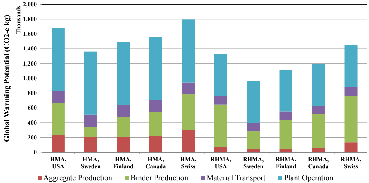
Figure 7.8: KER-5 Material Production Phase: GHG emissions for the functional unit (metric tons).
