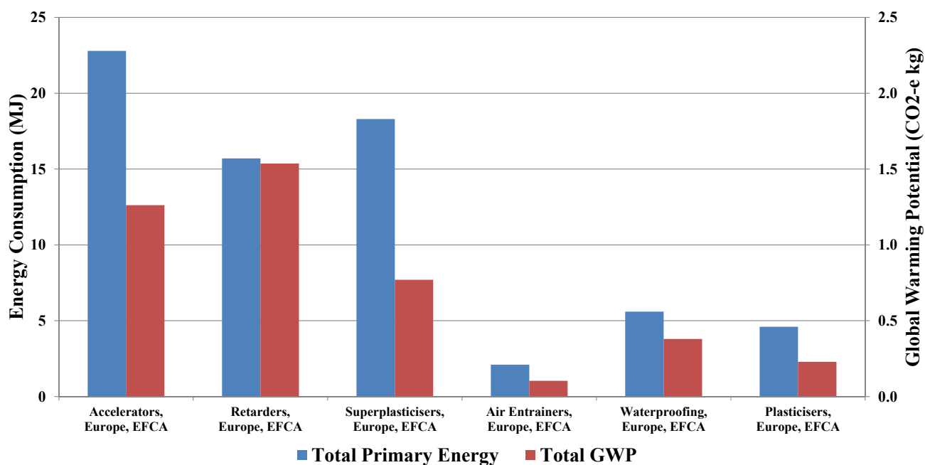
Figure 4.8: Concrete admixtures production, at plant (1 kg).
