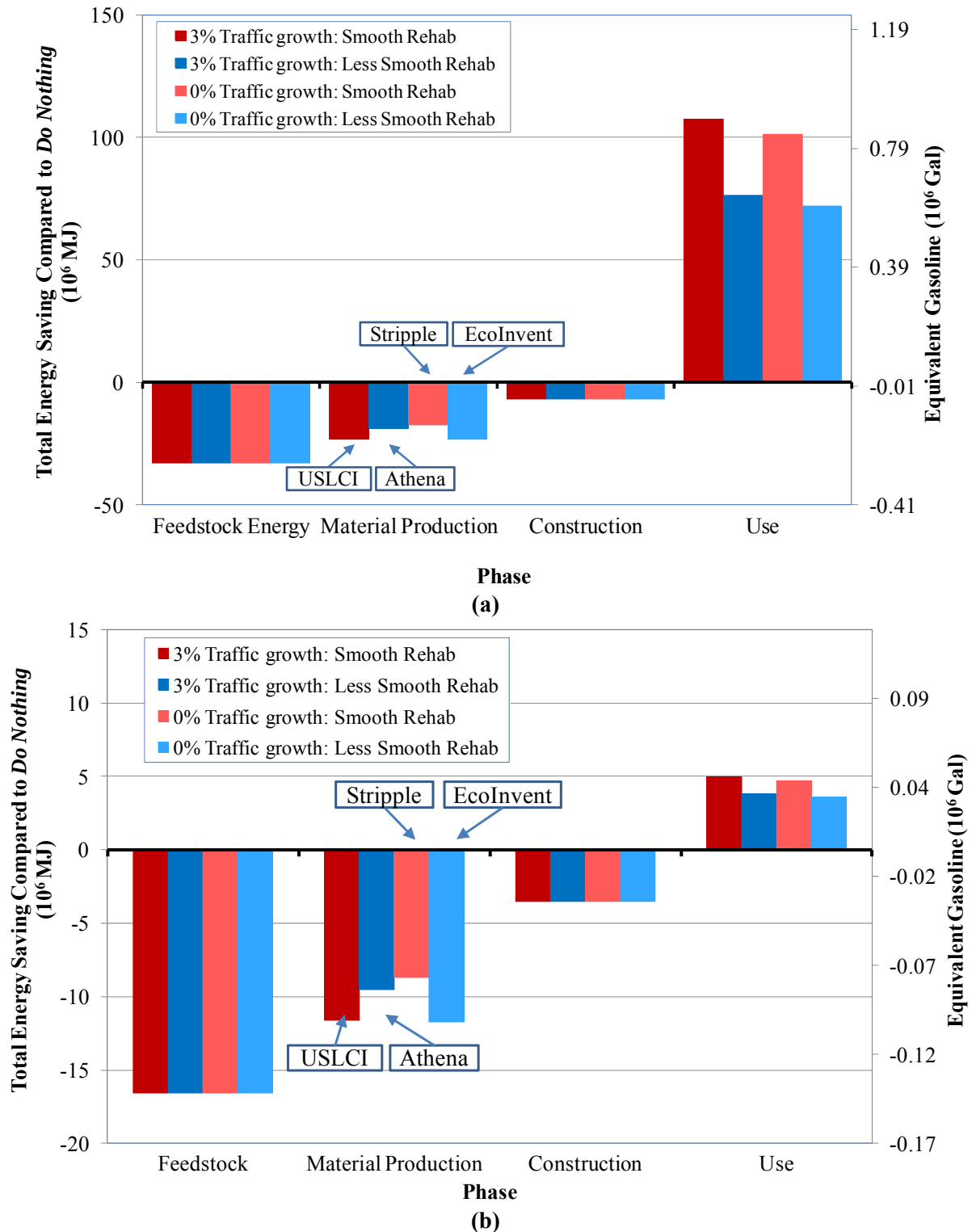
Figure 7.17: (a) Analysis period energy saving compared to Do Nothing with HMA overlay in KER-5; (b) Analysis period energy saving compared to Do Nothing with HMA overlay in BUT-70.
