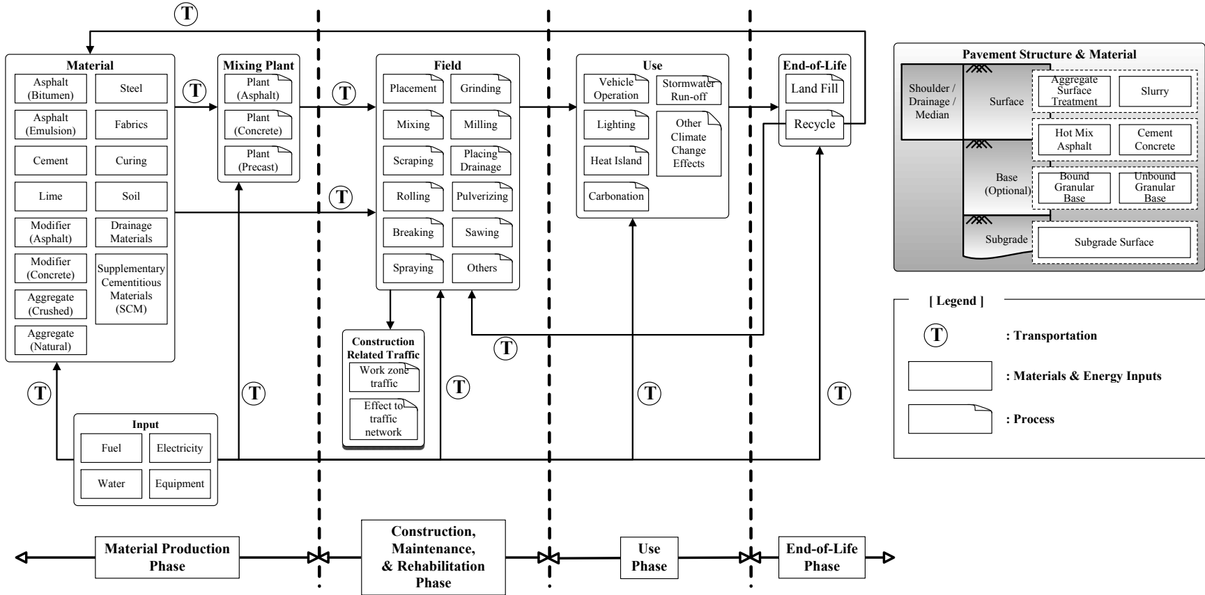
Figure 3.1: UCPRC Pavement LCA Framework.
