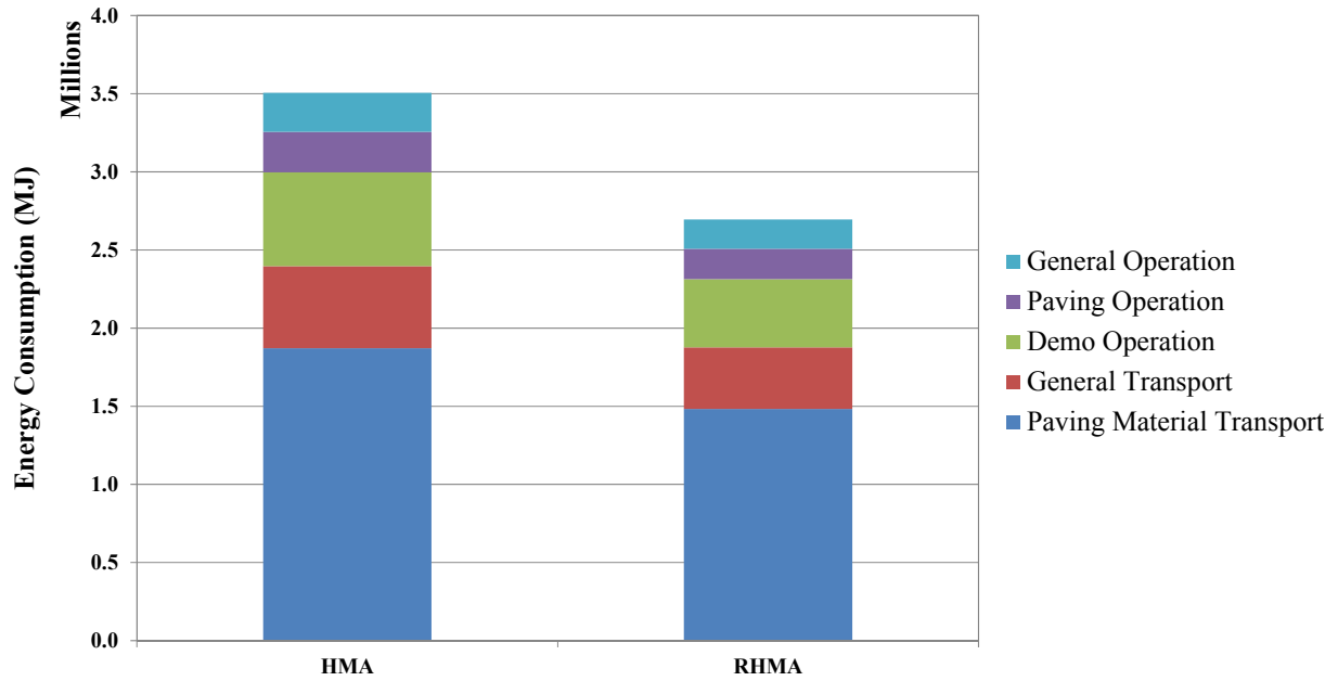
Figure C.3: BUT-70 Construction Phase: energy consumption for the functional unit.
