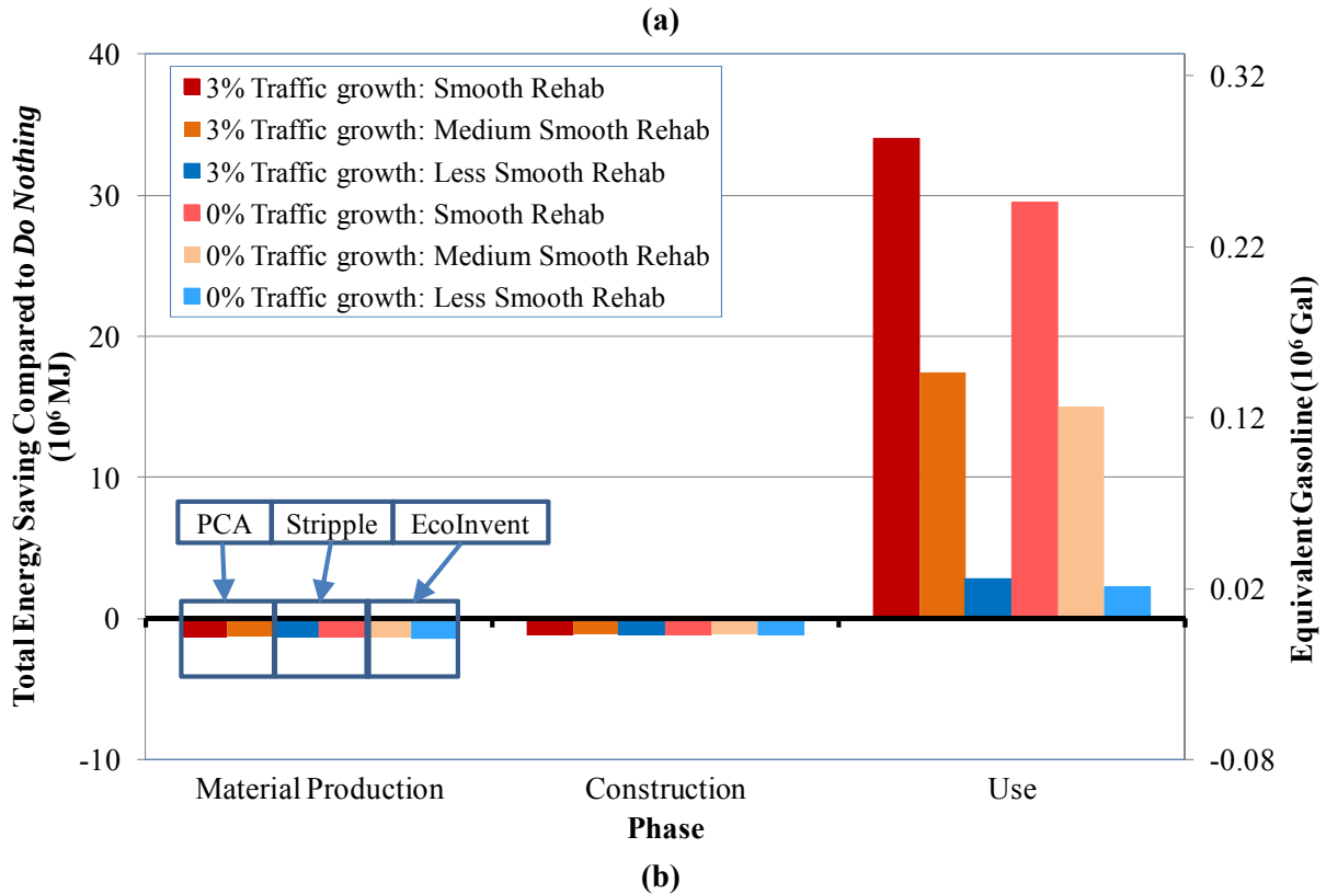
Figure 7.18: (a) Analysis period energy saving compared to Do Nothing with Type III PCC in LA-5; (b) Analysis period energy saving compared to Do Nothing with Type III PCC in IMP-86.
