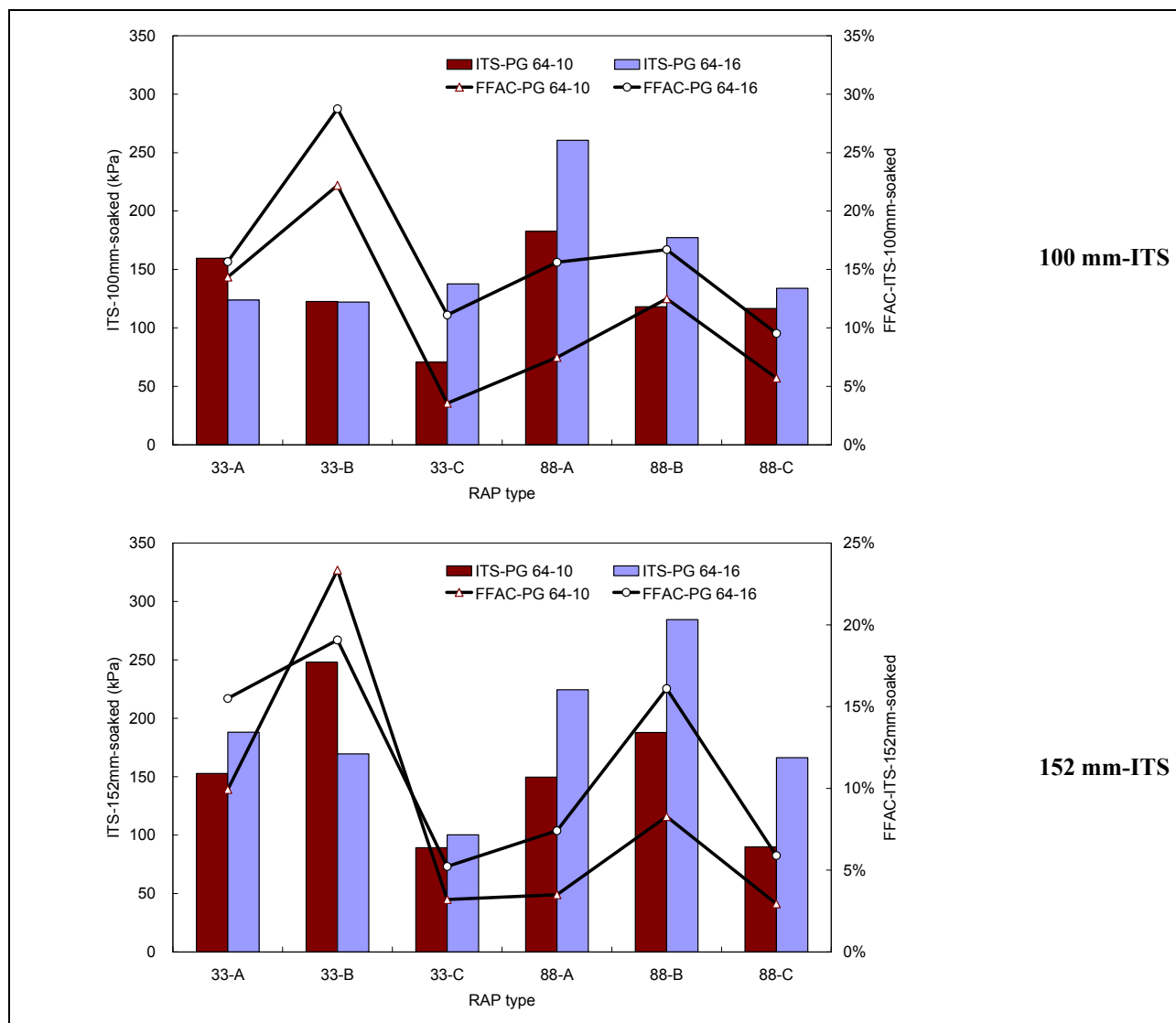
Figure 7.10: Effect of binder grade on strength.
