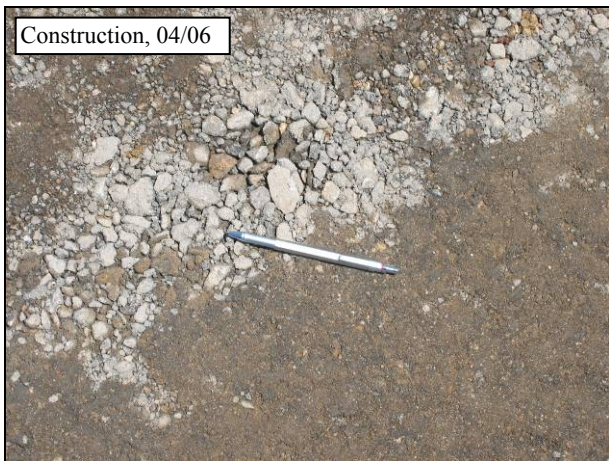
Figure 4.54: Area of segregated aggregate on 07-VEN-33.
