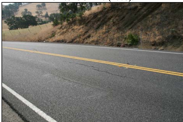
Figure 4.6: Longitudinal cracks in hill section on 03-COL-20 (2007–2008).
