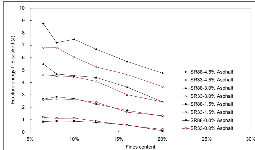
Figure 8.6: Soaked ITS fracture energy as a function of fines and asphalt content.
