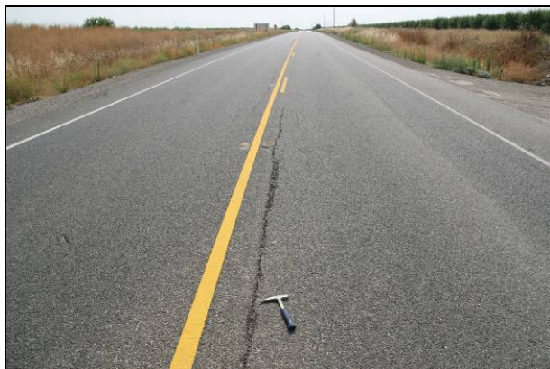
Figure 4.2: Centerline crack on 03-COL-20 (2006–2008).
