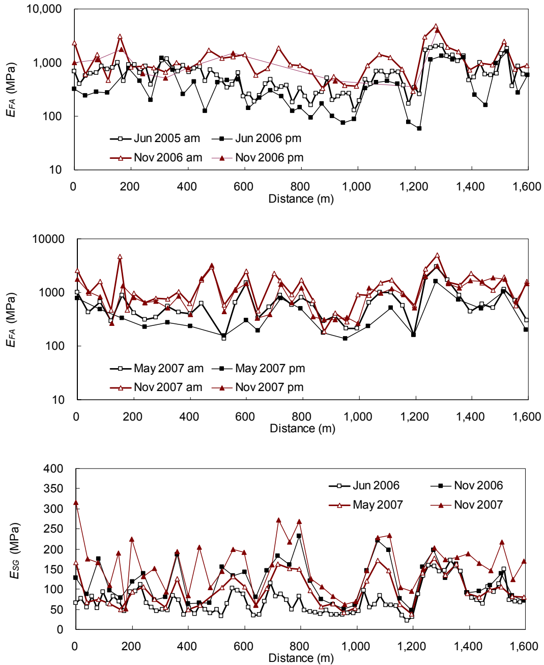
Figure A.3: Backcalculated Resilient Modulus for Section SR33-Ven-A. ([a] Foamed asphalt-treated layer in 2006; [b] foamed asphalt-treated layer in 2007; and [c] subgrade)
