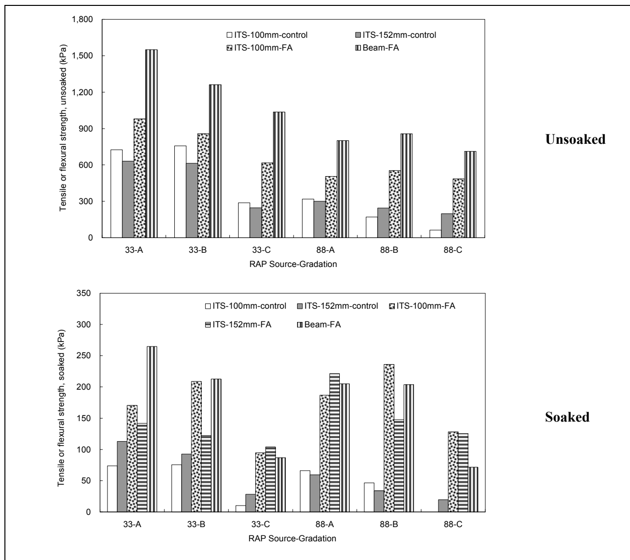
Figure 7.6: Comparison of unsoaked and soaked strength test results. (FA = foamed asphalt-treated specimens)
