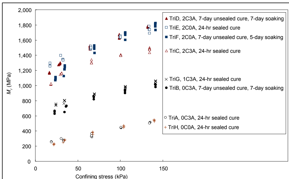
Figure 9.15: Triaxial Resilient Modulus test results under various conditions. (“XCYA” represents the mix design. For example, “2C3A” indicates that the mix contained 2% cement and 3% foamed asphalt.)
