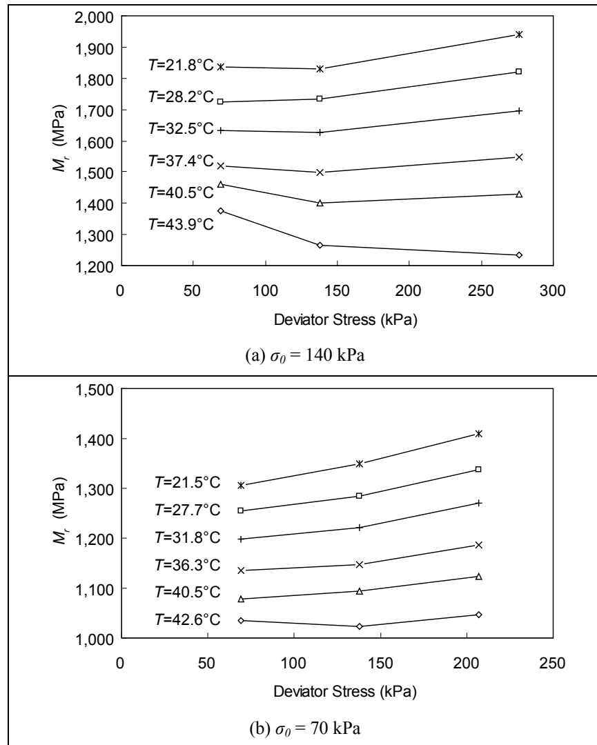
Figure 6.8: Interaction of deviator stress and temperature. (Specimen A-15)
