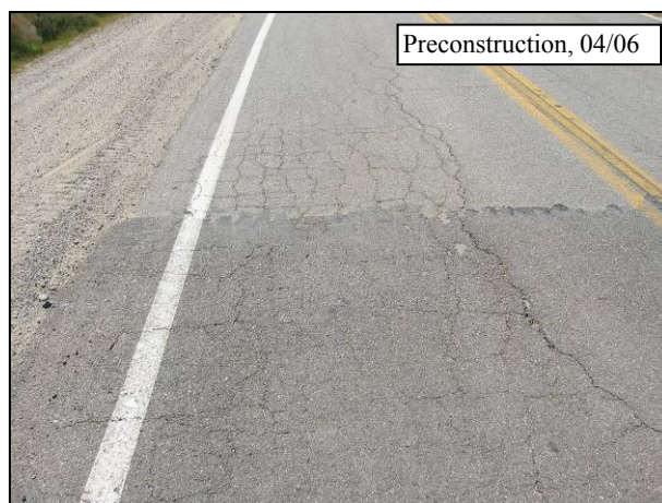
Figure 4.39: Preconstruction maintenance overlay on 07-VEN-33.
