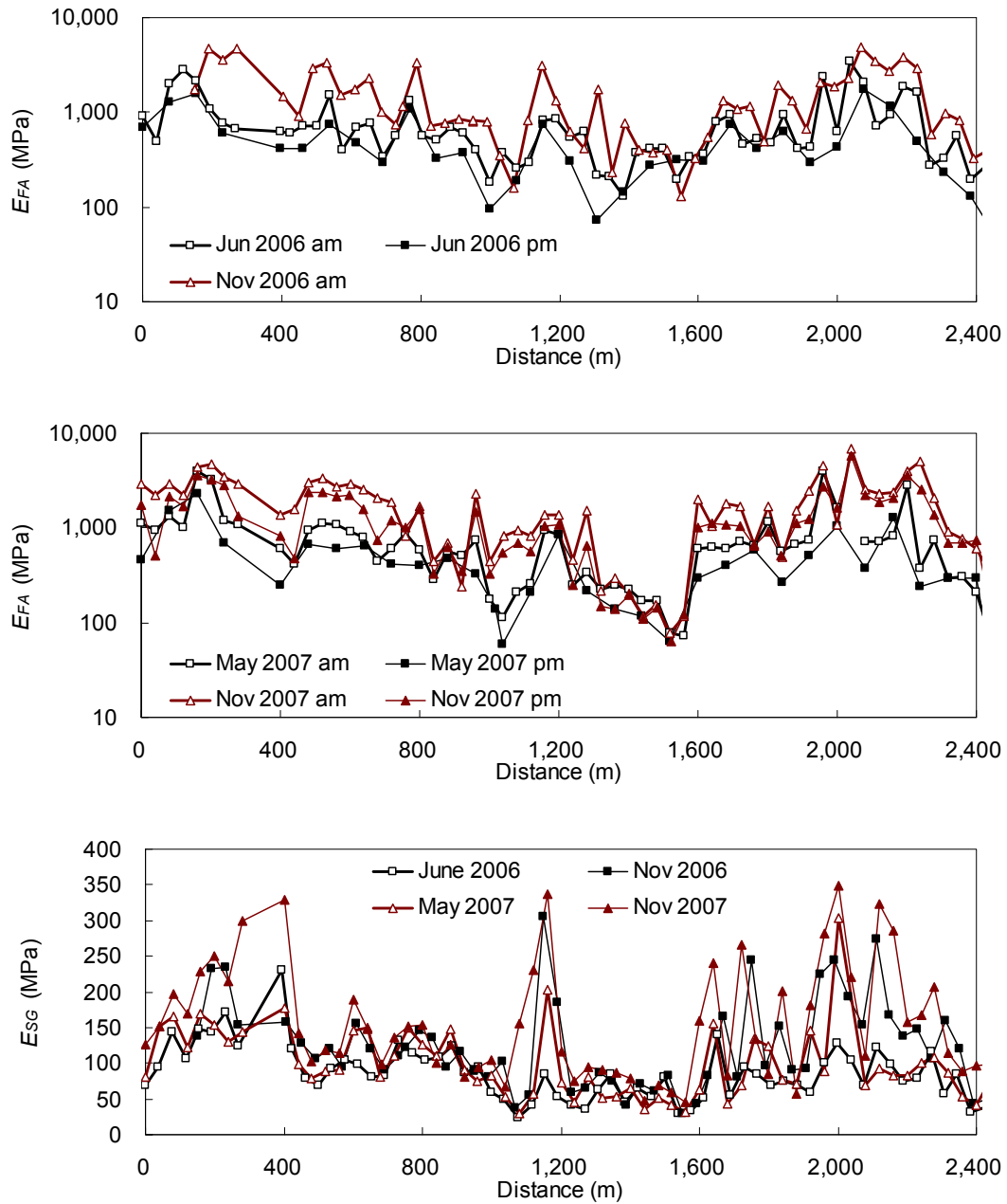
Figure A.4: Backcalculated Resilient Modulus for Section SR33-Ven-B. ([a] Foamed asphalt-treated layer in 2006; [b] foamed asphalt-treated layer in 2007; and [c] subgrade)
