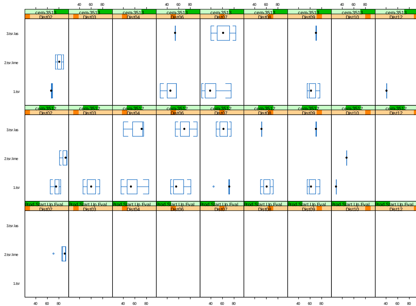
Figure 2.8: Trellis graph of CT 371-TSR value: tsr.type~tsr | dist*form.type .
