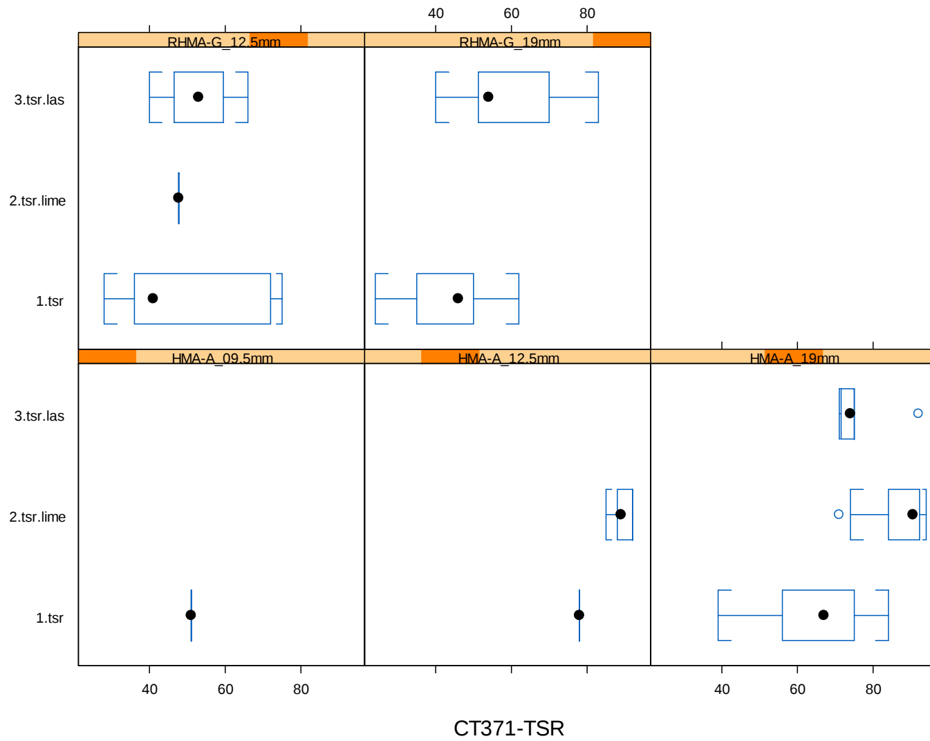
Figure 2.7: Trellis graph of CT 371-TSR value: tsr.type~tsr | mix.type .
