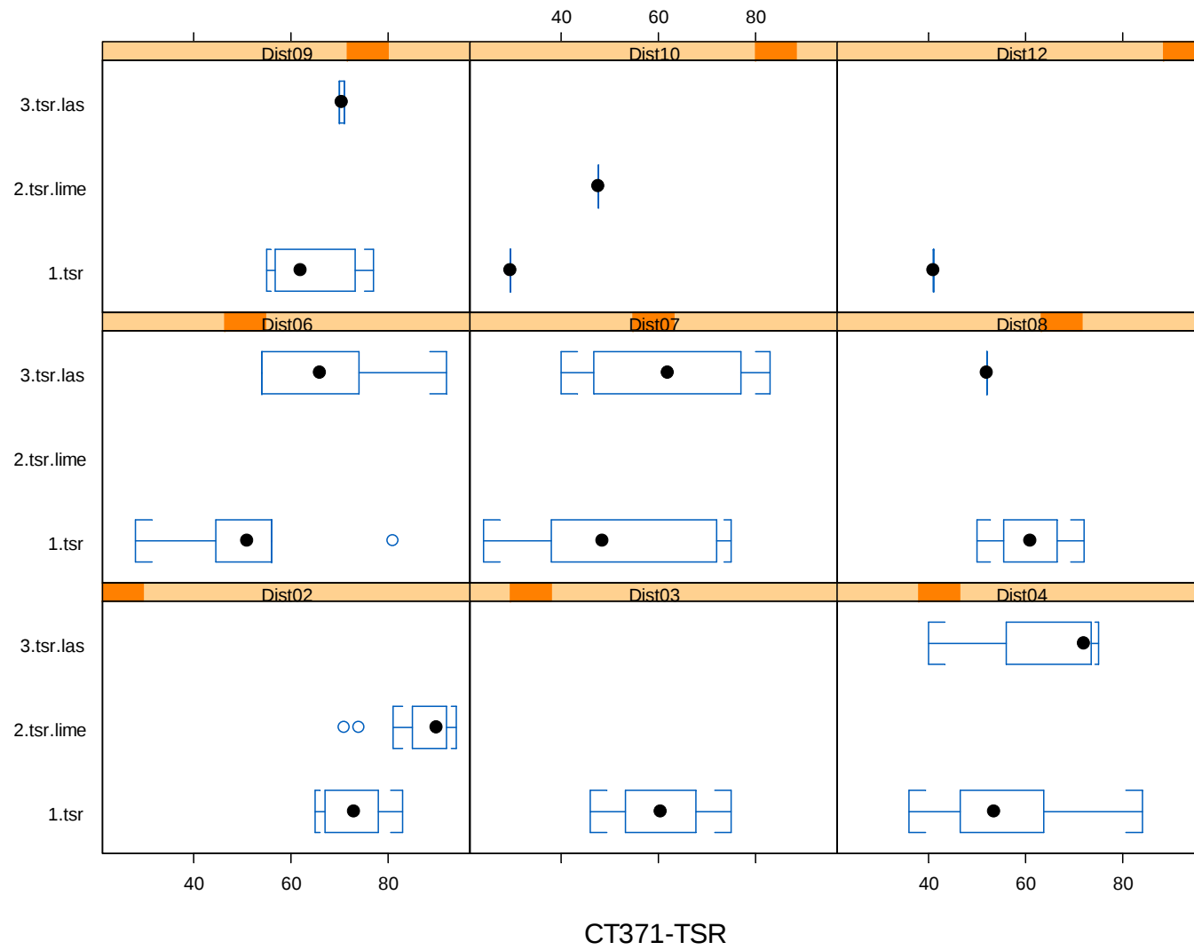
Figure 2.4: Trellis graph of CT 371-TSR value: tsr.type~tsr | dist.
