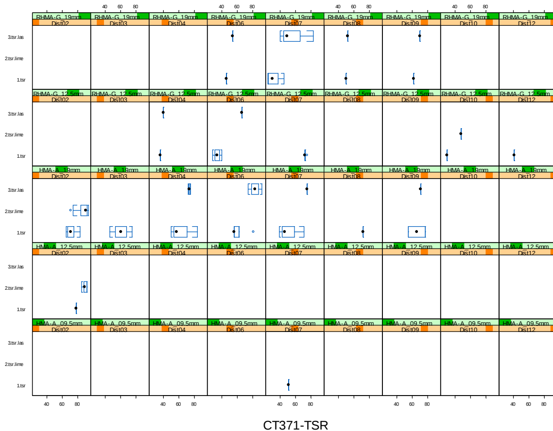
Figure 2.3: An example of Trellis graph: tsr.type~tsr | dist*mix.type .
