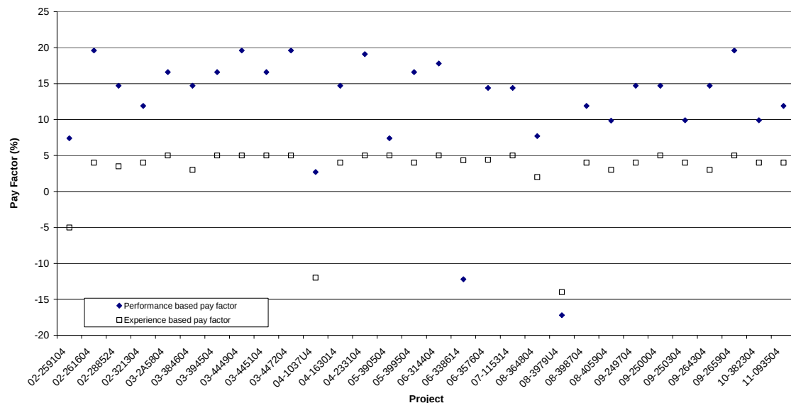
Figure 10. Variation of pay factor values when rutting is the predicted distress.
