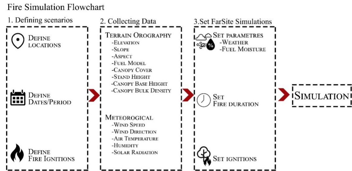
Figure 2. Framework of Fire Simulation
