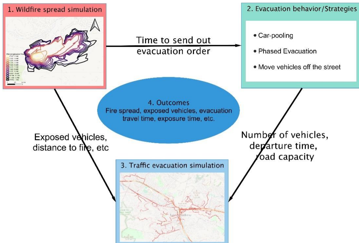
Figure 1. Study Flowchart
