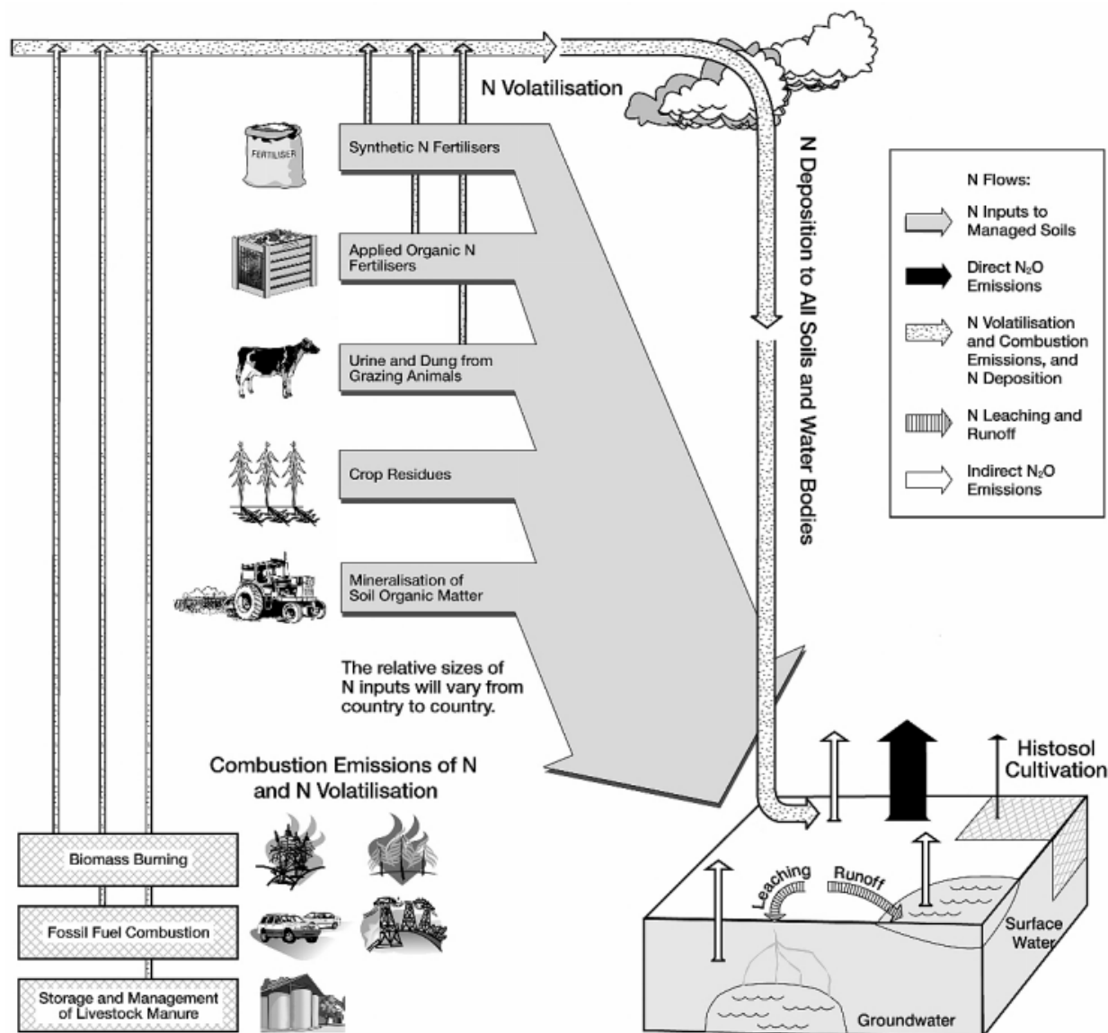
Figure 4. Schematic diagram illustrating nitrogen sources and pathways that result in direct and indirect N 2 O emissions from soils and waters.
