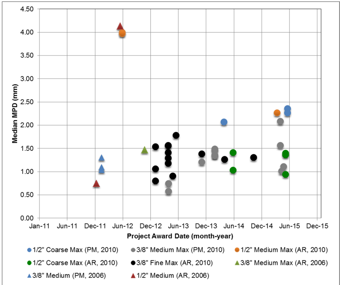
Figure 6.11: MPD results measured in fall 2015 plotted by project award date. (Note: Asphalt rubber binder [AR], polymer-modified binder [PM], 2006 Standard CT Specification [2006], 2010 Standard CT Specification [2010])
