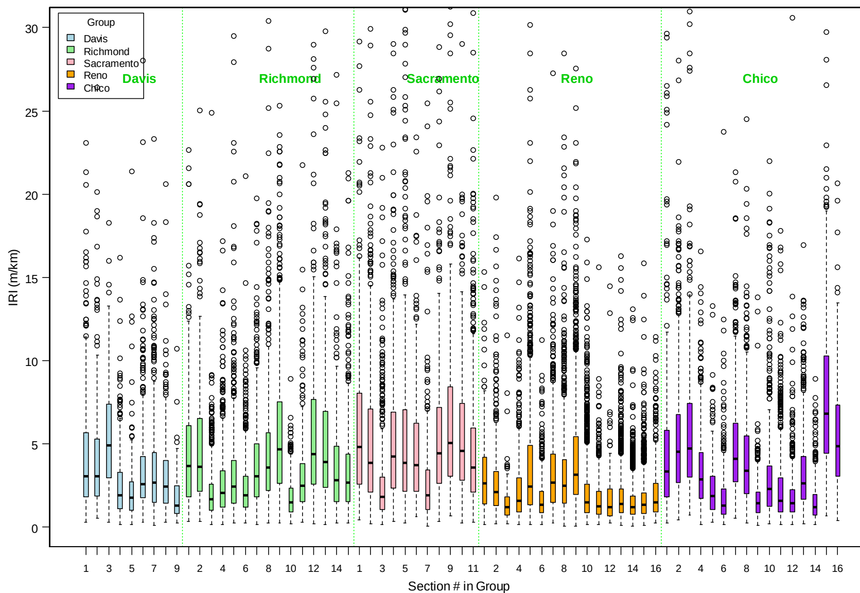
Figure 4.4: Summary box plots of IRI for all the survey sections in all groups. (Note: 1 m/km = 63.4 inches/mile)
