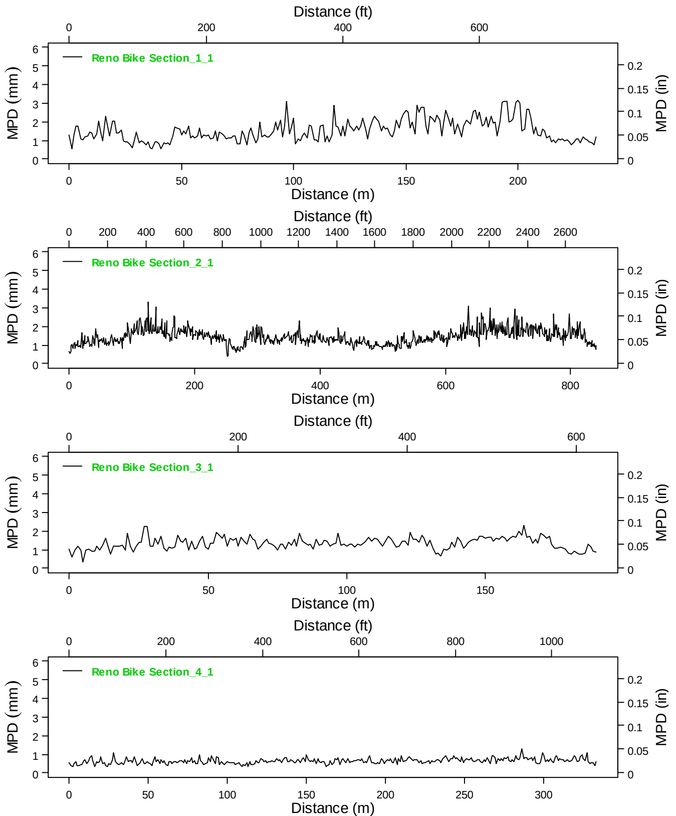
Figure B.11: Macrotexture measured using IP on Reno survey Sections 1 to 4.
