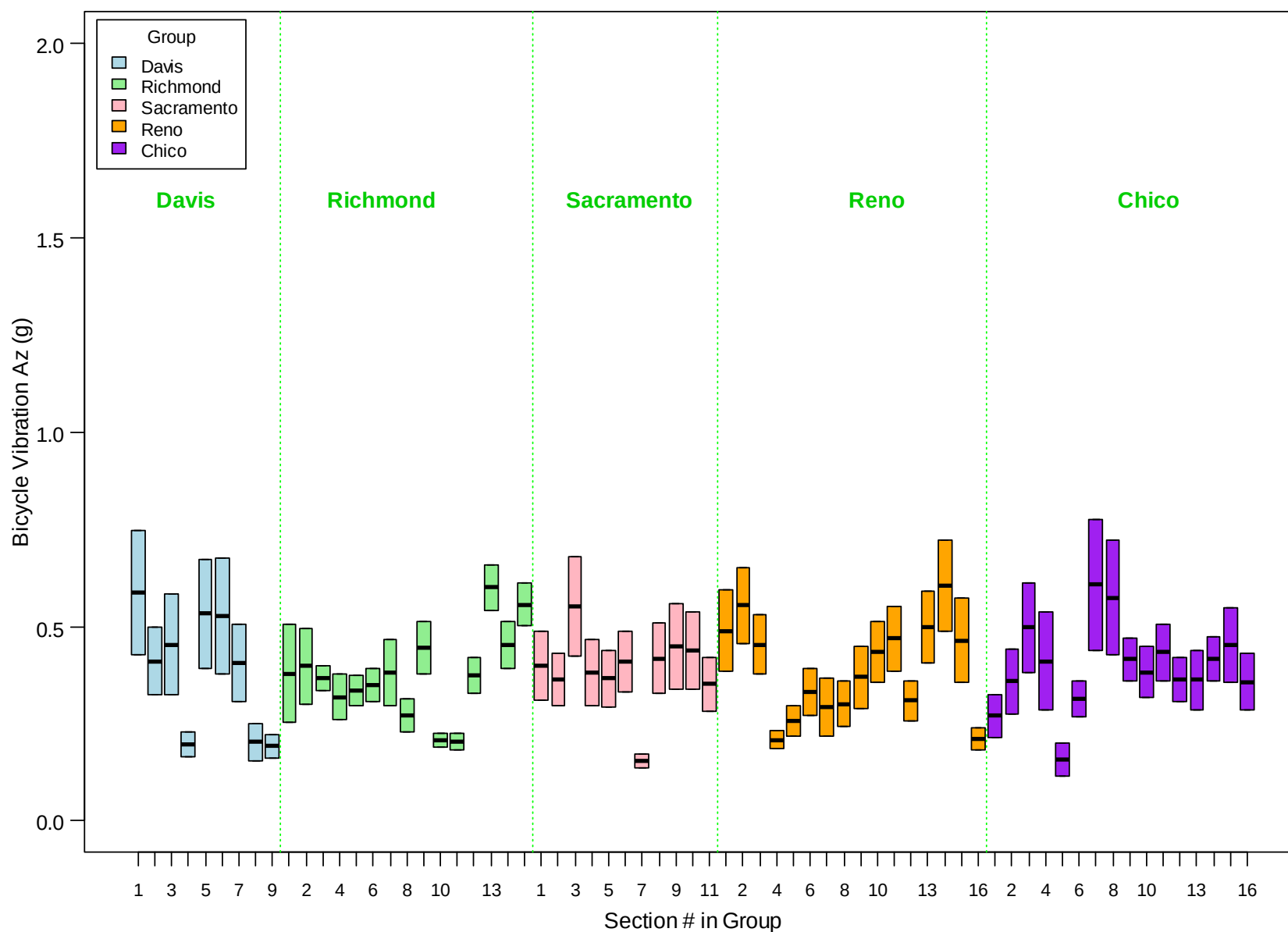
Figure 4.6: Summary box plots of commuter bicycle vibration for survey sections across all cities.
