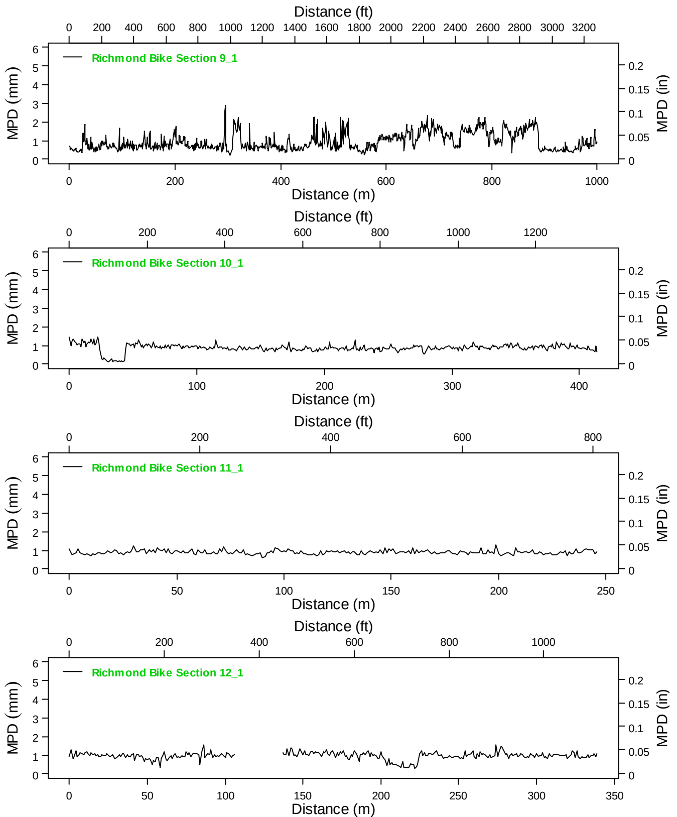
Figure B.6: Macrotexture measured using IP on Richmond survey Sections 9 to 12.
