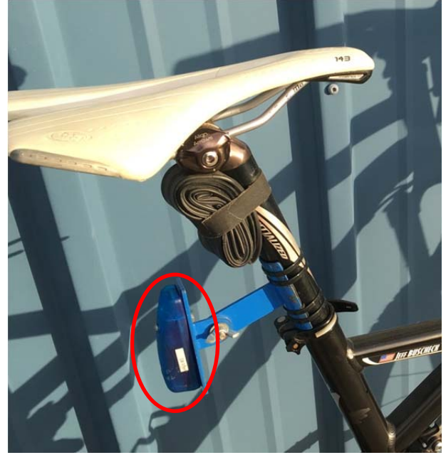
Figure 3.10: Detail of rear of mountain bicycle instrumented with accelerometer (solid red circle) at the seatpost mounting location.
