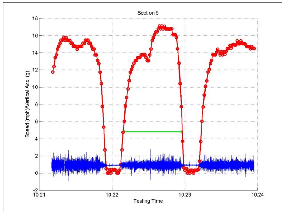
Figure 3.11: Example extract of bicycle speed with corresponding acceleration data. (Note: the red line with circles shows speed (mph), the blue line shows acceleration ( g ), and the green line shows the test section portion used for analysis where speed > 5 mph.)
