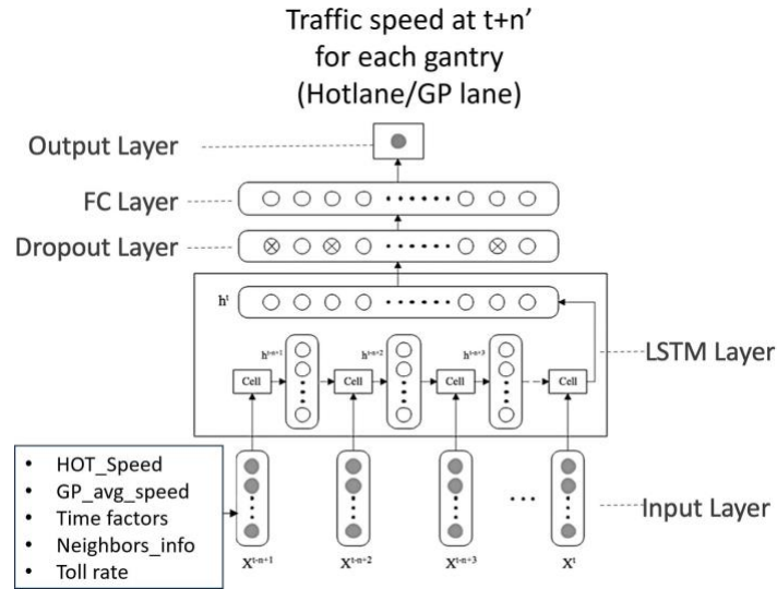
Figure 3. Architecture of the proposed traffic speed forecasting framework
