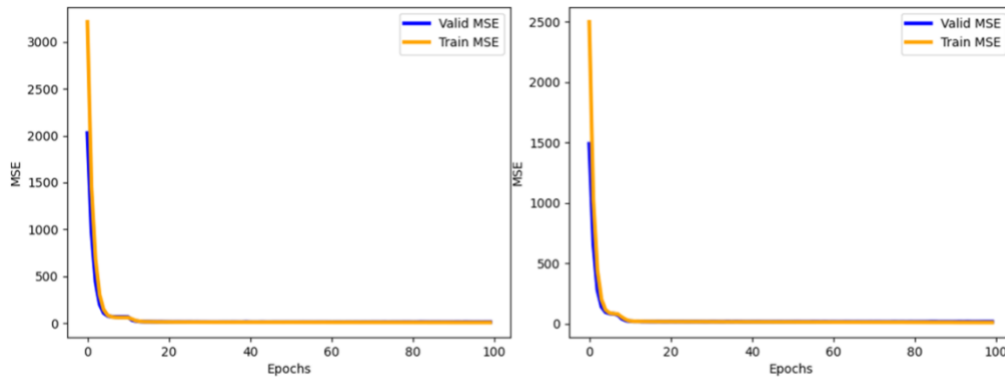
Figure 9. Training and evaluation loss for HOT-lane (left) and GP-lane (right) speed prediction
