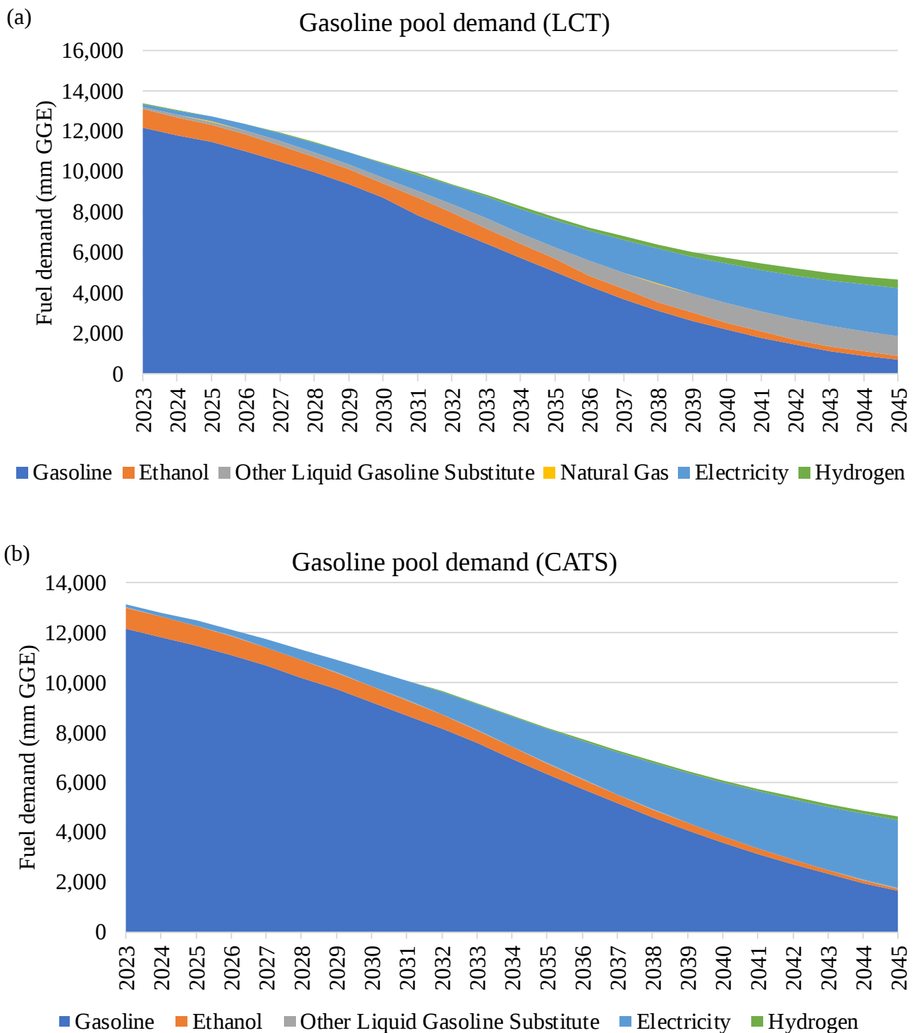
Figure 16. Gasoline pool demand projections for (a) LCT scenario with the default control parameters in the FPSM and (b) CATS scenario with the CATS control parameters.
