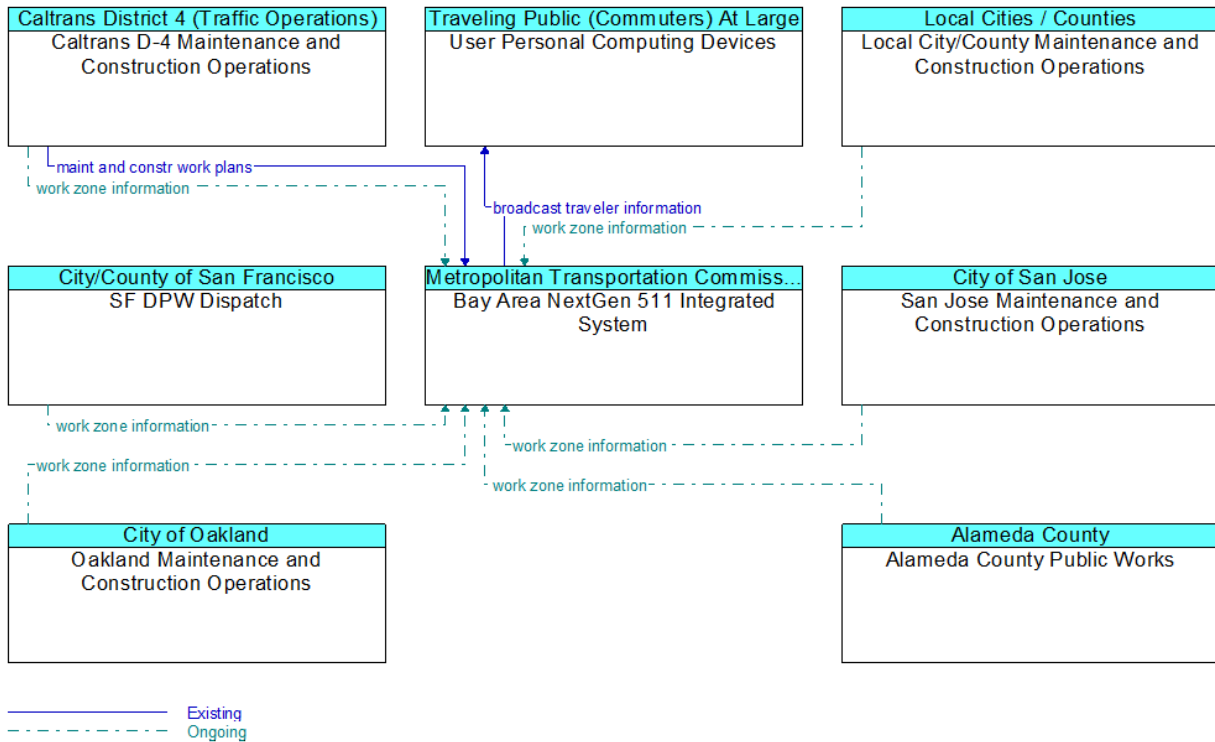
Figure 5-6: RITSA Diagram of Broadcast Traveler Information (8)
