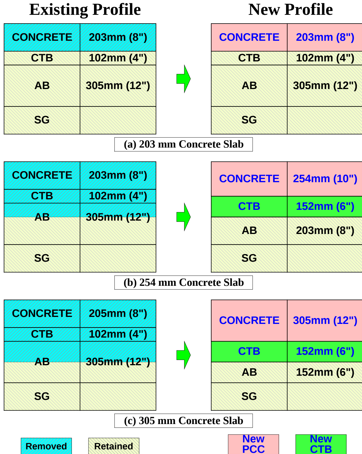
Figure 5. Change of design profiles for different slab thickness.
