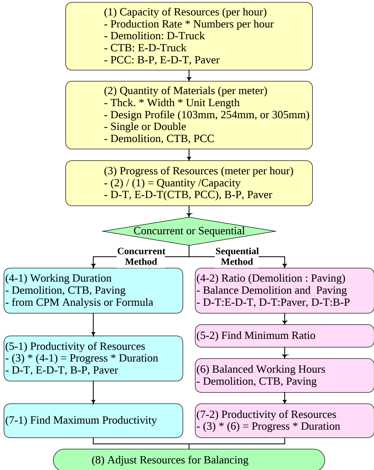
Figure 13. Processes of linear scheduling.
