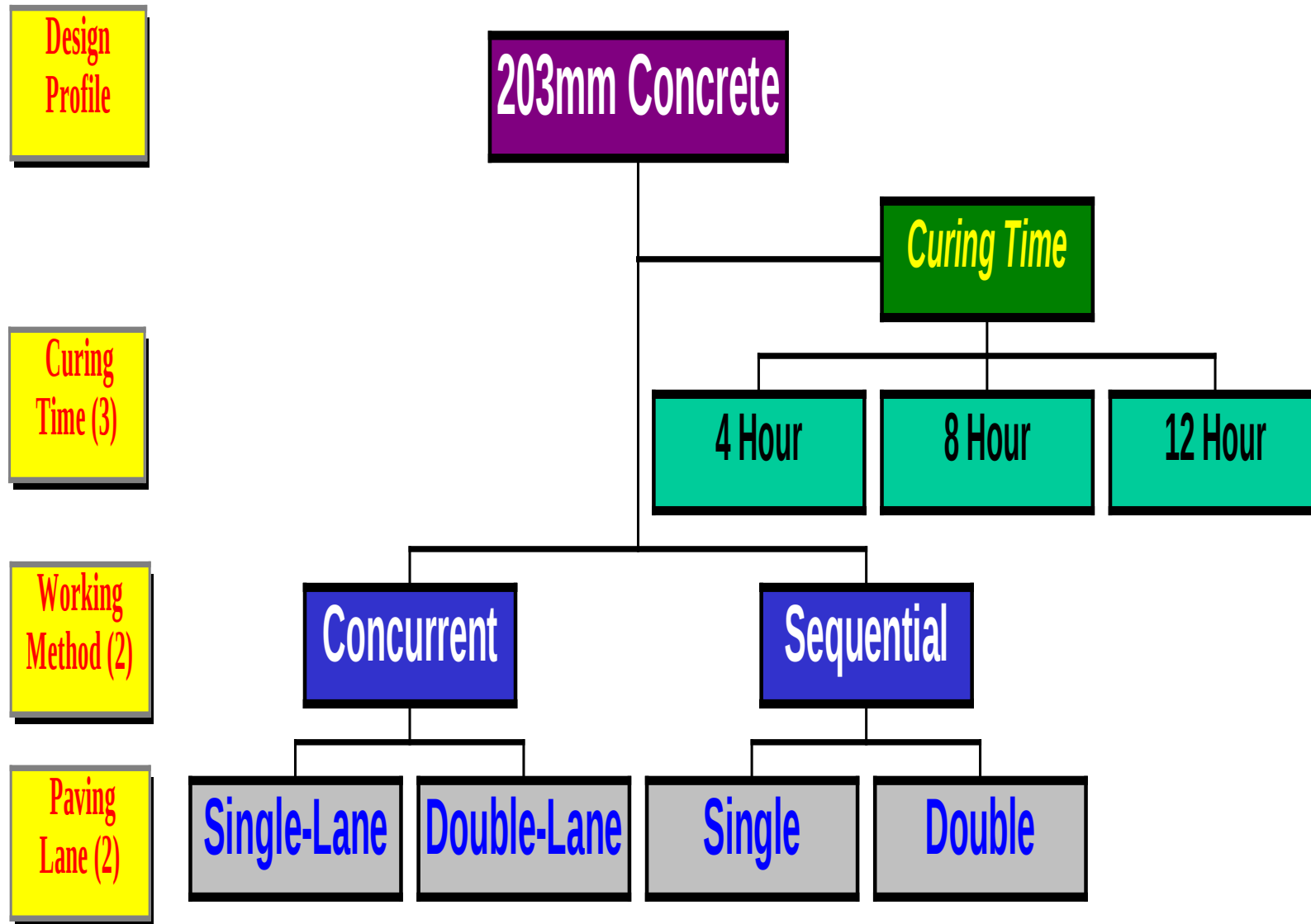
Figure 4. Options analyzed for each design profile for concrete rehabilitation.
