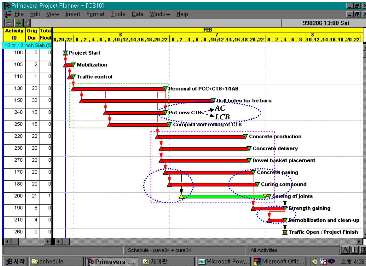
Figure 10. Typical CPM schedule for sequential working method (254-mm or 305-mm concrete slab).
