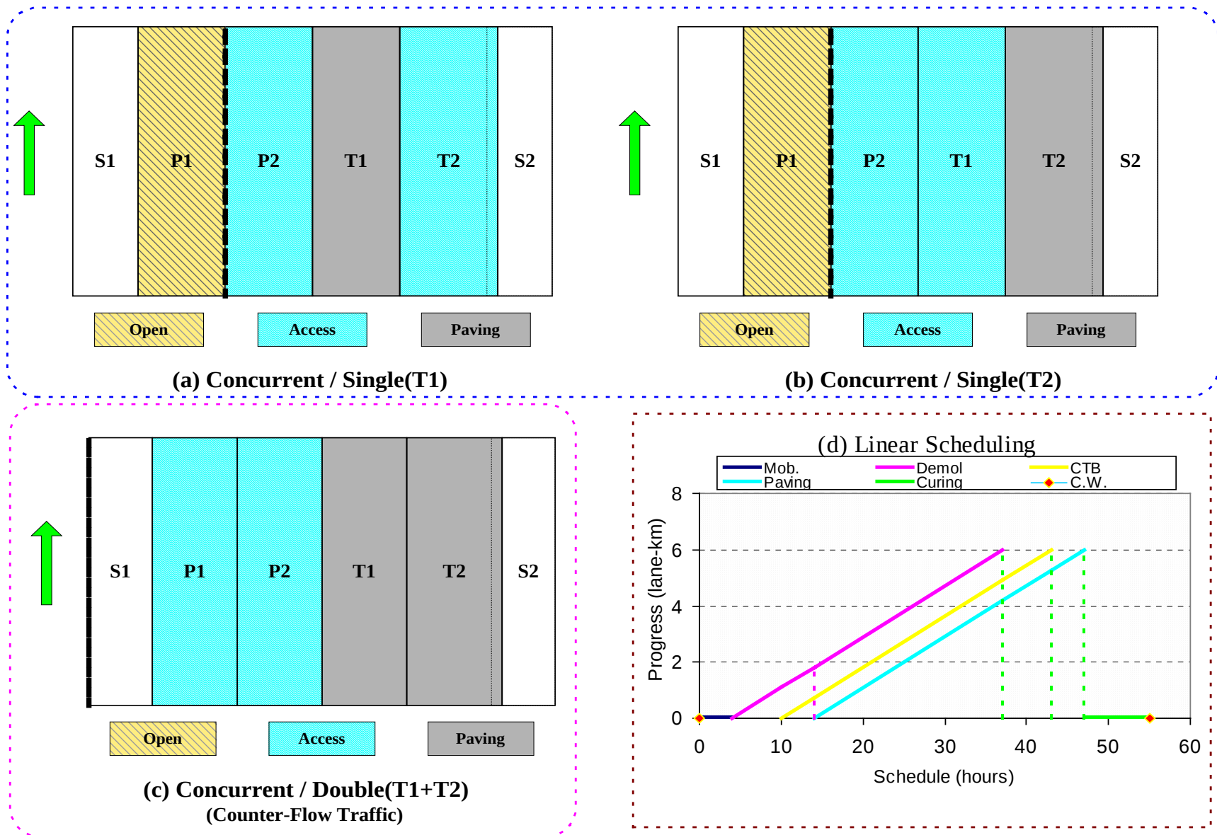
Figure 6. Work plan for concurrent working method.
