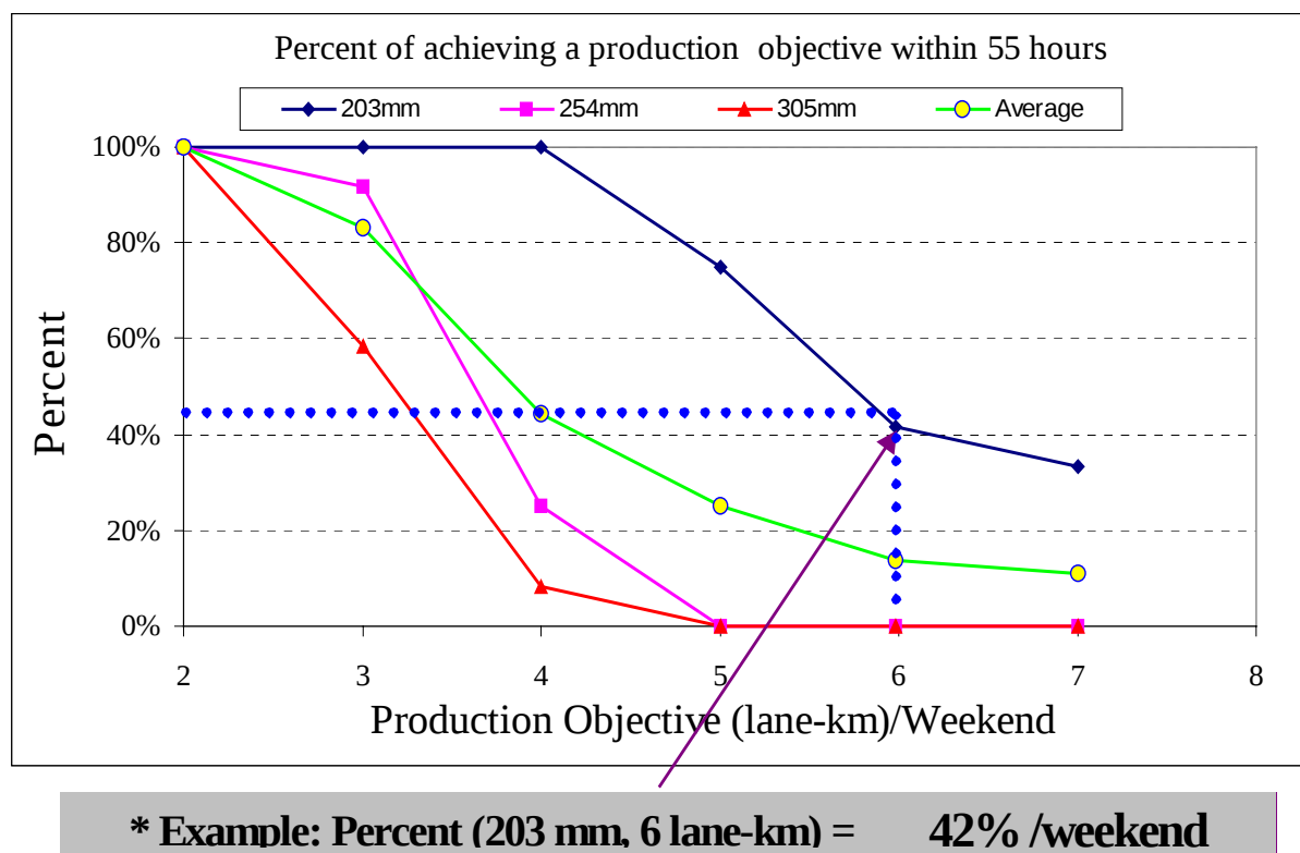
Figure 18. Percent of cases analyzed achieving a production objective within 55 hours.
