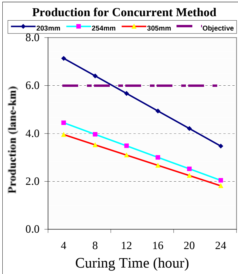
Figure 14. Single-lane production capability (lane-km) graphs.
