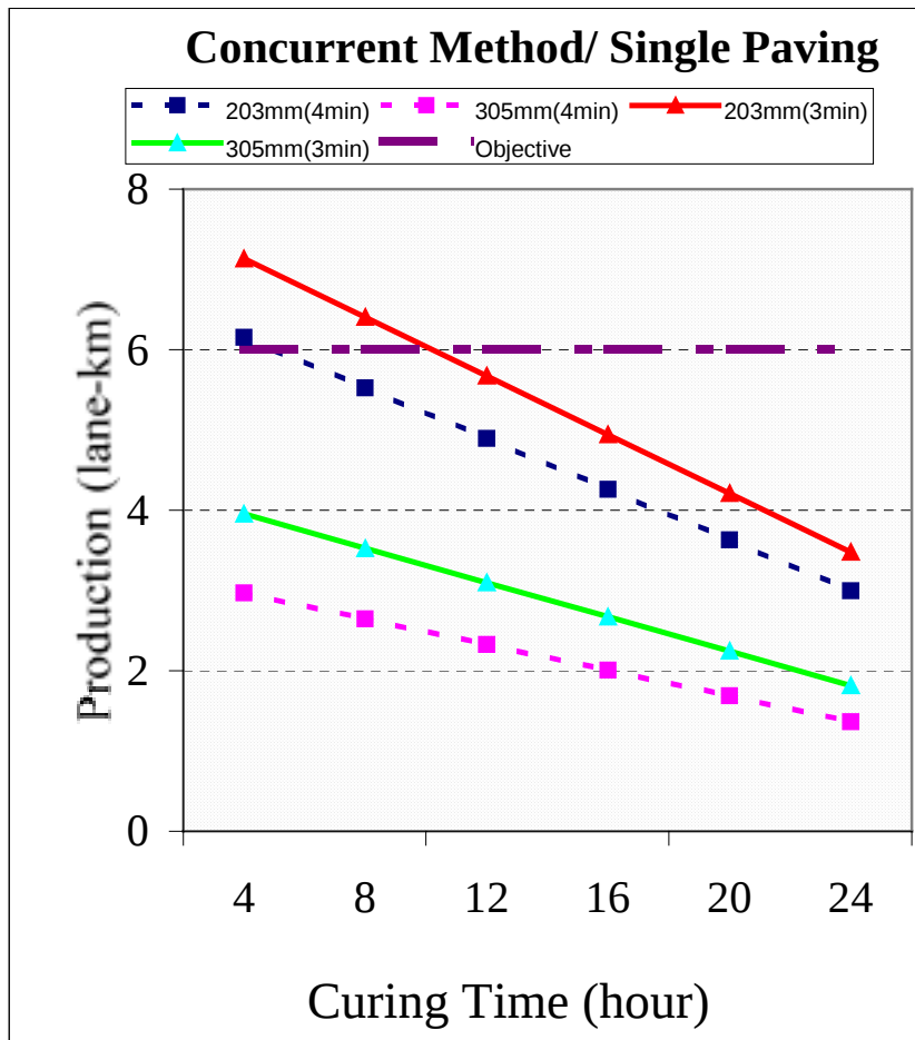
Figure 17. Reduction of production capability (lane-km) by changing the number of trucks from 20 (Cycle=3 min.) to 15 (Cycle=4 min.) per hour.
