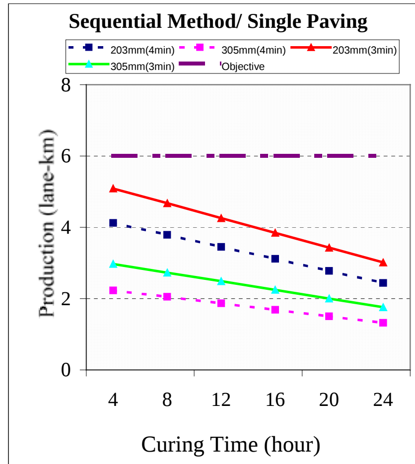
Figure 17. Reduction of production capability (lane-km) by changing the number of trucks from 20 (Cycle=3 min.) to 15 (Cycle=4 min.) per hour.
