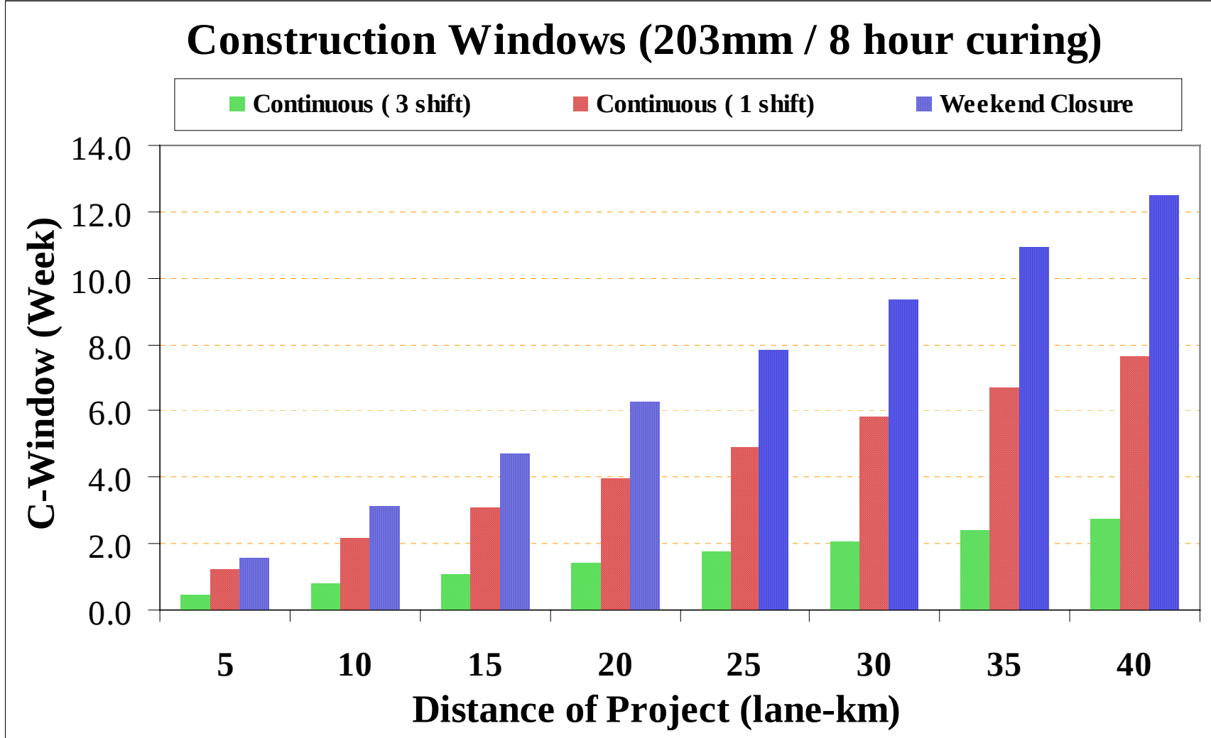
Figure 22. Construction windows covering any range of rehabilitation projects (203-mm slab/8-hour curing time/concurrent working method/single lane paving).
