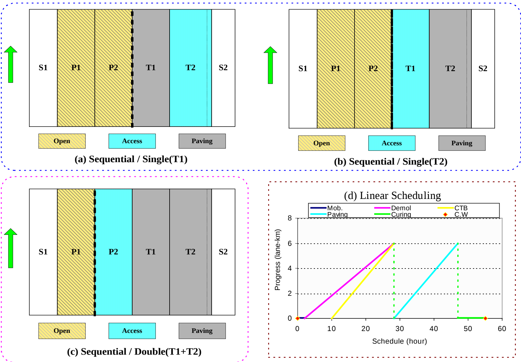
Figure 7. Work plan for sequential working method.
