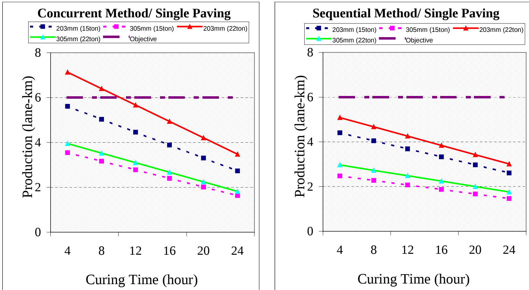
Figure 16. Reduction of production capability (lane-km) by changing the capacity of end dump trucks from 22 tons to 15 tons.
