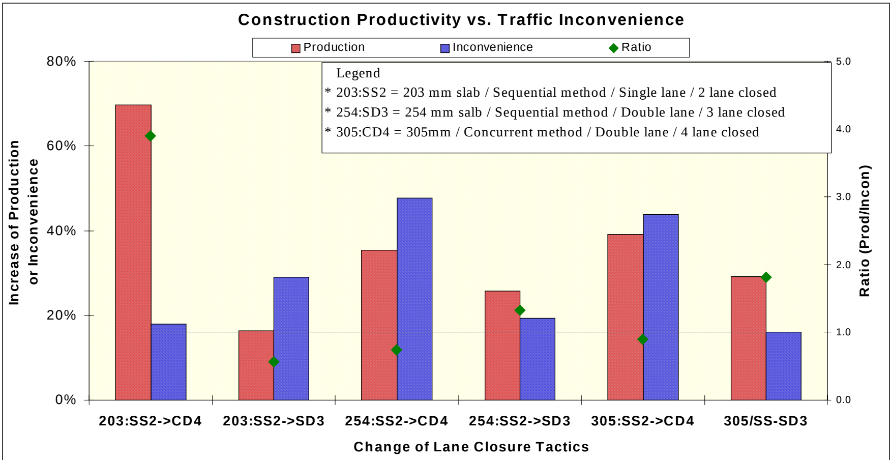
Figure 19. Comparison of increase between production and inconvenience.
