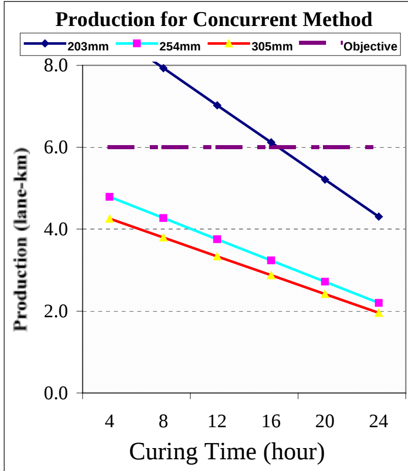
Figure 15. Double-lane production capability (lane-km) graphs.
