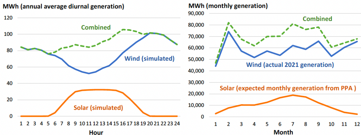
Figure 11. Annual average diurnal and monthly generation of Wheatridge wind+PV+storage plant (Bolinger et al., 2023). Results do not include battery charging or discharging.
