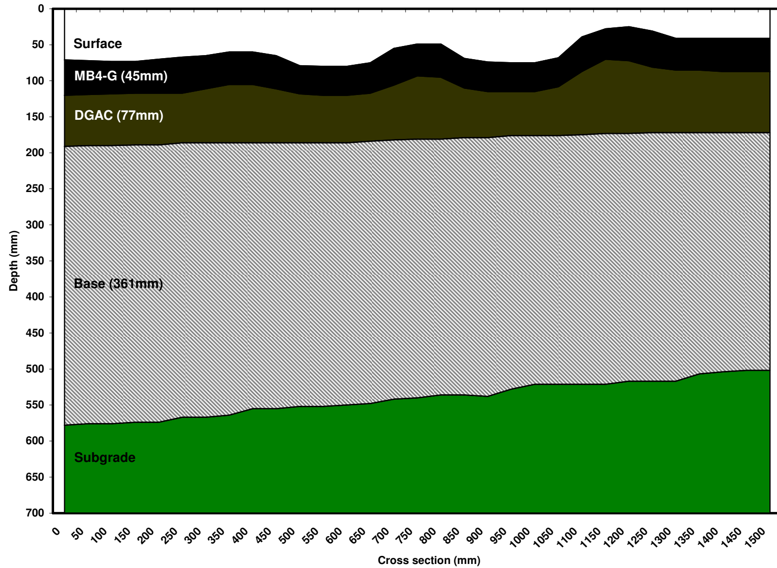
583RF #8 (45mm MB4-G) Cross Sectional Profile (15,000 reps)
