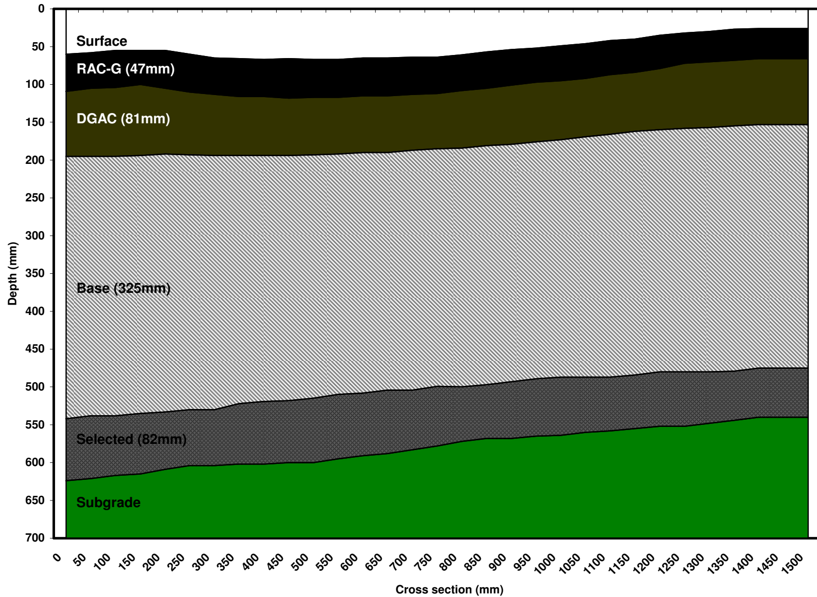
587RF #4 (45mm RAC-G) Cross Sectional Profile (2,024,793 reps)
