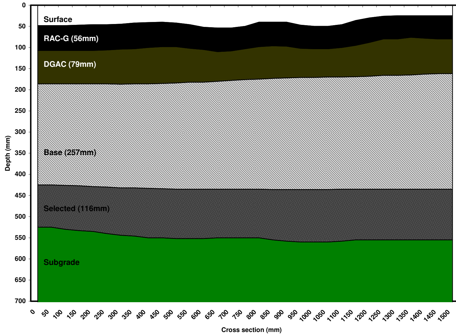
581RF (45mm RAC-G) Cross Sectional Profile (7,600 reps)
