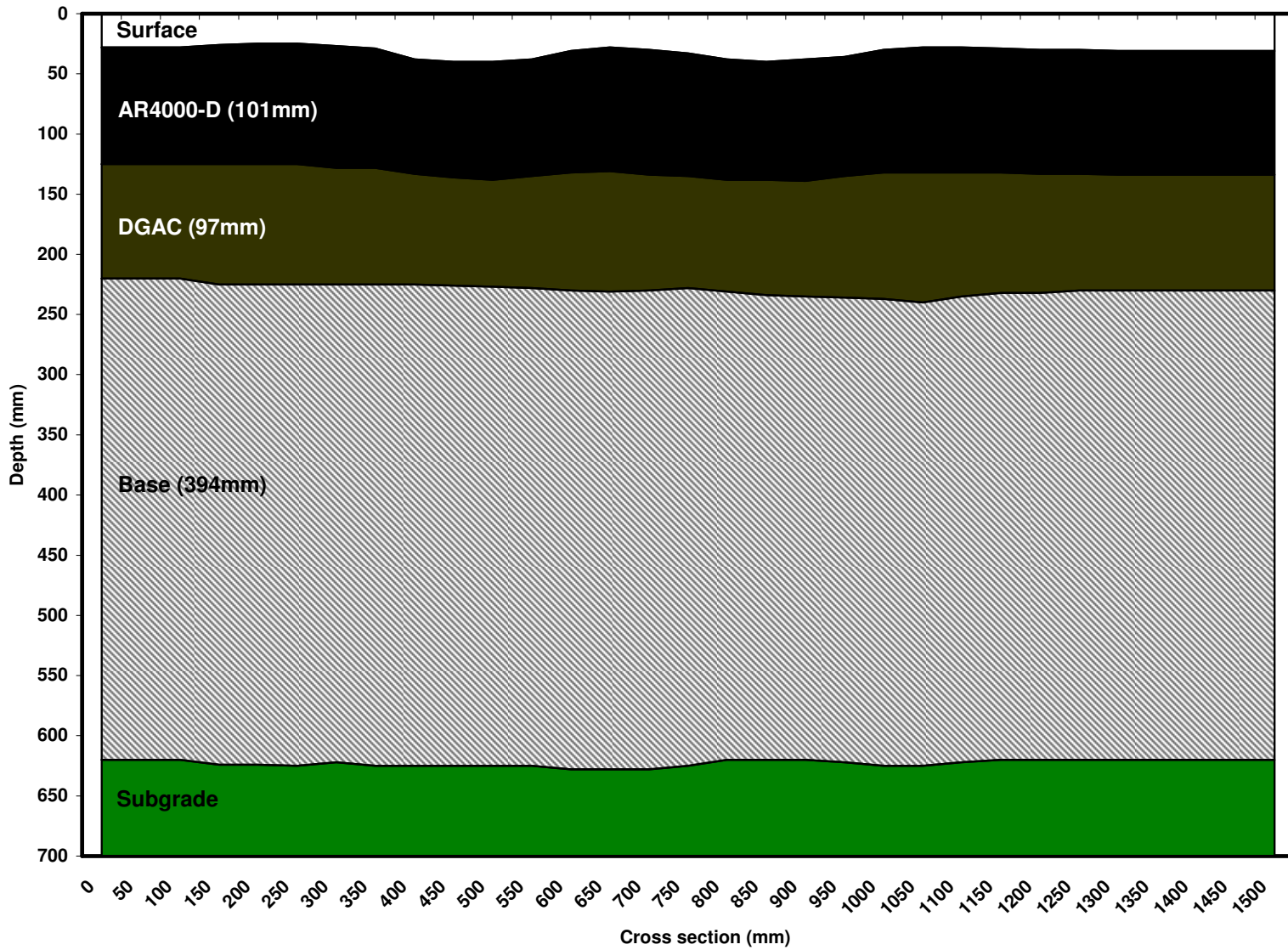
582RF (90mm AR4000-D) Cross Sectional Profile (18,564 reps)
