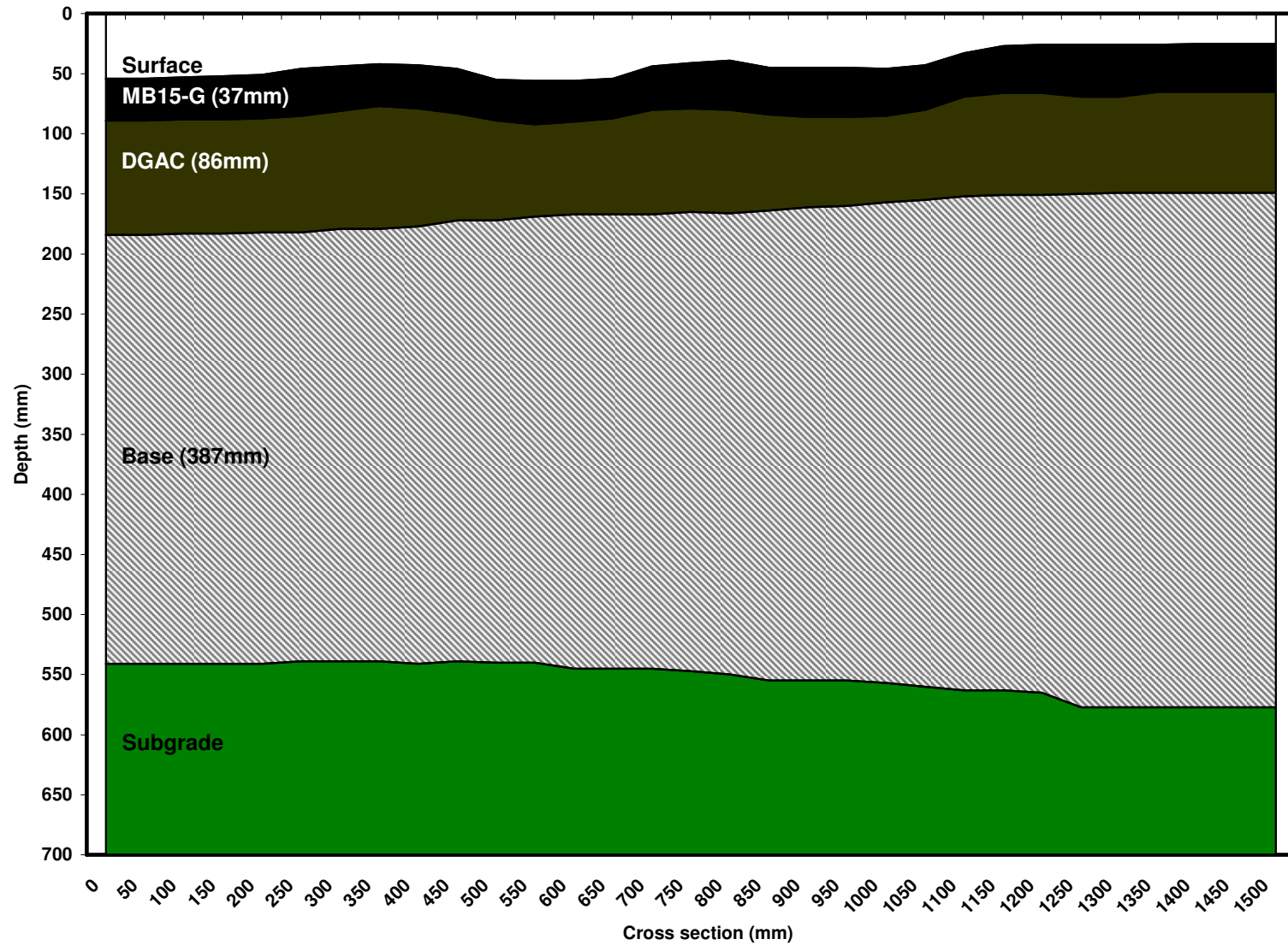
580RF (45mm MB15-G) Cross Sectional Profile (2,000 reps)
