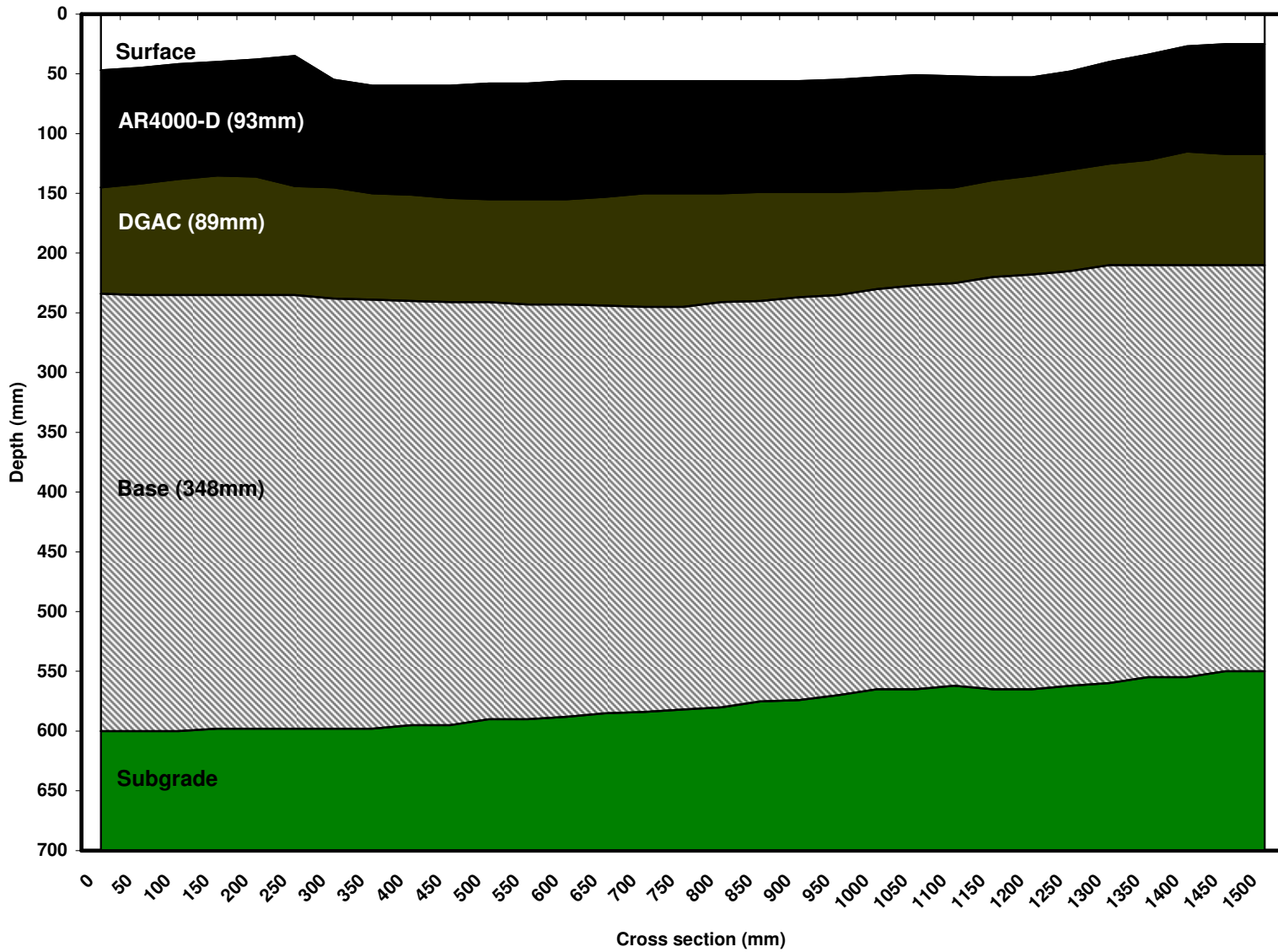
588RF #12 (90mm AR4000-D) Cross Sectional Profile (1,410,000 reps)
