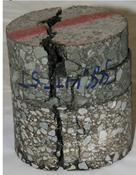
Figure 3.73: AR4000-D: Cracks on core.
