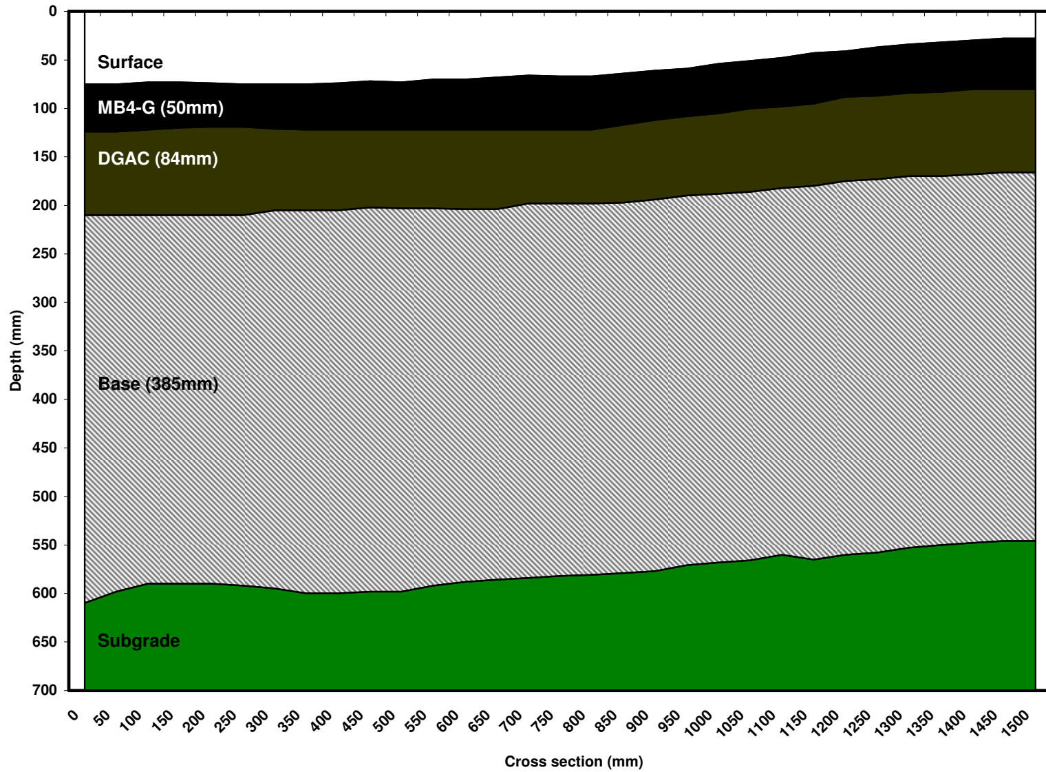
589RF #4 (45mm MB4-G) Cross Sectional Profile (2,086,004 reps)
