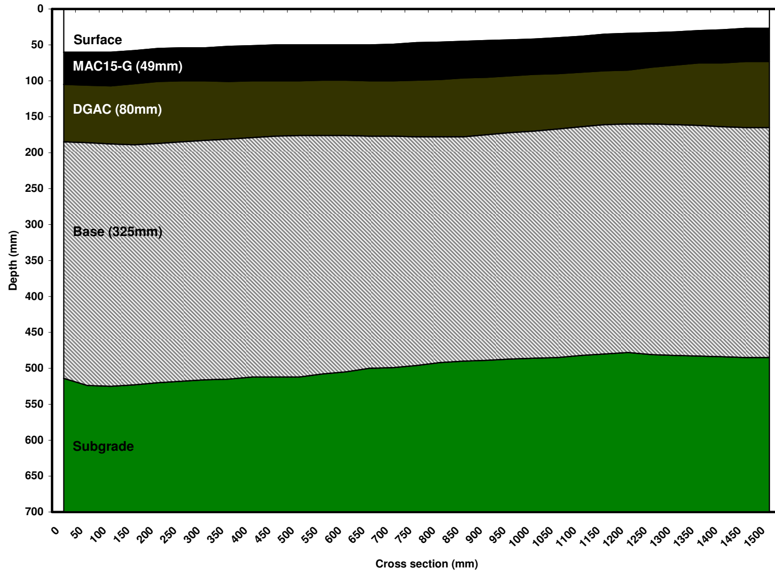
591RF #12 (45mm MAC15-G) Cross Sectional Profile (2,554,335 reps)
