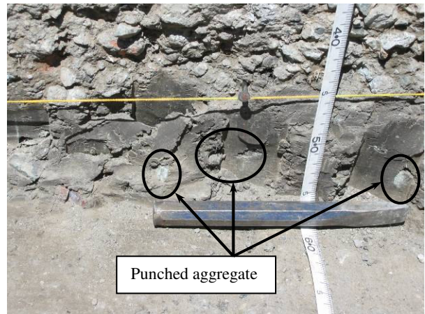
Figure 3.69: 591RF aggregate punched into subgrade.
