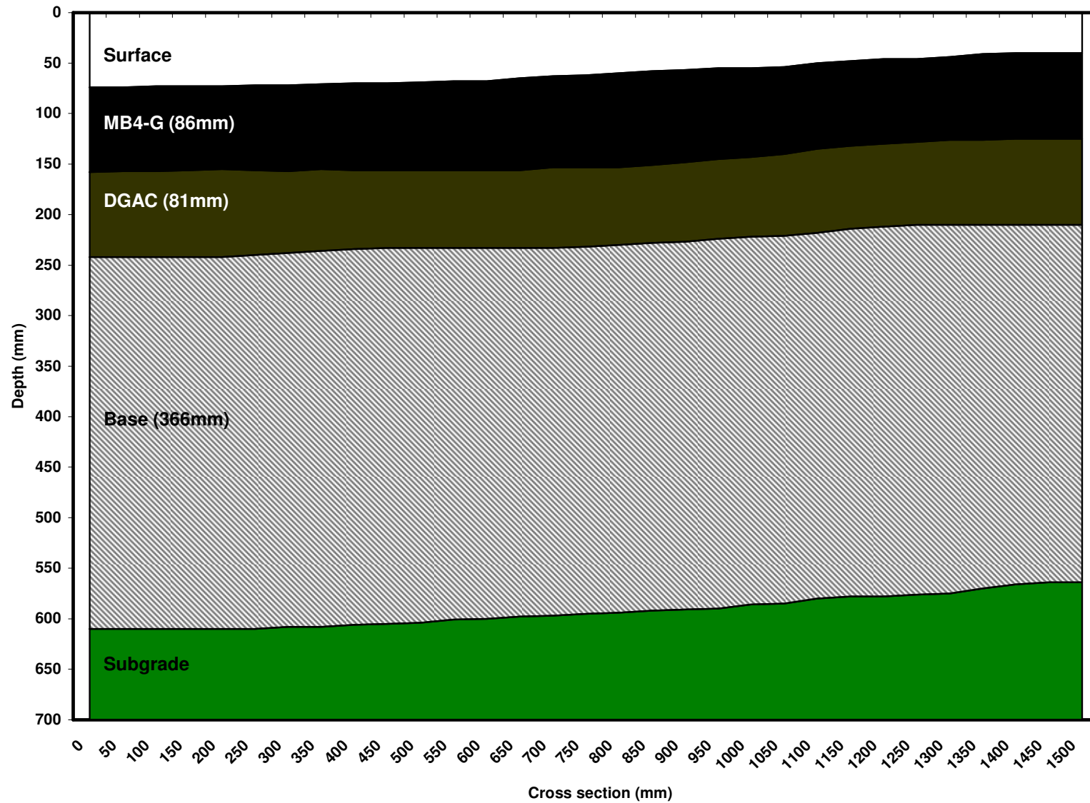
590RF #4 (90mm MB4-G) Cross Sectional Profile (1,981,365 reps)
