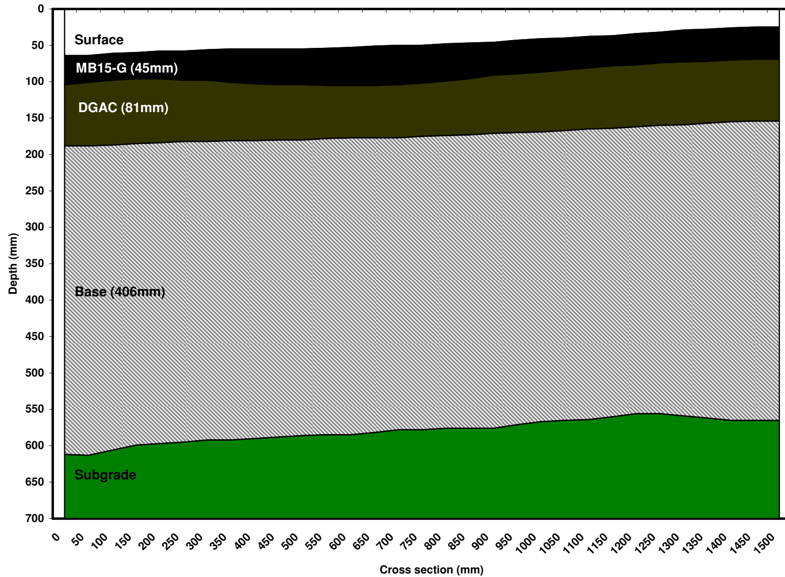
586RF #12 (45mm MB15-G) Cross Sectional Profile (2,492,387 reps)
