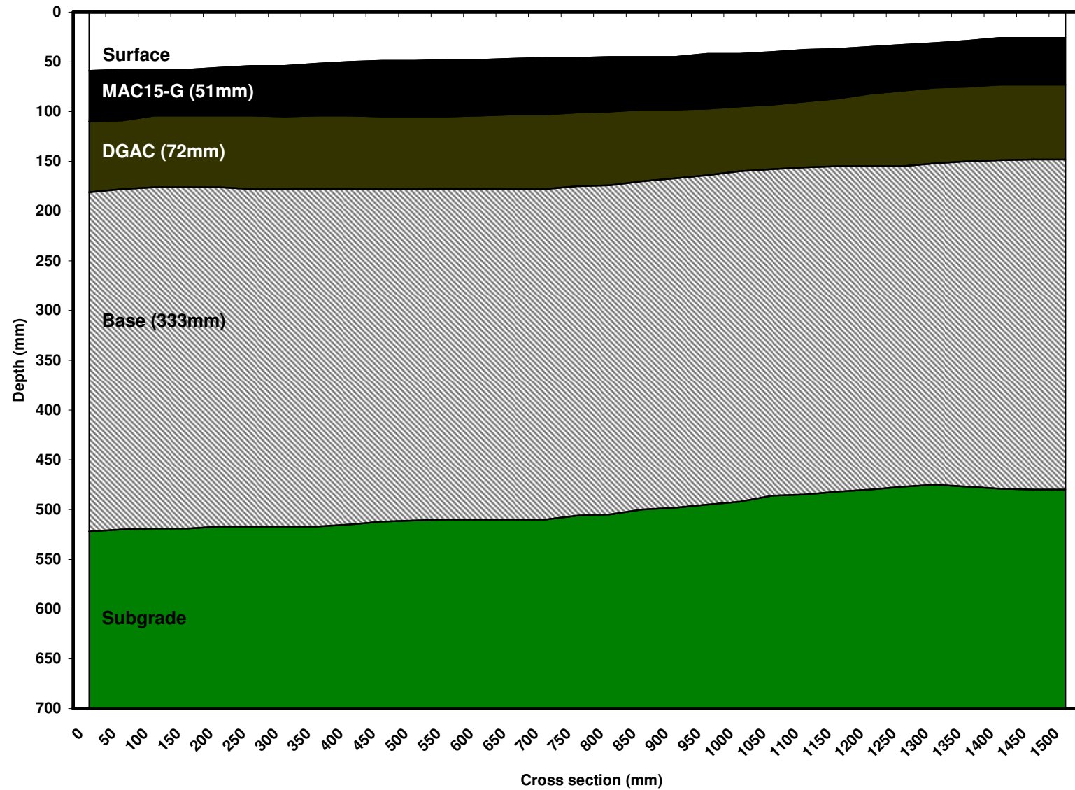
591RF #4 (45mm MAC15-G) Cross Sectional Profile (2,554,335 reps)
