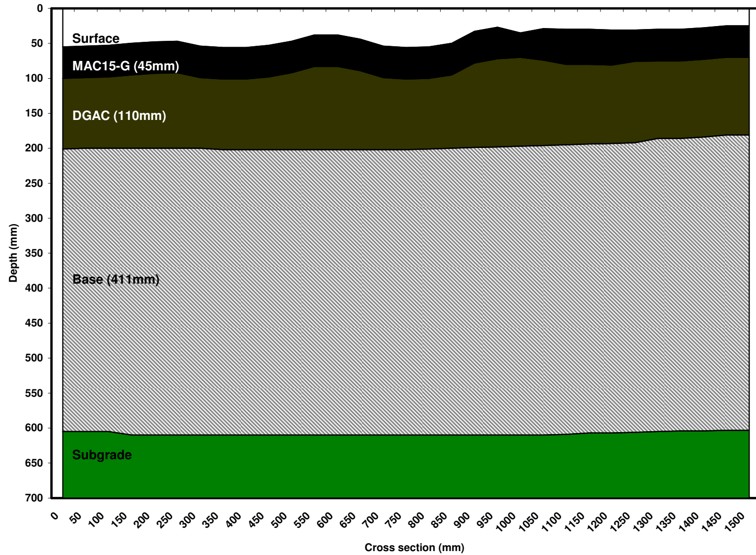
585RF (45mm MAC15-G) Cross Sectional Profile (3,000 reps)
