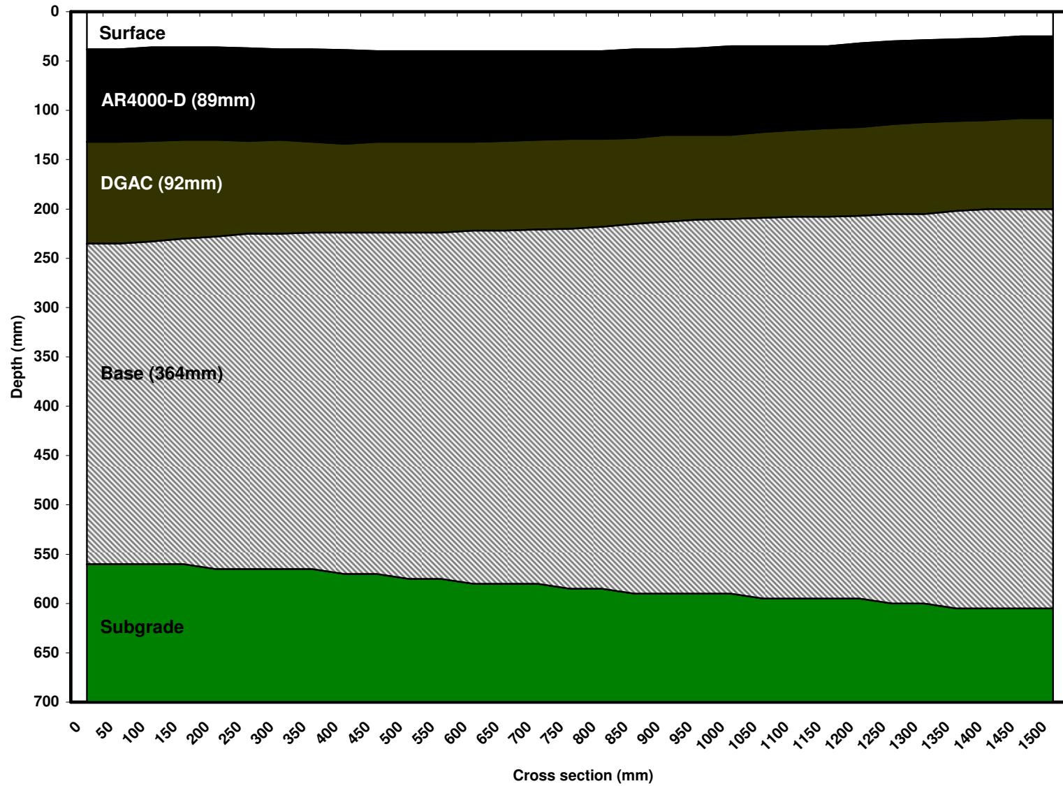
588RF #4 (90mm AR4000-D) Cross Sectional Profile (1,410,000 reps)
