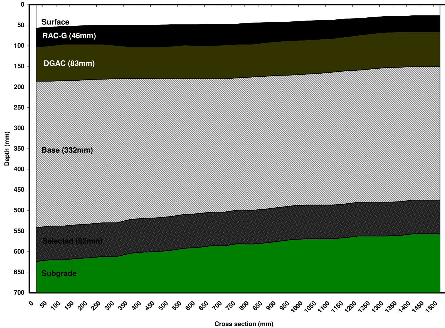
587RF #12 (45mm RAC-G) Cross Sectional Profile (2,024,793 reps)
