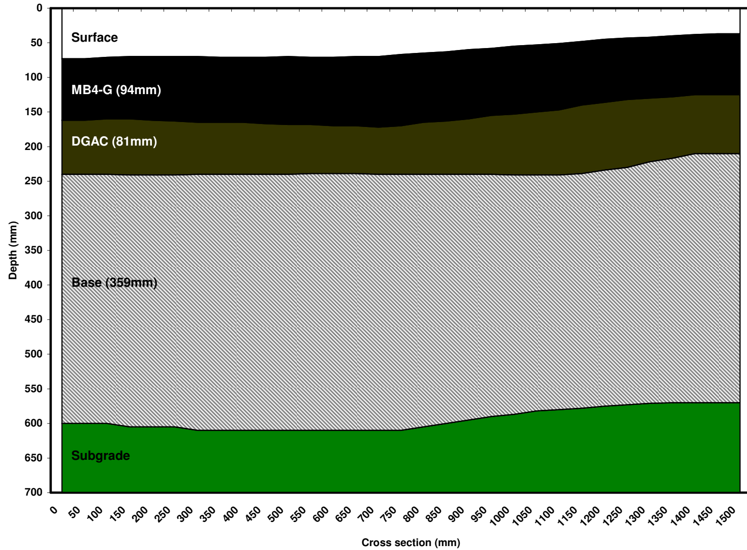
590RF #12 (90mm MB4-G) Cross Sectional Profile (1,981,365 reps)
