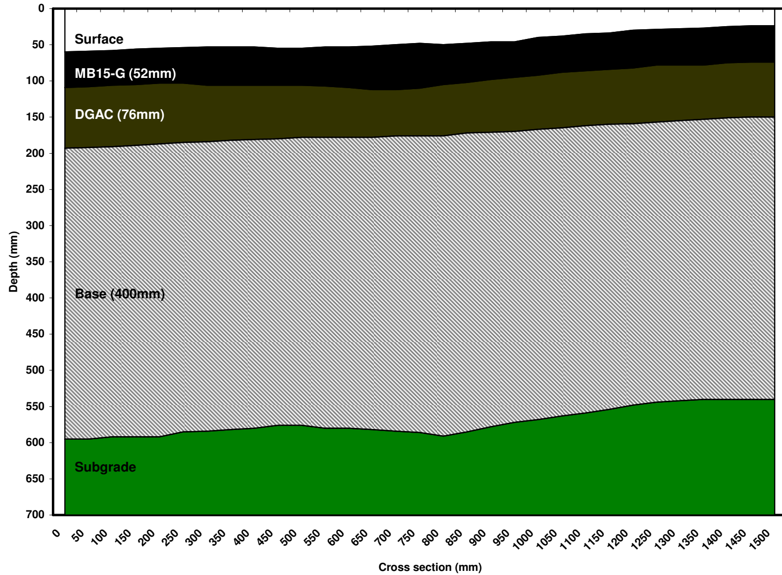
586RF #4 (45mm MB15-G) Cross Sectional Profile (2,492,387 reps)
