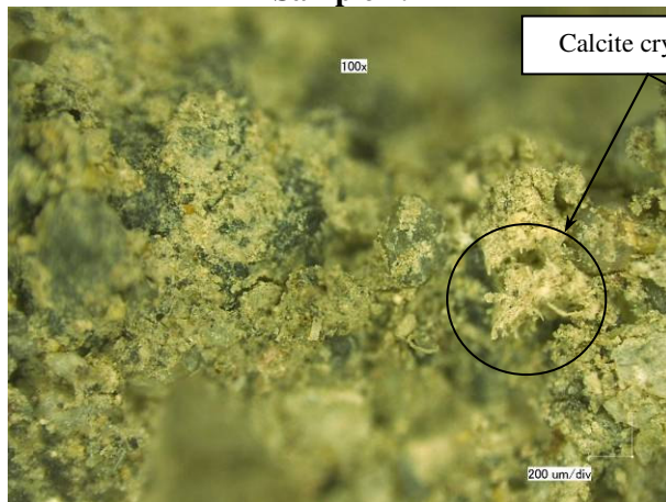
Figure 3.82: Optical microscope view ( \pm 100\times ) of calcite crystal development associated with cracks.
