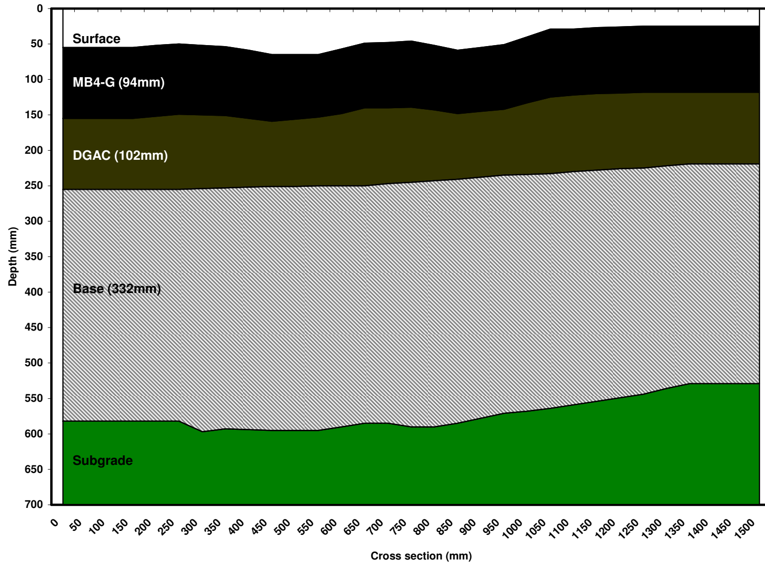
584RF (90mm MB4-G) Cross Sectional Profile (34,800 reps)
