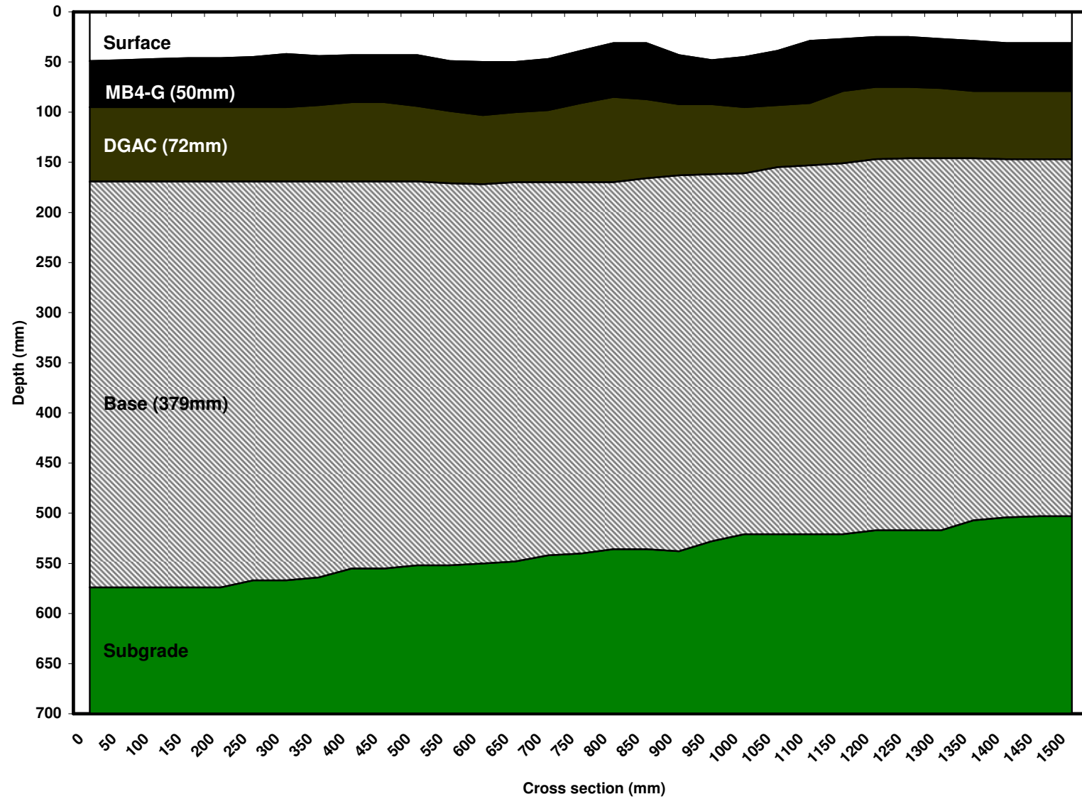
583RF #12 (45mm MB4-G) Cross Sectional Profile (15,000 reps)
