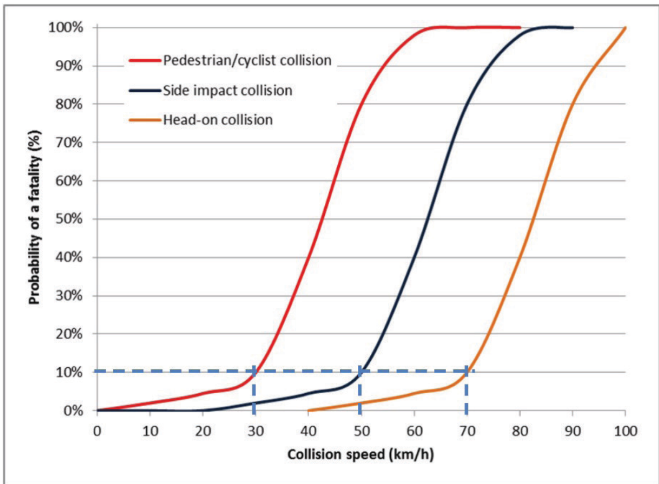
Figure 2.3. Fatal Probability vs. vehicle collision speed (Wramborg, 2015)
