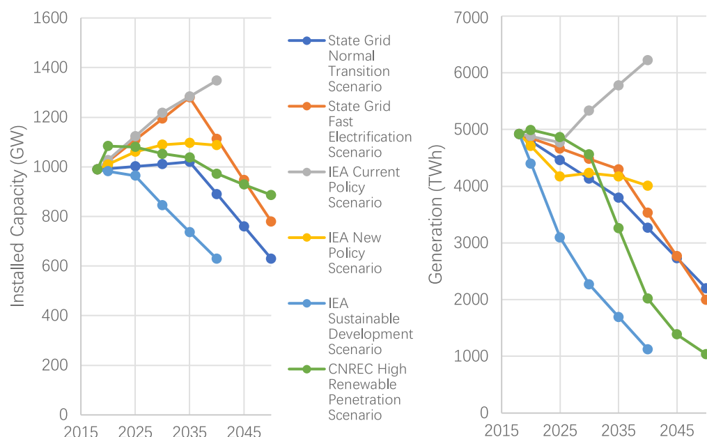
Figure 1. Installed coal capacity and annual generation in studies of china's long-term electricity needs
