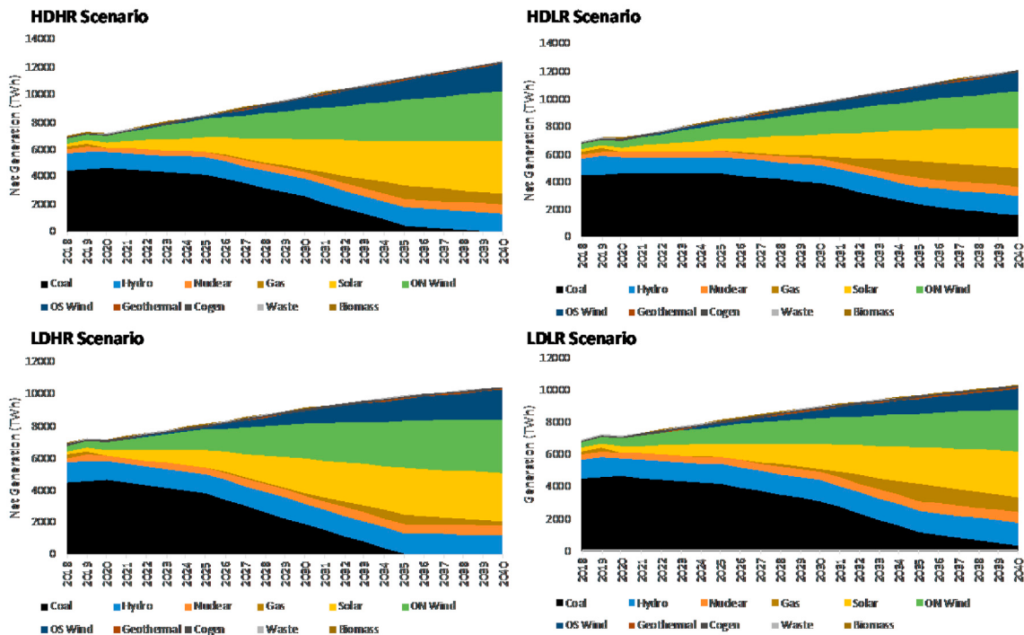
Figure 2. Installed capacity mix and annual generation mix in the four scenarios
