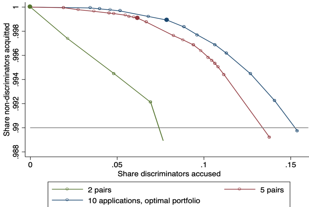
Figure VI: Detection/error tradeoffs, Nunley et al. data
