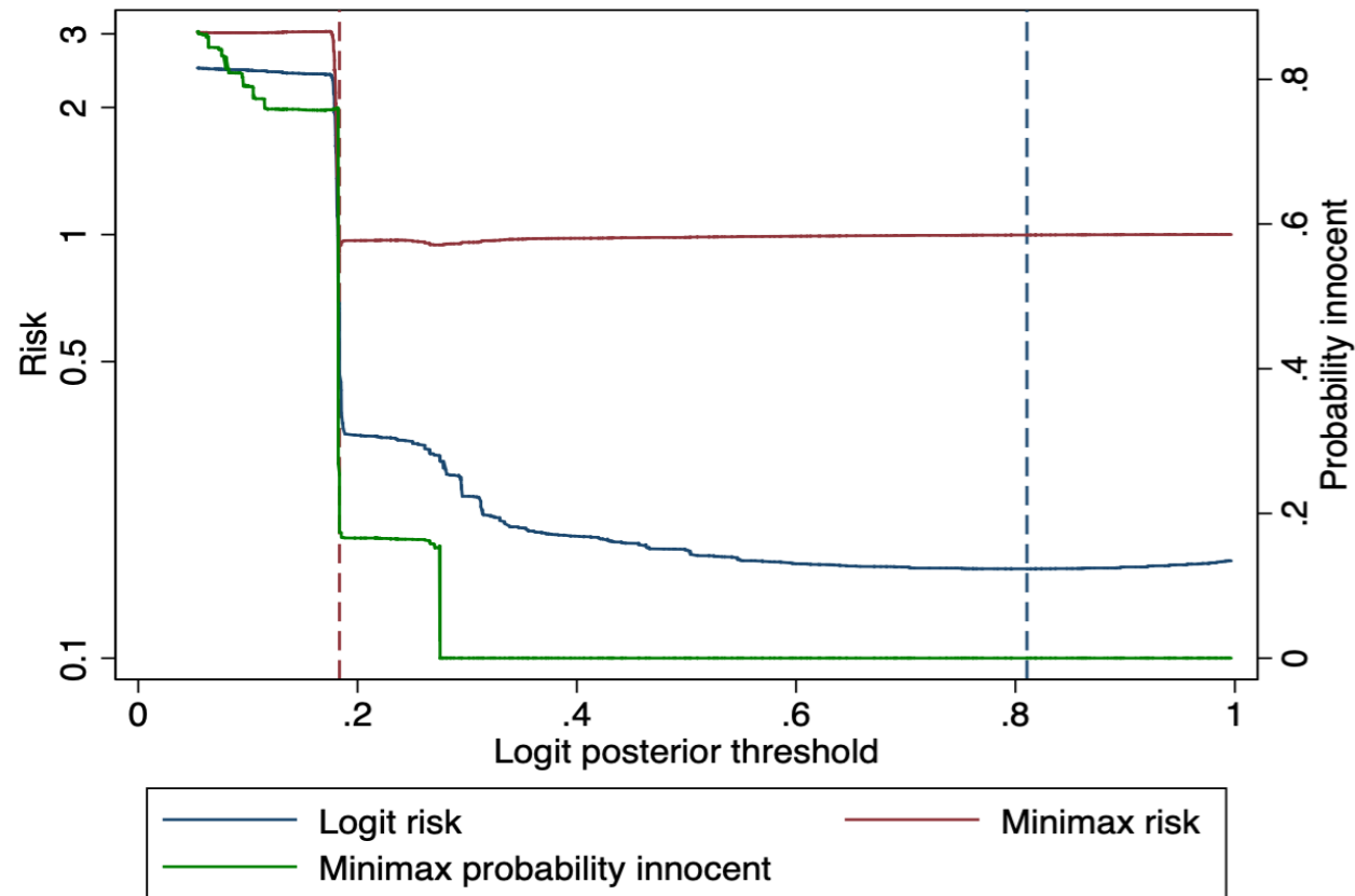
Figure VII: Logit and minimax risk, Nunley et al. data
