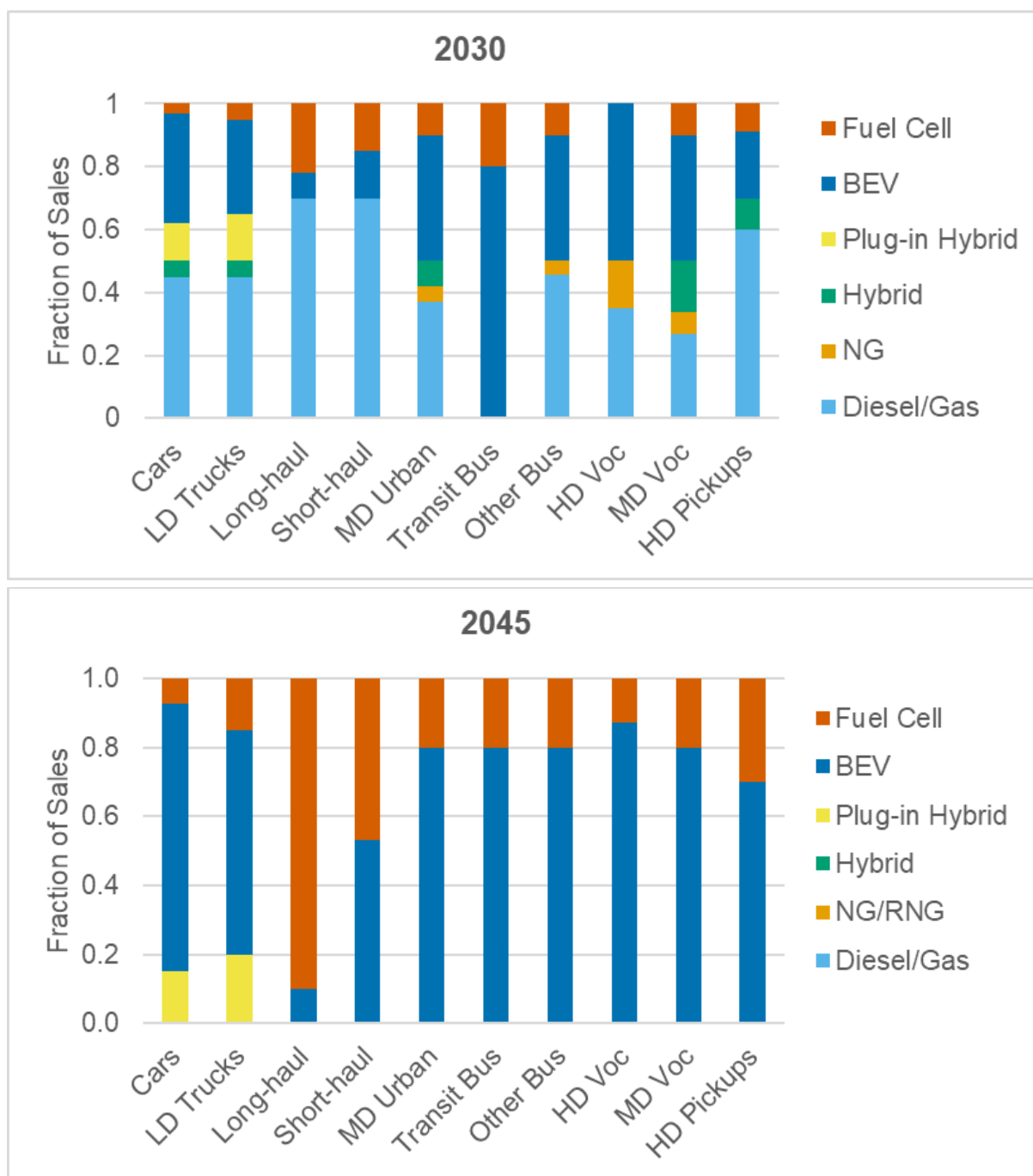
Figure 4.9. Sales shares of LDVs in the LC1 scenario for 2030 and 2045 show a wide variation in shares across vehicle class. by 2045, FCEVs dominate in long-haul and account for half of short haul trucks, while BEVs account for more than 50% sales in all other vehicle classes. (LD, light-duty; MD, medium-duty; HD, heavy-duty; Voc, vocational; BEV, battery electric vehicle; NG, natural gas; RNG, renewable natural gas)
