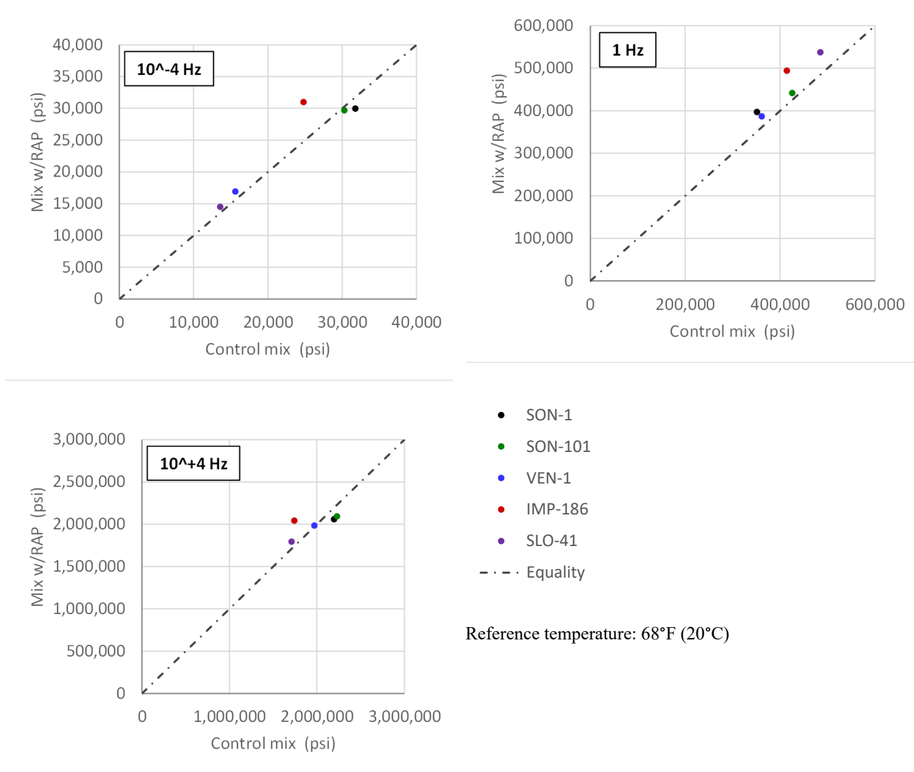
Figure 6.2: RAP effect on stiffness (AMPT axial dynamic modulus).
