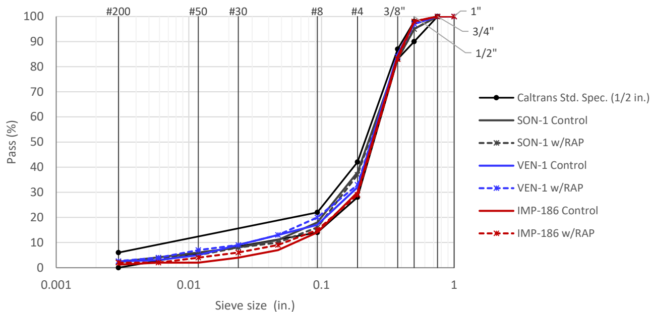
Figure 2.18: Gradation of RHMA-G mixes with 1/2 in. NMAS.
