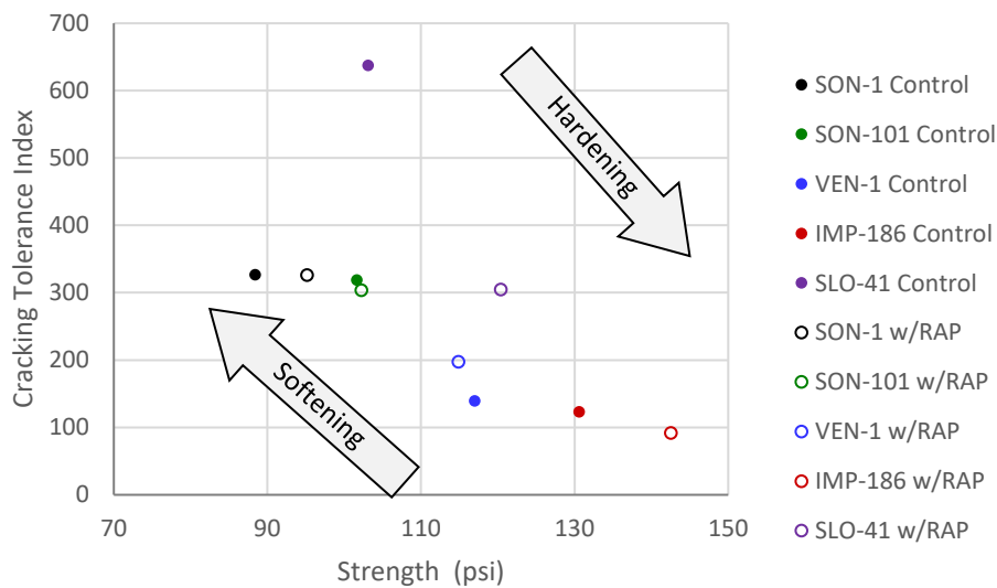
Figure 3.9: IDEAL-CT, CT_{Index} and Strength.
