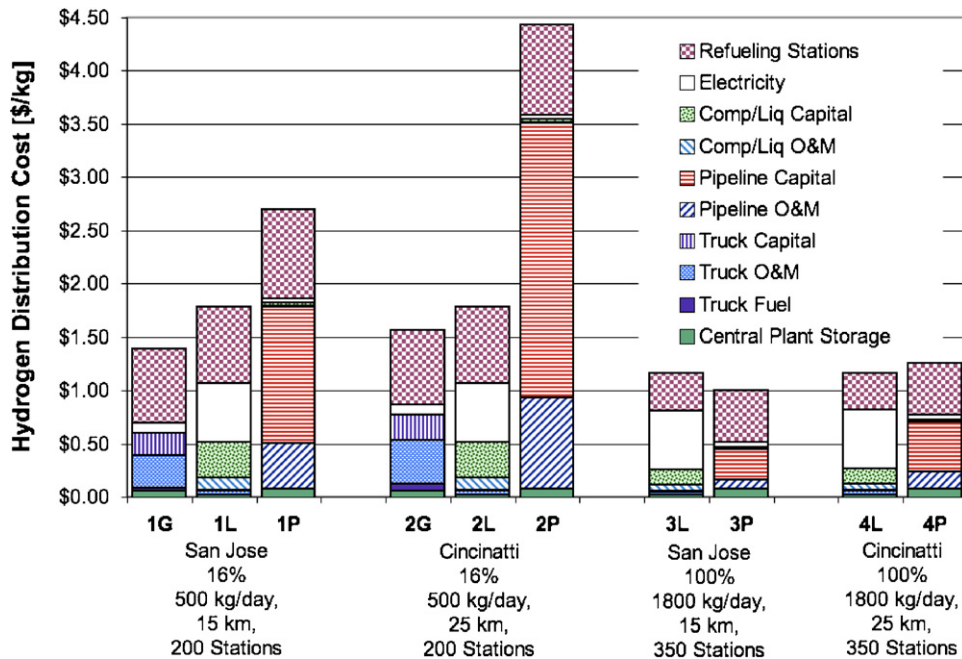
Fig. 10. Hydrogen distribution cost breakdown ($/kg) for the three delivery modes to a network of refueling stations in San Jose and Cincinnati (population 1.5 million): (1 and 2) 500 kg/day station size and 16% market penetration, (3 and 4) 1800 kg/day and 100% market penetration.
