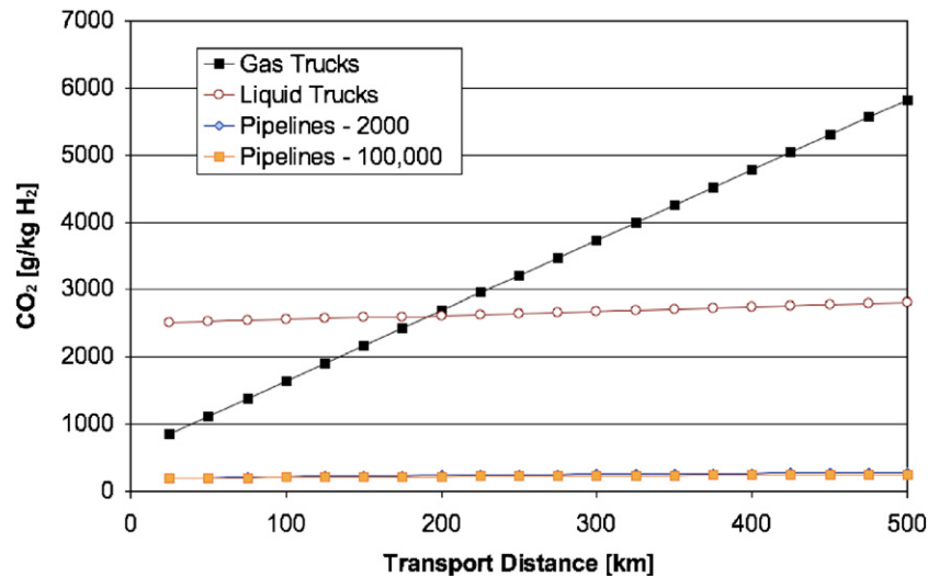
Fig. 9. CO 2 emissions (from electricity and diesel fuel) as a function of transport distance for the three different delivery modes. The CO 2 emissions associated with each of the modes are relatively constant with the flow rate of hydrogen. Electricity emissions are calculated for a California grid mix (low carbon).
