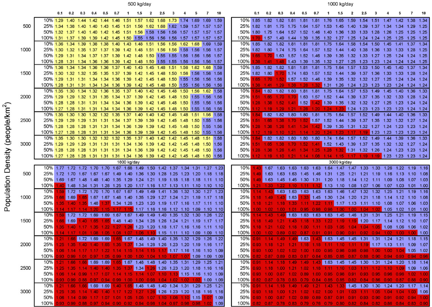
Fig. 14. Optimal distribution mode and cost ($/kg) maps for cities with different populations (0.1 to 10 million), population densities (500–3000 people/km 2 ) and station sizes (500–3000 kg/day) as a function of market penetration (10%, 25%, 50% and 100% penetration of H 2 fuel cell vehicles).
