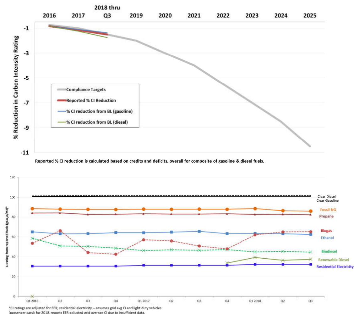
Figure 4. Annual average% CI rating reduction of reported fuels and compliance targets of gasoline and diesel fuel pools, CFP (top). Quarterly CI rating by fuel category, CFP (bottom). For both, reported data for 2016 and in 2018 through Q3. Reported ratings are adjusted for Energy Economy Ratio (EER), vi using the program value of 0.9 for natural gas in spark-ignition engines and 3.4 for residential electricity, which assumes all light-duty vehicles, or passenger cars). Reported CI ratings for all on-road electricity vehicles, and for off-road electricity use once covered by the program starting in 2018, were not calculated due to insufficient data and a data reporting error. vii Data source: [10].
