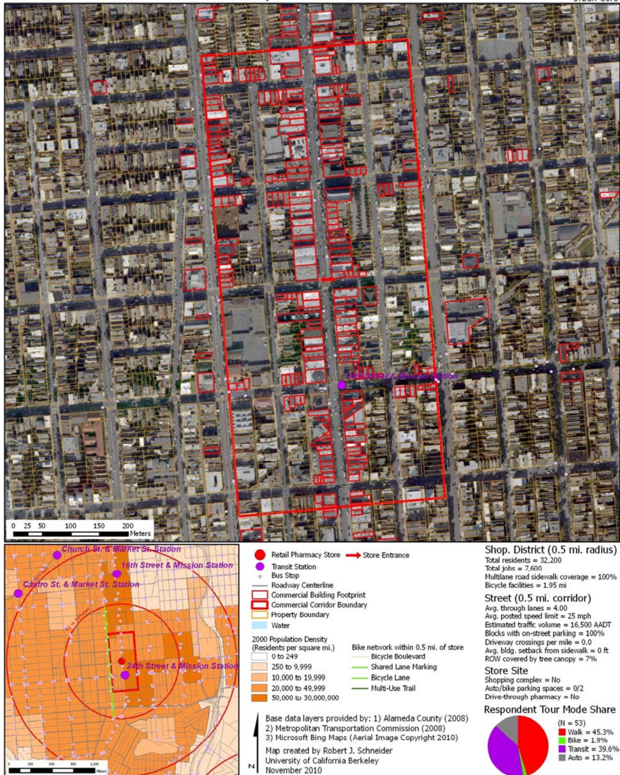
Figure 3.3., Part 1. Detailed Shopping District Characteristics: Urban Core Store Area: 2690 Mission Street, San Francisco
