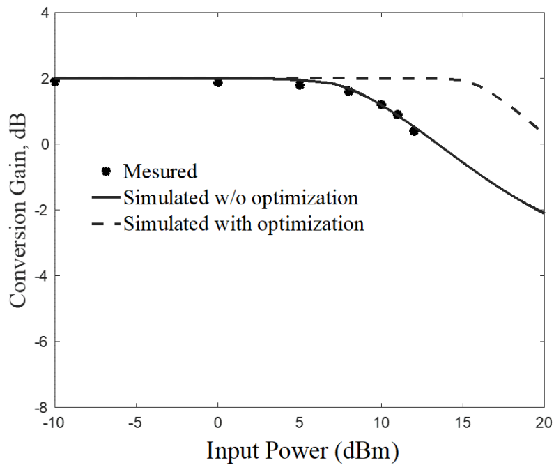
Figure 3.10: Measured conversion gain of the DP-TVTL versus the input power versus the simulated and optimized results.
