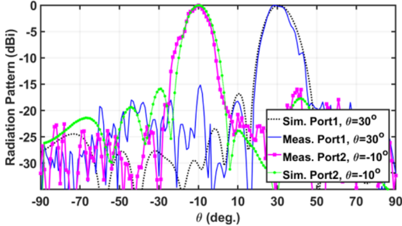
Figure 4.20: The simulated and measured normalized scanning radiation patterns in the elevation plane, when Right beam is directing at \theta = +30^\circ and Left beam is directing at \theta = -10^\circ .
