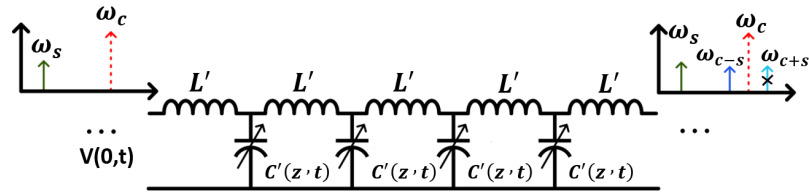
Figure 3.3: Simplified Lumped-element model of the Figure 3.2 with time-varying capacitance.
