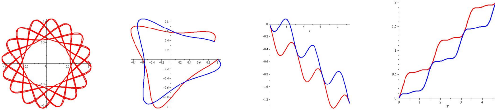
Figure 4.1: The first panel displays a typical r -periodic solution of an-harmonic oscillator. The last three panels show the Maxwell point in the plane (x_1, x_2) , (t, y) and (t, z) , respectively.
