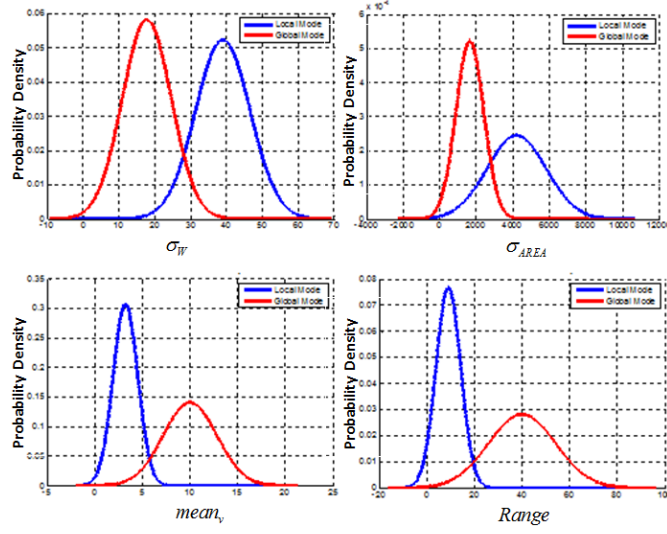
Figure 2.8: Estimated conditional probability distributions of the four motion attributes given the activity mode
