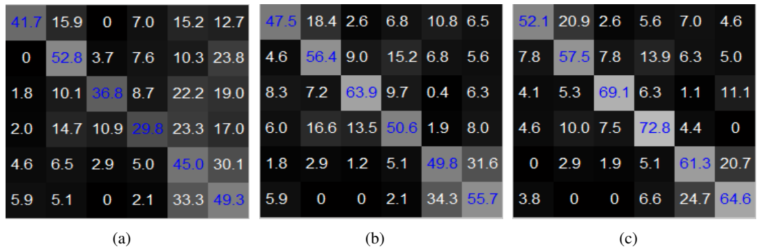
Figure 3.12: Recognition Results for VIRAT Release 1. (a): Confusion matrix for the baseline classifier; (b): Confusion matrix for our approach using motion and intra-activity context features; (c): (b): Confusion matrix for our approach using motion and intra- and inter- activity context features.
