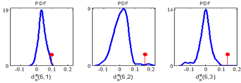
Figure 5.2: Example of probability density functions of d_x^a(y_{a_t}^{opt}, j) , j = 1, 2 and 3 for normal activities and the corresponding distances of a point anomaly (indicated by red circle). The first ten activities in Section 3.6.1.2 are considered as normal activities, and used to train the structural model. For the point anomaly detected y_{a_t}^{opt} = 6 .
