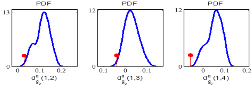
Figure 5.3: Example of probability density functions of d_{g_k}^a(y_{a_t}^{opt}, j) , k = 2 , j = 2, 3 and 4 , for normal activities and the corresponding distances of a contextual anomaly (indicated by red circle). The first ten activities in Section 3.6.1.2 are considered as normal activities and used to train the structural model. For the contextual anomaly detected y_{a_t}^{opt} = 1 . Intra-activity context subset G_2 is defined in Sec. 3.4.1.
