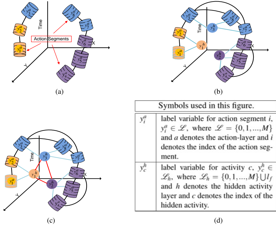
Figure 3.6: Illustration of CRF models for activity recognition. (a): Action-based Linear-Chain CRF; (b): Action-based higher-order CRF model (with latent activity variables); (c): Action-based two-layer HCRF. Note that all the observations for the random variables are omitted for compactness. One action segment denotes a random variable in the action layer, whose value is the activity label for the action segment. A colored circle denotes a random variable in the activity layer, whose value is the label for its connected clique. As shown in (a), in the action layer, action segments that belong to the same trajectory are modeled as a linear-chain CRF. Then, hidden activity-level variables with action-activity edges (in light blue) are added for each action cliques to form higher-order CRF as shown in (b). An activity nodes and its associated action nodes have a same color. Finally, pair-wise activity edges (in red) are added to form the proposed two-layer HCRF model.
