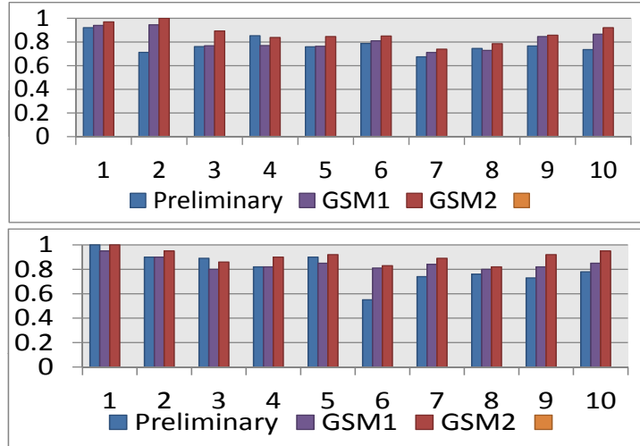
Figure 4.4: Precision (top) and recall (bottom) for the ten activities in UCLA Office Dataset.
