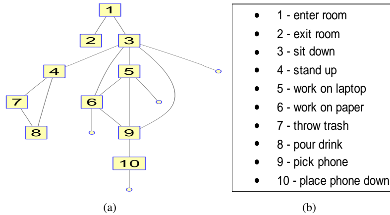
Figure 4.5: (a): The learned graphical structure using the proposed GSM. (b): Indexes vs activity classes
