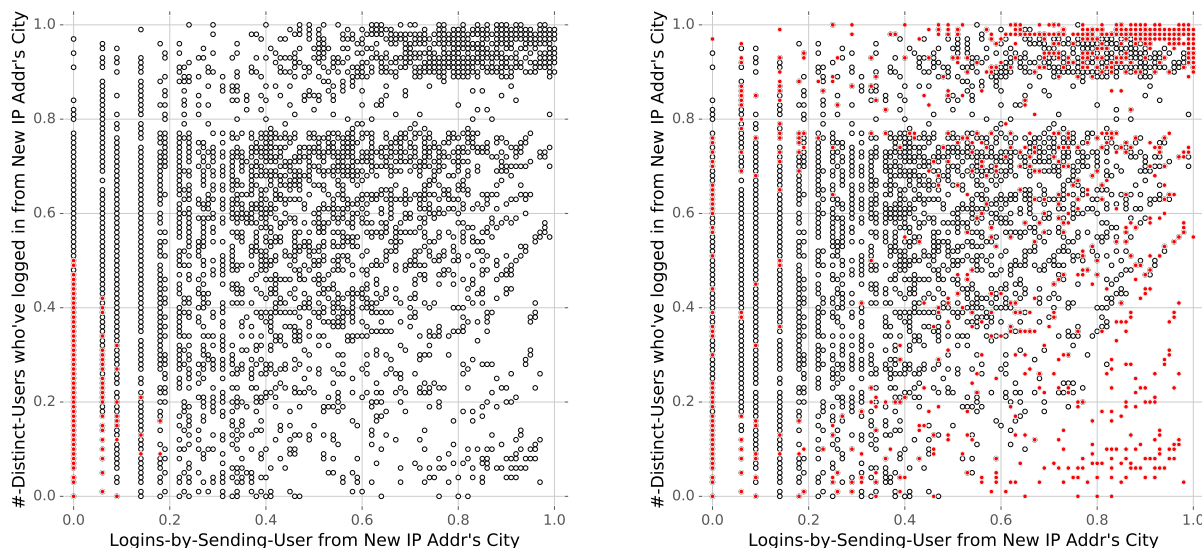
Figure 3.7: Both plots show the sender reputation feature values (scaled between [0, 1]) of a random sample of 10,000 lateral attacker click-in-email events. Filled red points denote events that generated alerts within the daily budget by DAS (left-hand figure) and KDE (right-hand figure).
