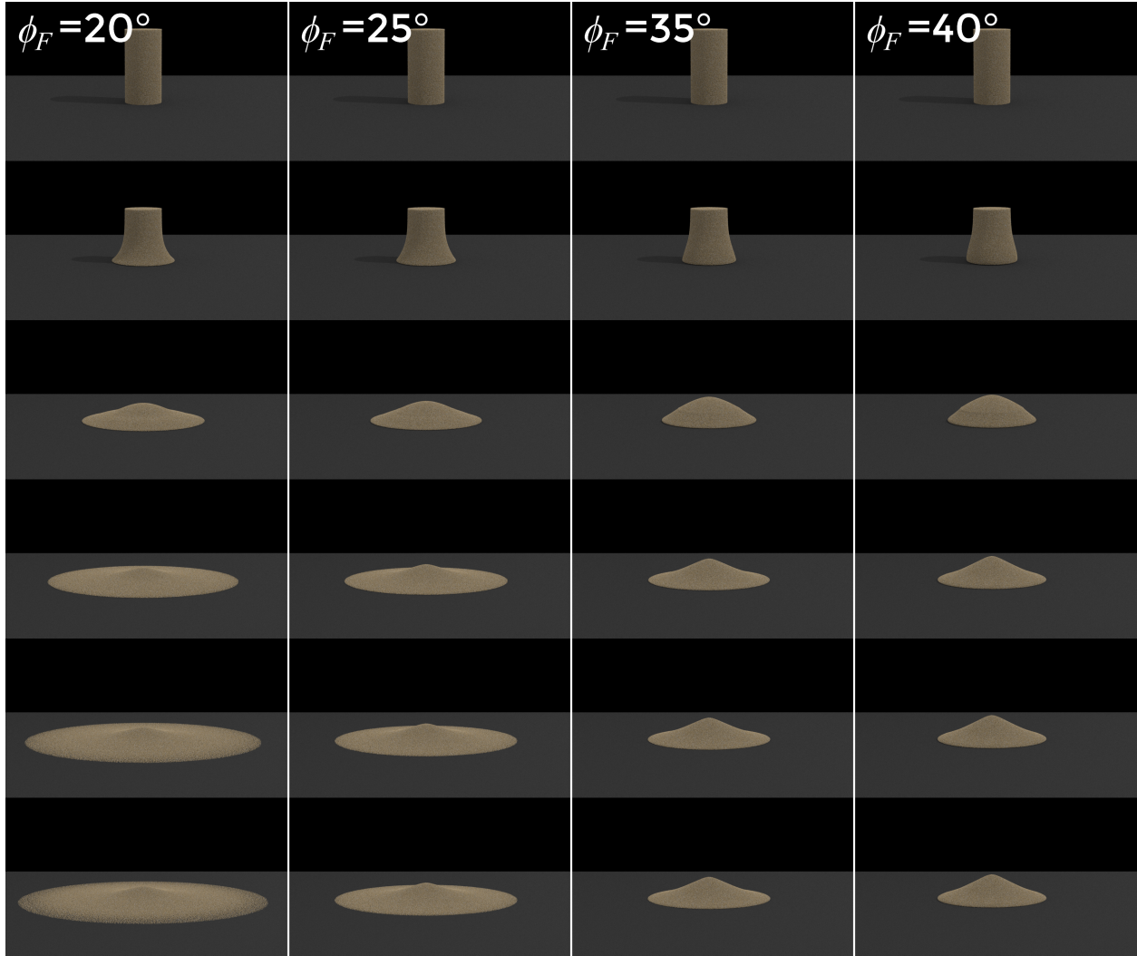
Figure 4.1: Effect of friction angle on piling.
