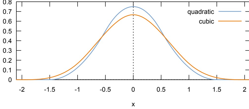
Figure 3.1: Interpolation kernels
