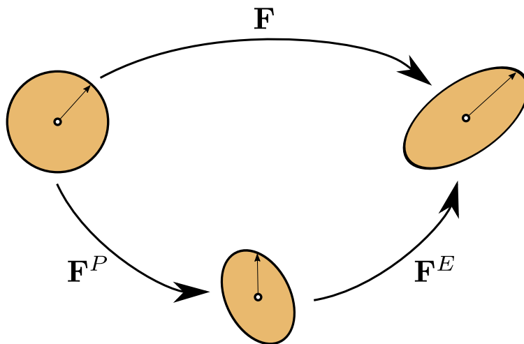
Figure 2.2: Multiplicative decomposition of a neighborhood
