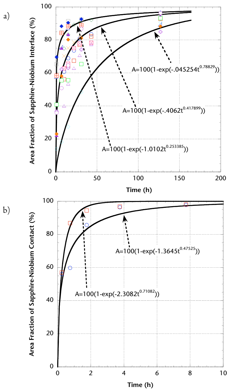
FIGURE 6 Assessment of the “dewetting” kinetics for the copper film in LFAJ. a) At 1150°C, the area fraction of sapphire-niobium contact increases rapidly and typically exceeds 80% after 10-20 hours. b) At 1400°C, the area fraction of sapphire-niobium contact exceeds 90% after just a few hours.
