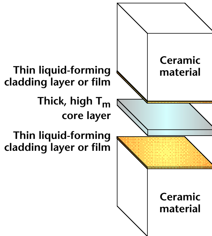
FIGURE 1 Schematic illustration of an assembly with a multilayer interlayer. Two relatively thin cladding layers that form a liquid at low temperature flank a thicker and higher melting point core layer that dominates the composition and ultimate physical properties of the interlayer.
