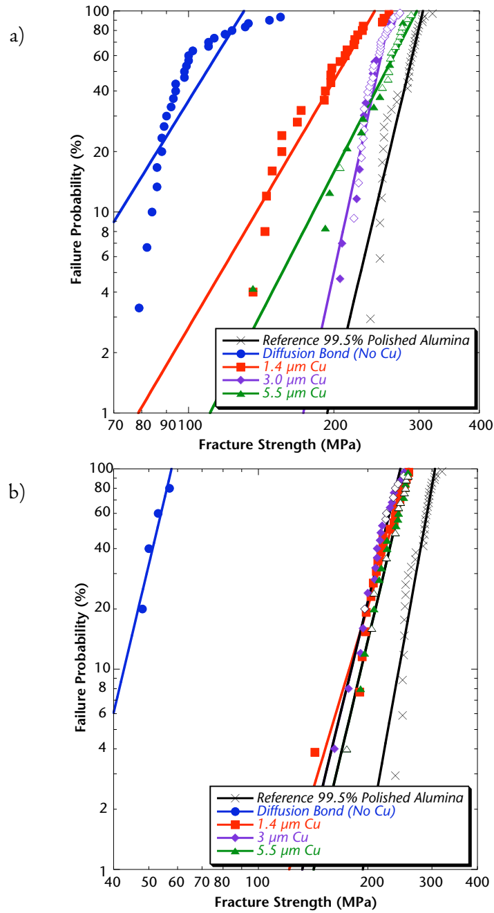
FIGURE 7 Plots of fracture probability versus fracture strength for alumina joined using Cu/Nb/Cu interlayers. Results are for bonding cycles of 6 h at 1400°C using a) polished substrates, and b) as-ground (400 grit) substrates. It is evident that the liquid copper film is beneficial, especially for ground substrates.
