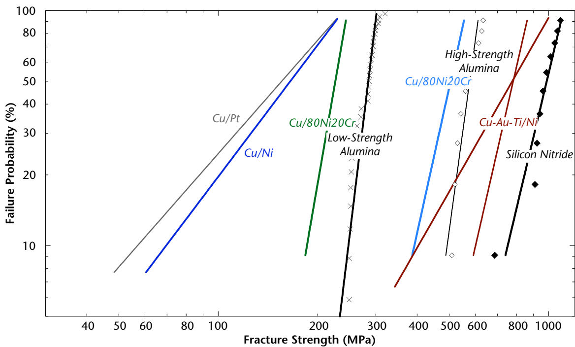
FIGURE 4 Room-temperature strength distributions for different interlayer designs used to join alumina and silicon nitride. Cu/Pt, Cu/Ni, and Cu/80Ni20Cr interlayers were used to bond alumina. Note the beneficial effect of Cr additions. The Cu-Au-Ti/Ni interlayer was used to bond silicon nitride; the two lines correspond to different joining temperatures.
