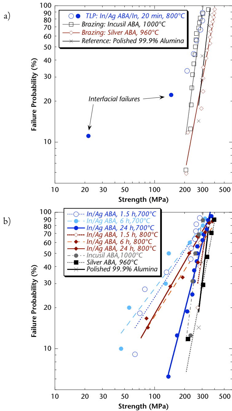
FIGURE 5 Plots of fracture probability versus fracture strength for alumina joined using In/Silver ABA/In interlayers. a) 20 min bonding cycle at 800°C, and comparison to conventional reactive-metal brazing. b) Effect of bonding time and temperature on strength and failure characteristics of TLP bonds.
