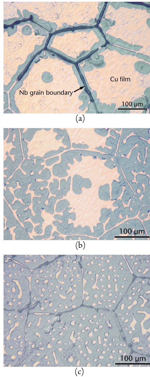
FIGURE 3 Optical micrographs taken of a sapphire/copper/niobium interface showing a) initial, b) intermediate, and c) final stages of sapphire-niobium contact growth. Note that in the final stage, sapphire-niobium contact dominates the interface microstructure ( \approx 90\% area fraction), and therefore the thermomechanical characteristics of the interface.
