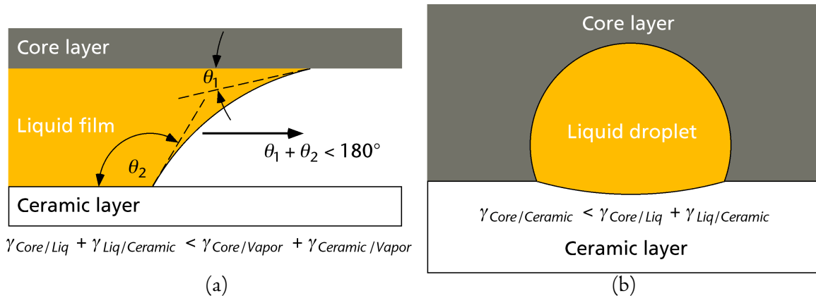
FIGURE 2 a) Schematic illustration of a thin liquid film sandwiched between a solid metallic core layer and a ceramic on which the liquid has contact angles \theta_1 and \theta_2 , respectively. For parallel core layer and ceramic surfaces, void filling requires that \theta_1 + \theta_2 < 180^\circ . b) In LFAJ, at later stages, liquid-film-assisted growth of ceramic-core contact produces a “dewetting” of the ceramic–core layer interface and results in isolated droplets of liquid.
