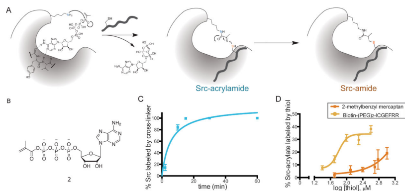
Figure 2. Reactions of crosslinker 2 with c-Src. (A) Reaction scheme of crosslinker 2 with c-Src. (B) Structure of crosslinker 2 . (C) Time course of acrylamide formation with 20 \mu\text{M} crosslinker added to 4 \mu\text{M} c-Src and quantified by LC-MS. Error bars represent the SEM of duplicate data points. Data is representative of three separate experiments. (D) Dose response curve of thiol reaction with Src-acrylamide. Indicated thiol was added to 4 \mu\text{M} c-Src-acrylamide and allowed to react for 25 minutes at room temperature. Results were analyzed as in (C).
