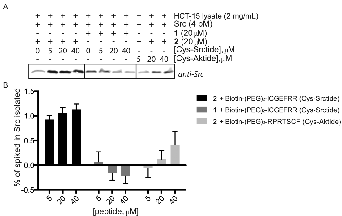
Figure 4. Streptavidin-agarose precipitation of recombinant c-Src added to HCT-15 cell lysate. (A) Representative western blot. 4 pmol recombinant c-Src was added to 500 \mu L of 2 mg/mL HCT-15 cell lysate followed by 20 \mu M crosslinker. After 10 minutes the indicated quasi-substrate was added and the reaction proceeded for 25 minutes. The proteins were captured using High Capacity Streptavidin beads. Bands were quantified using Odyssey Imaging System Imager. (B) Quantification of c-Src obtained from Streptavidin precipitation experiments as a percentage of total c-Src added to the HCT-15 cell lysate. Error bars represent the SEM of duplicate data points. Data are representative of two separate experiments.
