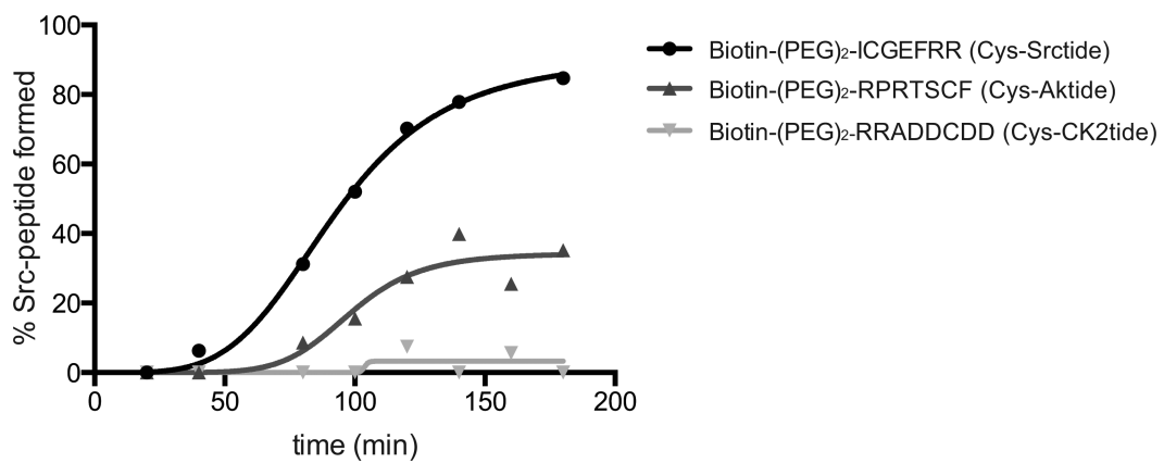
Figure 3. Product formation as a function of time. The indicated peptide (74 \mu M) was added to 4 \mu M c-Src with 20 \mu M crosslinker 2 . Percentage final product was calculated as a percentage of total c-Src present as quantified by LC-MS. Also see figure S4.
