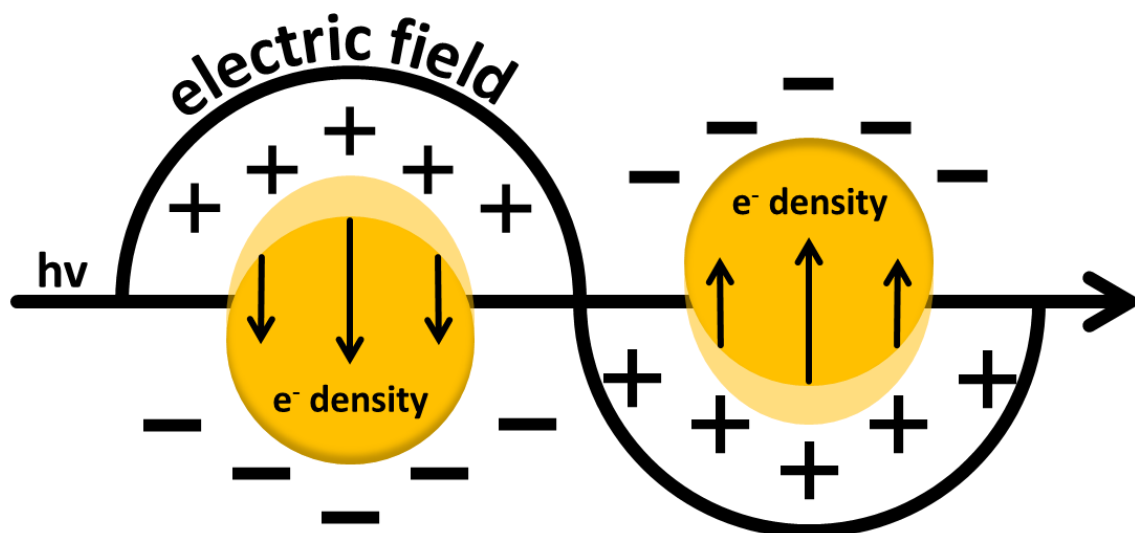
Figure 11: Localized surface plasmon resonance showing oscillations of electrons due to electromagnetic waves When these electric fields decay on the order of 1-100 femtoseconds, the energy dissipates through radiative emission, or through the more preferred path of hot electron generation. These energetic electrons are termed ‘hot’ because they exist at the top of a Fermi distribution of electron energies in conductive nanostructures. Most often observed in gold or silver nanoparticles and nanorods, these hot electrons may be injected into the conduction band of an appropriate semiconductor such as titania. An ideal semiconductor has an electron affinity below the Fermi level of the metal, forming a Schottky barrier that the hot electrons overcome. A small percentage of these hot electrons succeed in becoming charge carriers in the semiconductor conduction band as shown by the red arrow in Figure 12. This occurs at a reduced energy requirement compared to the standard bandgap of the semiconductor and absorbing light of lower energy than would otherwise be possible. An alternate, though much less likely, non-radiative path for the same hot electrons is to tunnel through the Schottky barrier into the semiconductor as seen by the dotted arrow in Figure 12. 13
