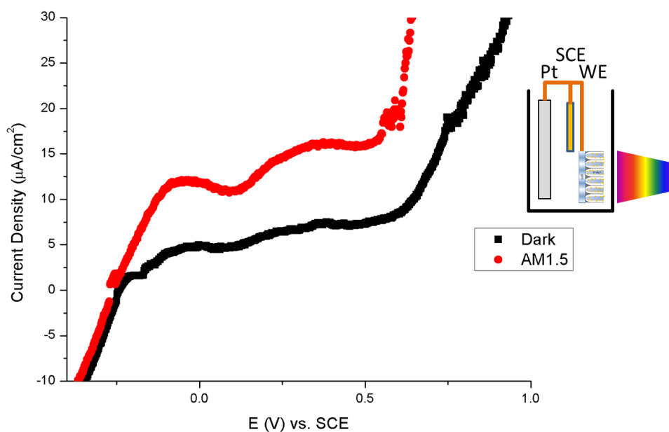
Figure 21: Linear sweep voltammogram of TNA-AuNP photoanode on FTO at 20mV/sec in 1M NaOH normalized for 1 sun AM1.5 solar radiation above 420nm.
