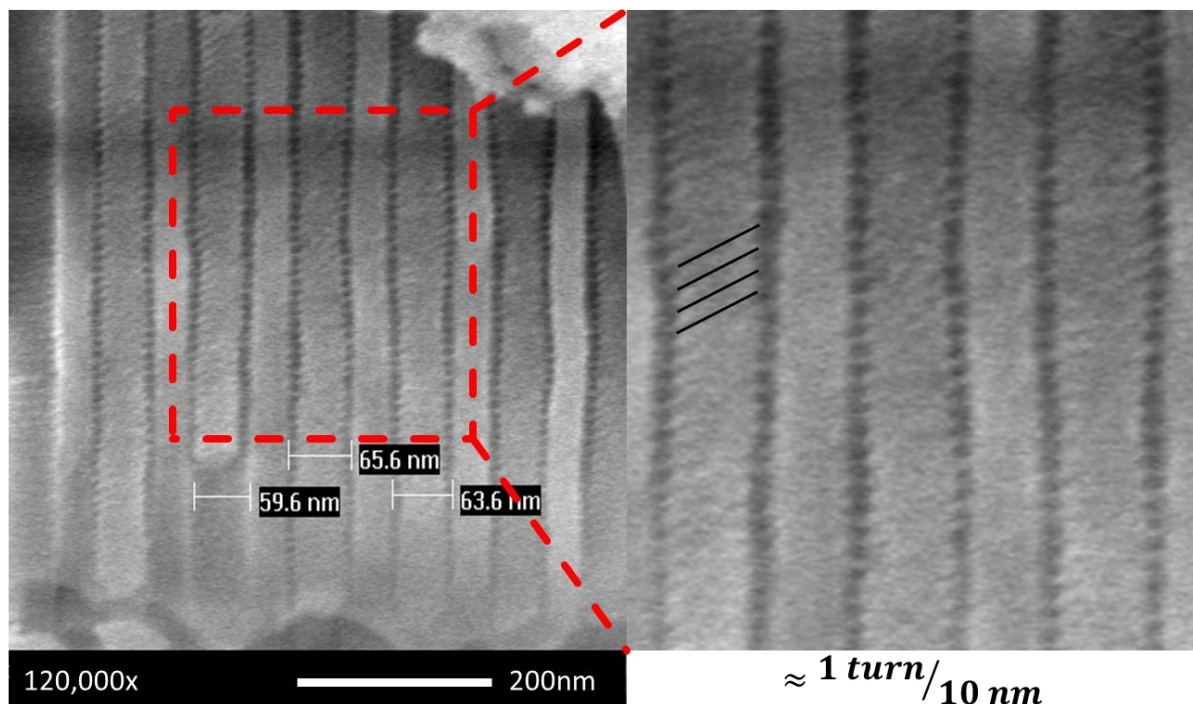
Figure 25: SEM images of double helical mesoporous silica template within AAO template. Enlargement shows angular nature of helical structures.
