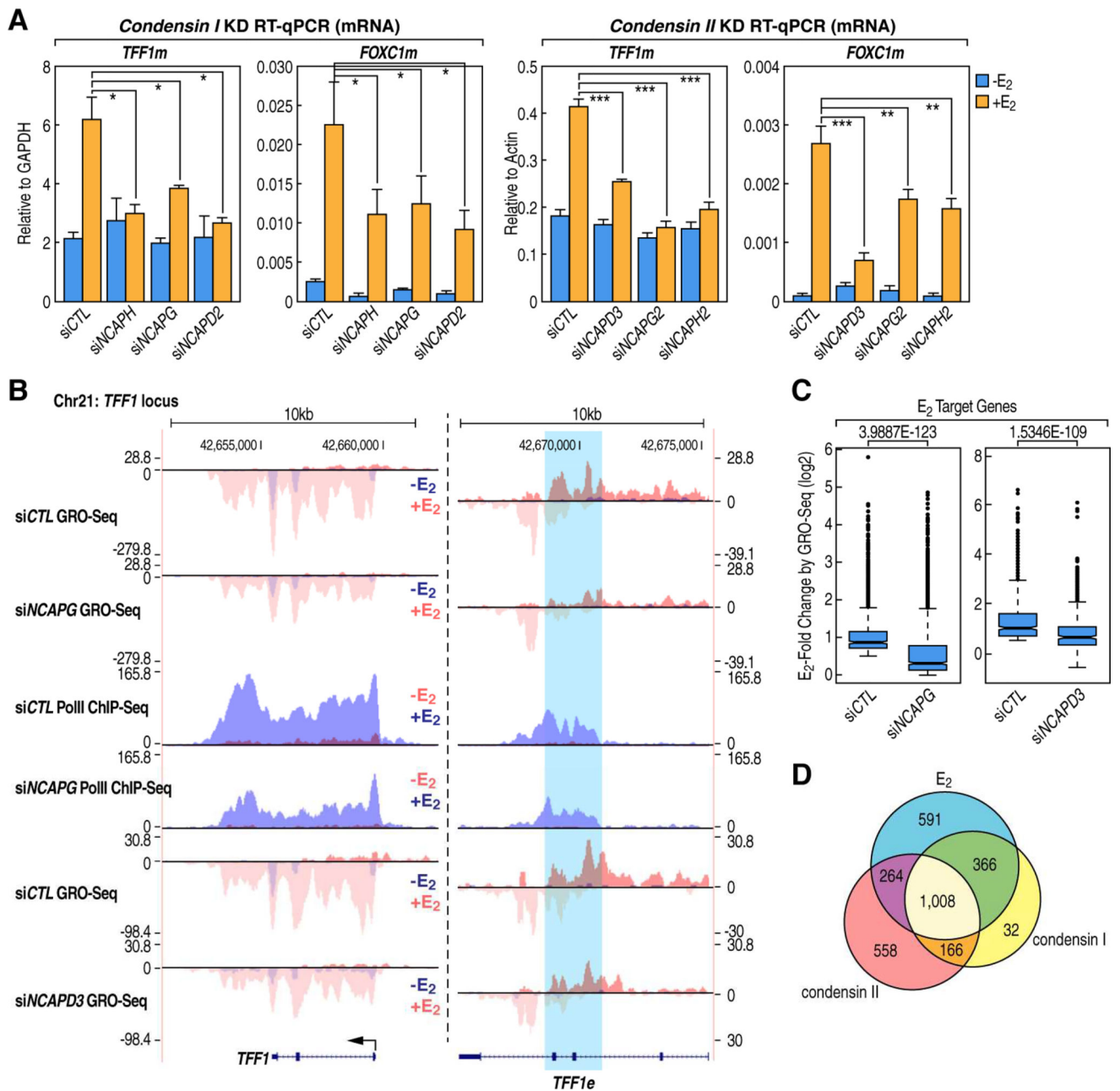
Figure 3. Condensin I and condensin II control ER- \alpha -regulated gene activation in a partially overlapping manner
