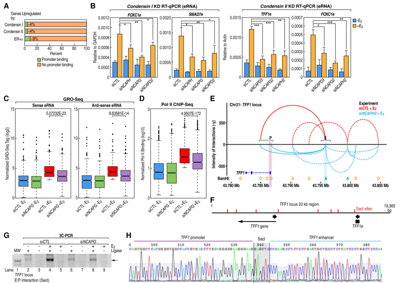
Figure 4. Condensins are needed for full eRNA activation and enhancer:promoter looping (A) Bar graphs showing the percentage (green colored) of the RefSeq genes up-regulated by condensin I, II or ER- \alpha that possesses direct promoter-binding of the respective factor. (B) RT-qPCR data indicating the levels of representative E 2 -induced eRNAs when either condensin I or condensin II subunit was knocked down ("e" after gene names denotes eRNA). (n=5). KD, knockdown. Data are represented as mean \pm s.d.. *p<0.05, **p<0.01, ***p<0.001, (Two-tailed students' T-test). (C) Boxplots of normalized GRO-Seq tags showing levels of E 2 -induced eRNAs on the active enhancers in siCTL or siNCAPG transfected cells, from both sense and antisense directions. (Two-tailed students' T-test). (D) Boxplot of normalized ChIP-Seq tags showing RNA Pol II recruitment to active enhancers in same group of cells as in panel C. (Twotailed students' T-test). (E) Results from 3D-DSL assay showing detected chromatin interactions in the displayed region of TFF1 locus in the presence of either siCTL or siNCAPH2 (blue) (plotted by GGbio, see methods). The normalized intensities of interaction counts are plotted on the y-axis, and the x-axis depicts coordinates from UCSC browser (Hg19). Interaction data are overlaid with positions of the Donor (D, yellow) and Acceptor (A, green) BamHI sites. The pertinent E:P interactions are shown in solid lines and other interactions are shown in dotted lines. The interactions are quantitatively coded by height. Highlighted areas denote E: enhancer, P: promoter. More details can be found in the Supplemental Experimental Procedures. (F,G) A 3C-PCR assay
