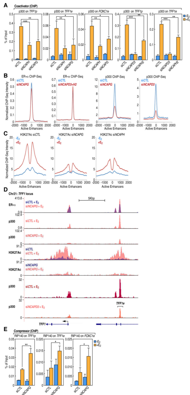
Figure 5. Condensins license appropriate coactivator (CoA) and corepressor (CoR) recruitment during enhancer activation
