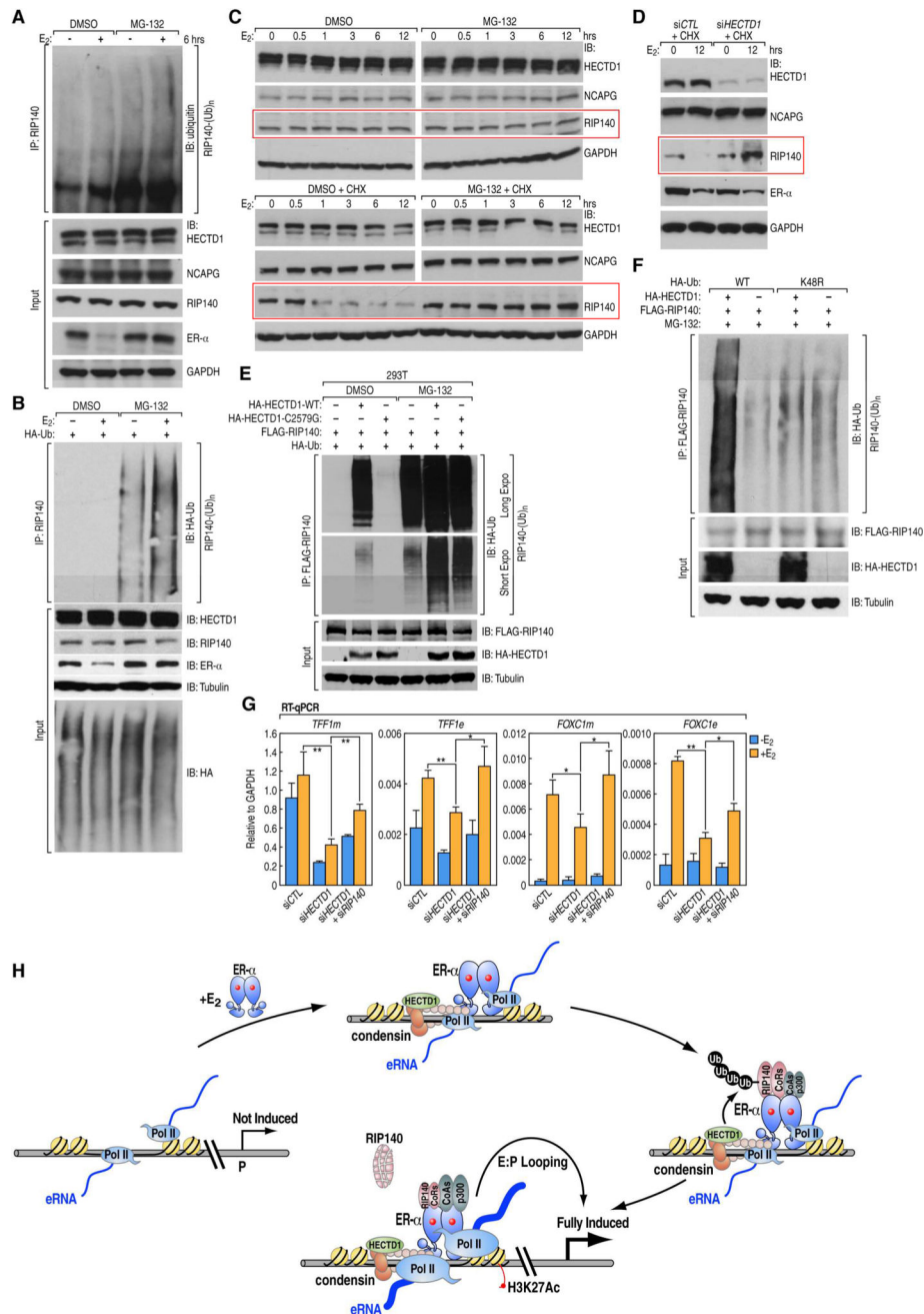
Figure 7. Evidence suggesting RIP140 as a polyubiquitination substrate of HECTD1 (A,B) Immunoblotting with indicated antibodies showing IP results using a native RIP140 antibody in wild type MCF-7 cells (A) or cells transfected with a HA-Ub plasmid (B) , revealing the poly-ubiquitination ((Ub) n ) of RIP140. (C) Western blots showing total protein levels of HECTD1, NCAPG and RIP140 in MCF-7 cells upon different lengths of E_2 treatment with or without cycloheximide (CHX, 10ug/ml) or MG132. Red boxes highlight the changes of RIP140. (D) Western blots showing that knockdown of HECTD1 in MCF-7 cells blocked the reduction of RIP140 protein levels after E_2 treatment, in the presence of CHX. Levels of other interrogated proteins are shown, too. (E,F) Western blots with
