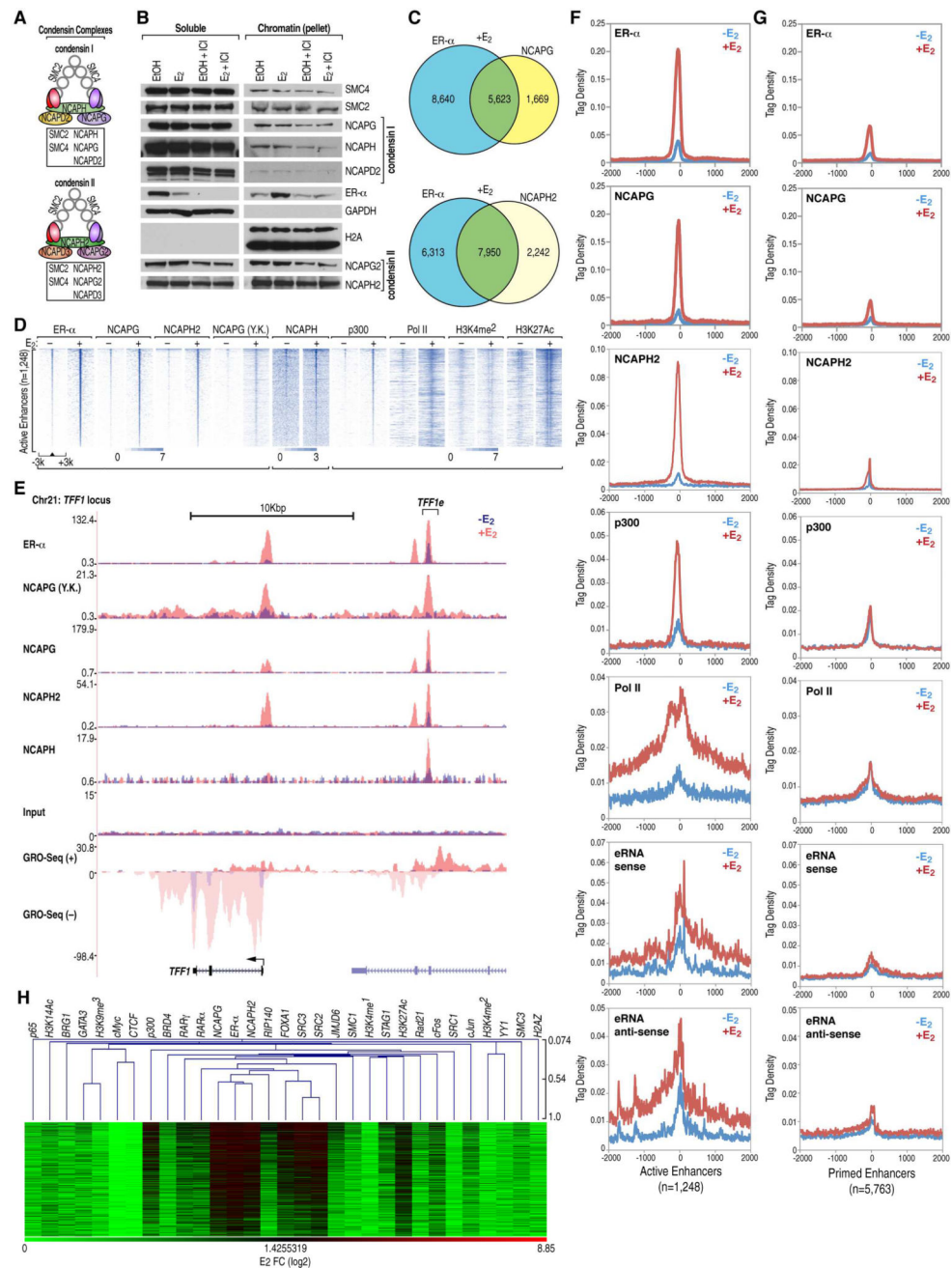
Figure 1. Estrogen-induced loading of condensins to ER- \alpha -bound active enhancers (A) A cartoon diagram showing the subunit constituents of the condensin I and condensin II complexes. (B) Chromatin fractionation followed by Western blots showing the localization of condensin subunits in MCF-7 cells upon E 2 or ICI treatment. (C) Venn diagram showing the genome-wide ChIP-Seq peak numbers of NCAPG and NCAPH2, and their overlap with that of ER- \alpha in E 2 -treated MCF-7 cells. (D) Heatmaps showing ChIP-Seq data of condensin I (NCAPG, NCAPH, NCAPG (Y.K.)) and condensin II (NCAPH2) together with p300, RNA Pol II, active histone marks H3K4me 2 and H3K27Ac on active enhancers (n=1,248) in MCF-7 cells (-/+E 2 , with scales indicated. The map was sorted vertically by the binding
