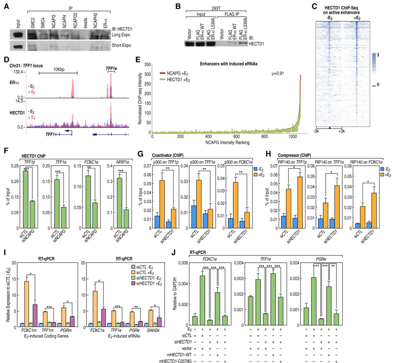
Figure 6. Condensin-dependent recruitment of HECTD1 is required for E 2 -induced eRNA activation
