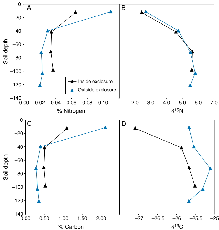
Fig. 4. Profiles of weight % N (A) and \delta^{15}\text{N} values (B) of soil nitrogen, and weight % (C) and \delta^{13}\text{C} values (D) of soil carbon, both outside (blue triangles) and inside (black triangles) of deer exclosures. Values are for depth ranges in Data S3 and reported for the midpoint depth of each range.
