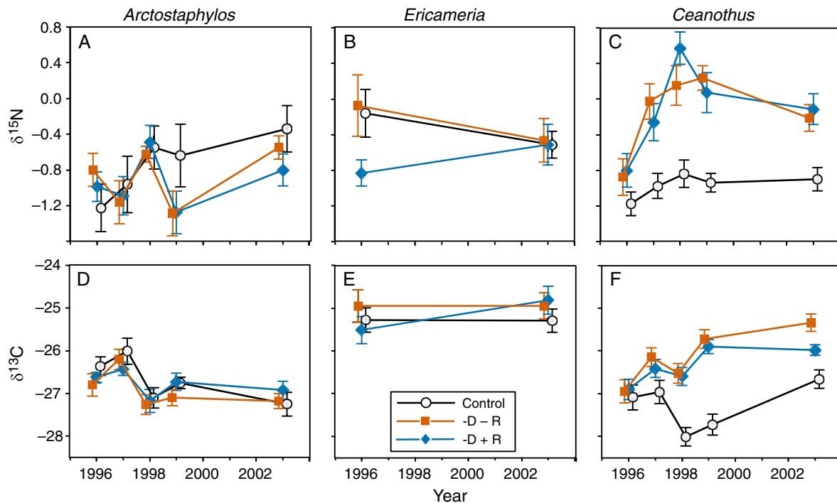
Fig. 2. Changes in foliar \delta^{15}\text{N} (A–C) and \delta^{13}\text{C} (D–F) values for N-fixing shrubs, Ceanothus rigidus , and adjacent non-fixing shrubs, Ericameria ericoides and Arctostaphylos pumila , for seven years of a field experiment that excluded only deer (–D+R, blue diamonds) or both deer and rabbits (–D–R, orange squares) from some plots. Controls are +D+R (black open circles). Data are \bar{x} \pm \text{SE} .
