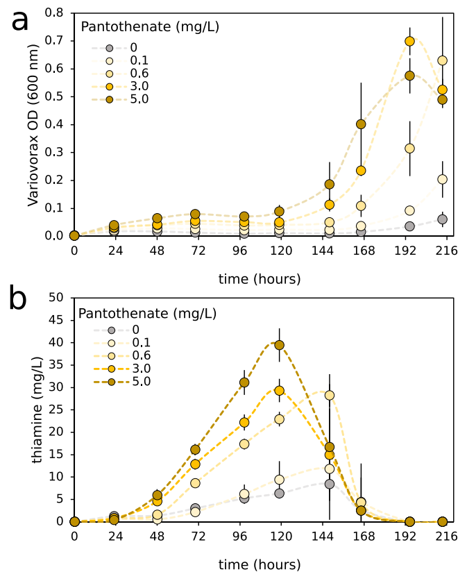
Fig. 7 | Variovorax produces thiamine during lag-phase and consumes extracellular thiamine during exponential growth. Growth, measured by optical density (OD), of Variovorax ( a ) and its thiamine production ( b ) when grown in M9 minimal media with the addition of varying concentrations of pantothenate (vitamin B5). Error bars represent one standard deviation from the mean of n = 4 biologically independent experiments.
