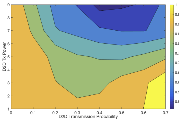
Figure 7: Contour plot for efficiency with respect to D2D transmission probability and D2D transmission power.
