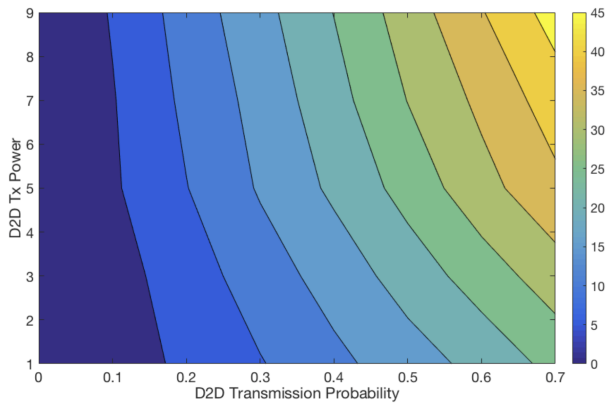
Figure 6: Contour plot for Object detection with respect to D2D transmission probability and D2D transmission power.
