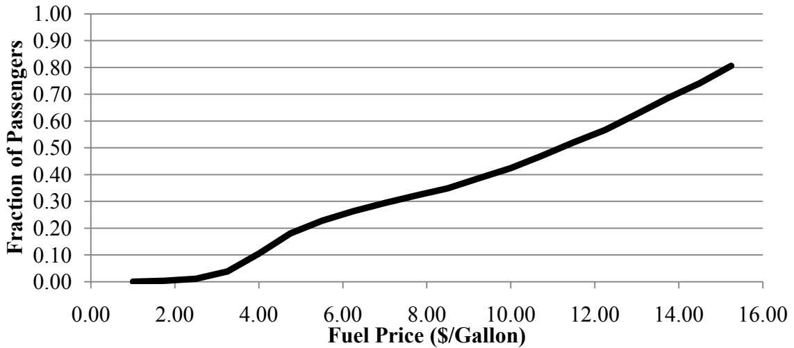
Figure 2.5 Potential fraction of passengers served on a turboprop for the lowest comparative total cost per passenger.
