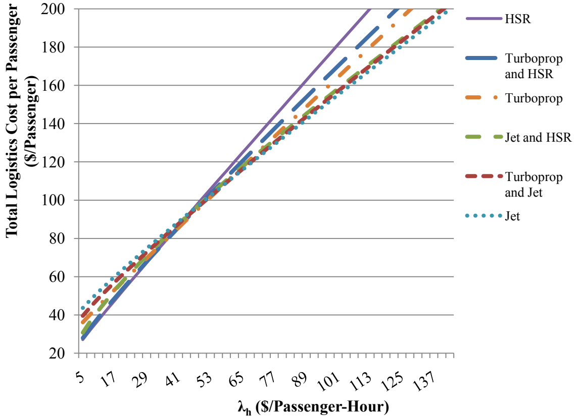
Figure 5.6 Total logistics cost vs. business passenger value of time.
