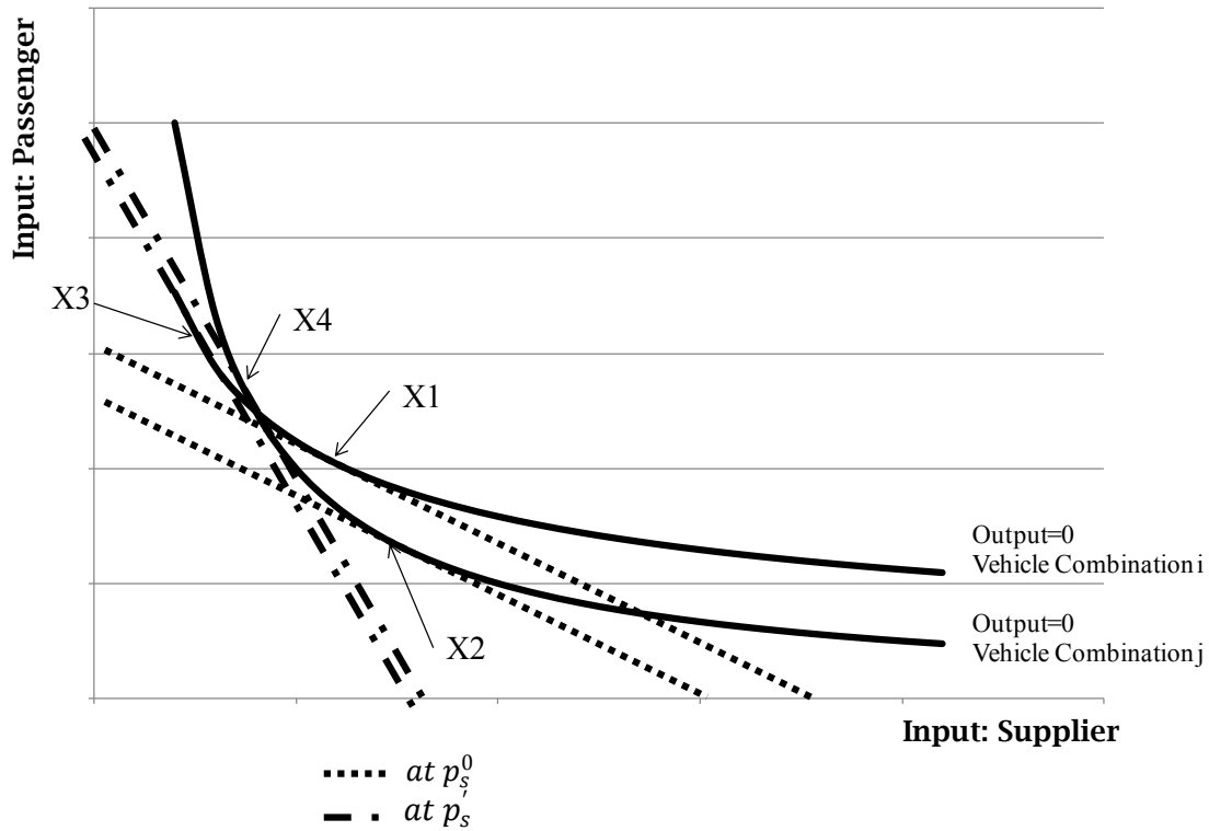
Figure 1.11 Illustration of input substitution and induced technological change.
