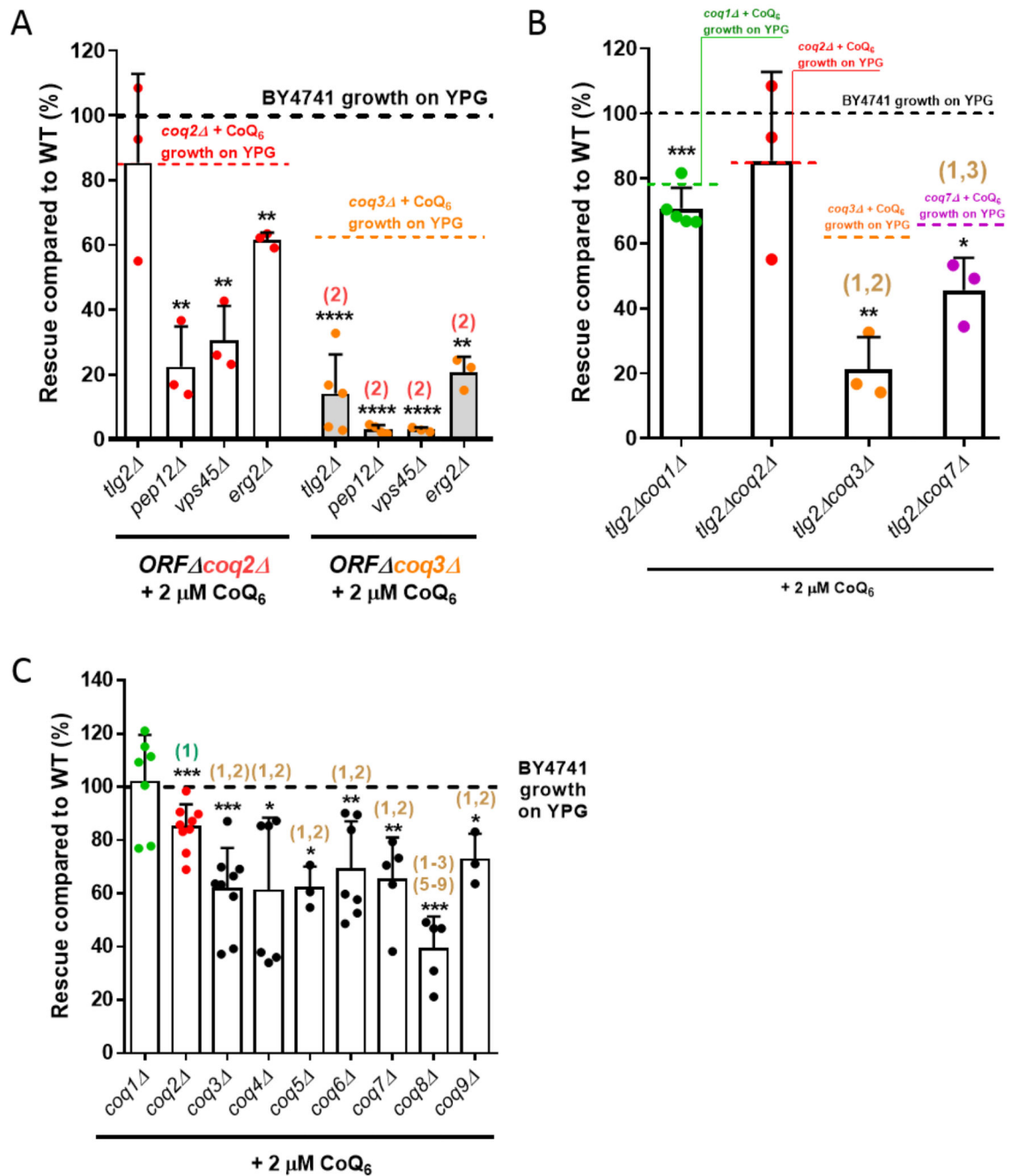
Figure 3. Yeast mutants harboring deletions in distinct COQ genes show different degrees of rescue in response to exogenously added CoQ 6 .
