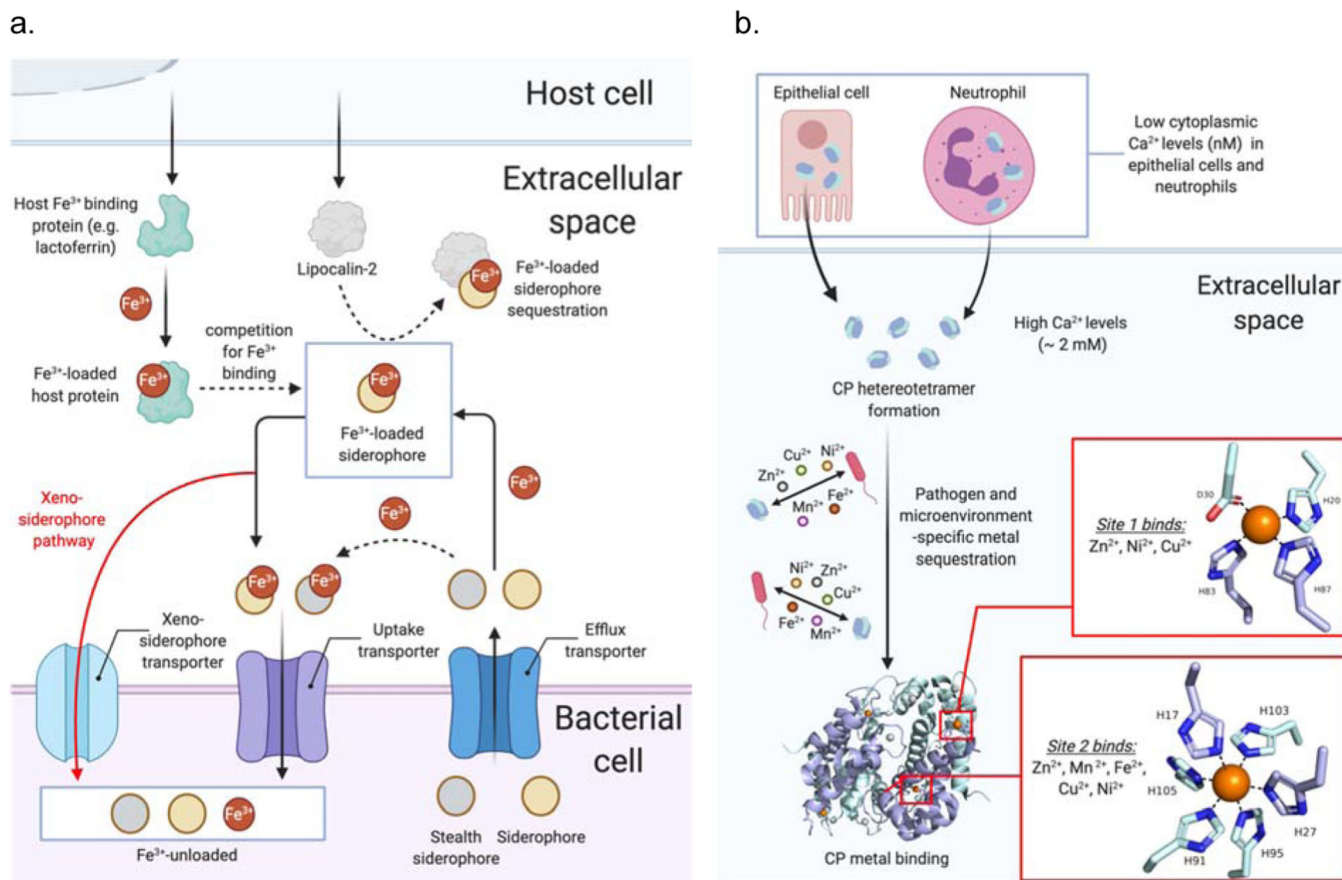
Figure 2. Iron and other metal ions during host-pathogen interaction. (a) Competition for \text{Fe}^{3+} resources is centered around bacterial siderophores and mammalian \text{Fe}^{3+} and siderophore-binding proteins. (b) Calprotectin (CP) is a general metal sequestering protein the binds \text{Fe}^{2+} and other divalent metal ions in the extracellular environment.
