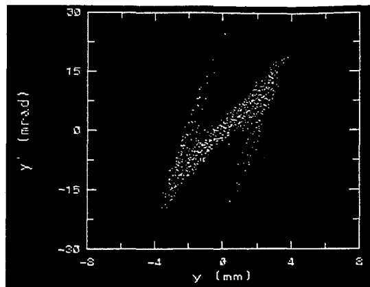
Figure 2: HIBEAM-predicted y - y' phase space at the M2 diagnostic location. This run was initialized with a semi-Gaussian phase space distribution.
