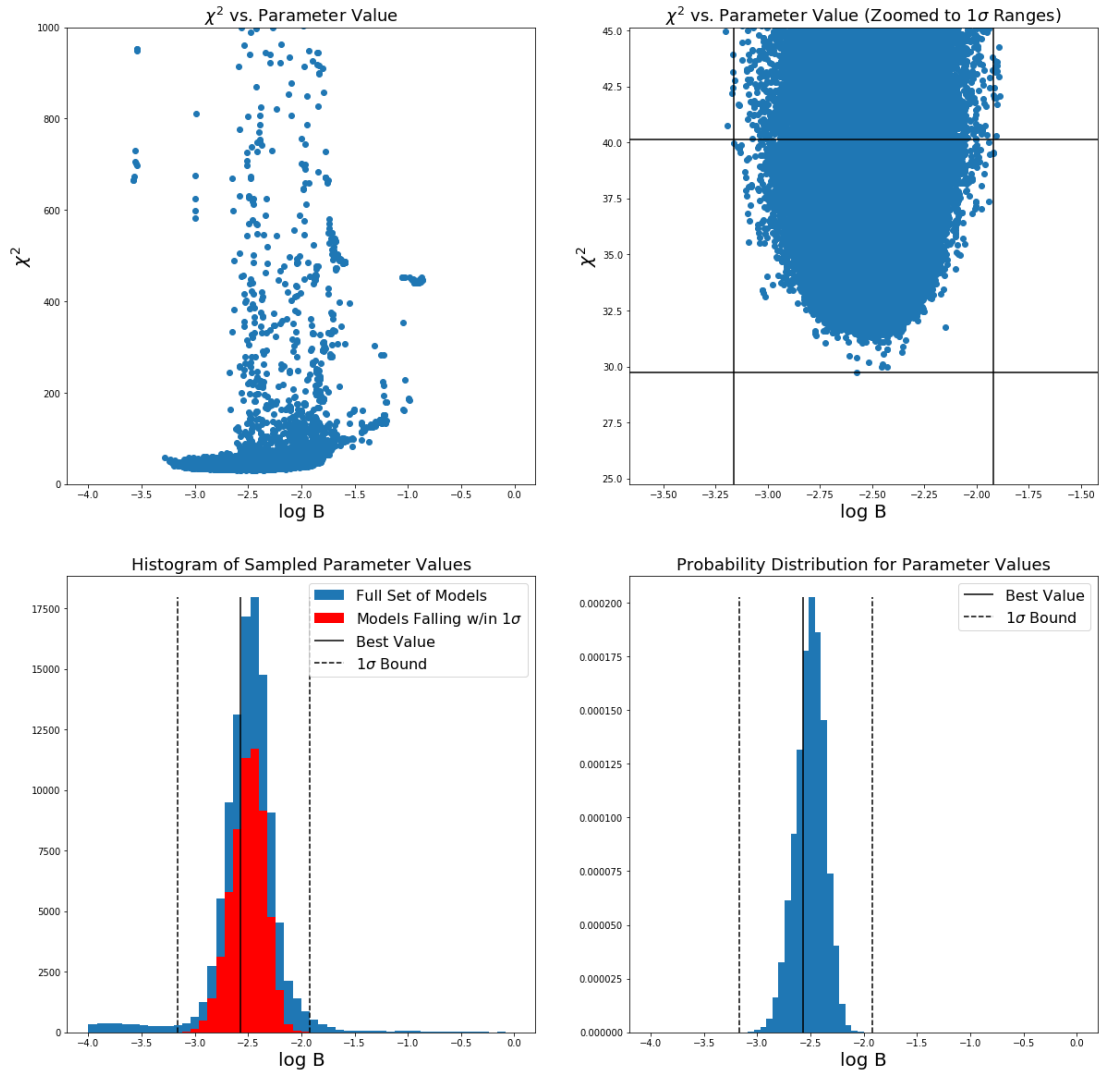
Figure A.11: Top left: \chi^2 value plotted as a function of the B value. Top right: \chi^2 vs. B value with the smallest \chi^2 value and largest \chi^2 1\sigma bounds shown as horizontal lines. The smallest and largest 1\sigma values of B are marked with vertical lines. Bottom left: Distribution of B values in the accepted steps. Bottom right: Non-normalized probability distribution for B.
