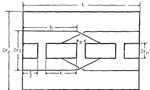
Fig. 2 L = 3/2 \lambda Cell
