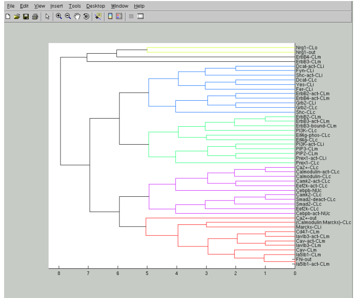
Figure 4: Hierarchical decomposition of one connected component of the composite graph using recursive spectral bisection. Each node in the dendrogram corresponds to a directed graph.
