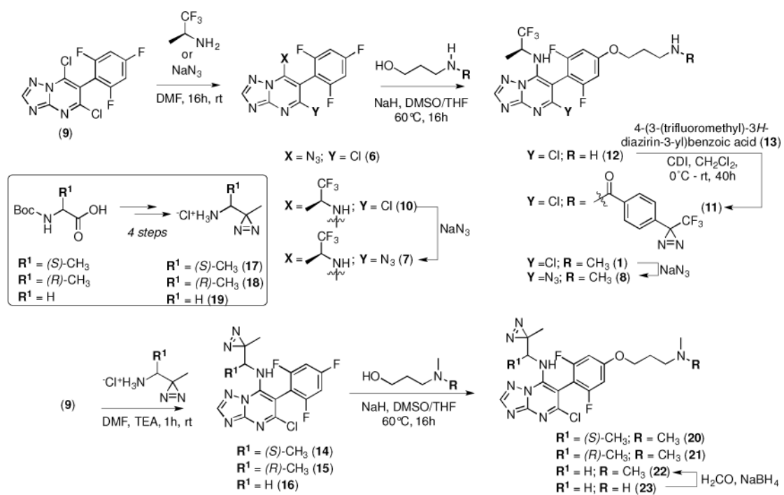
Scheme 1. Synthesis of triazolopyrimidine derivatives.
