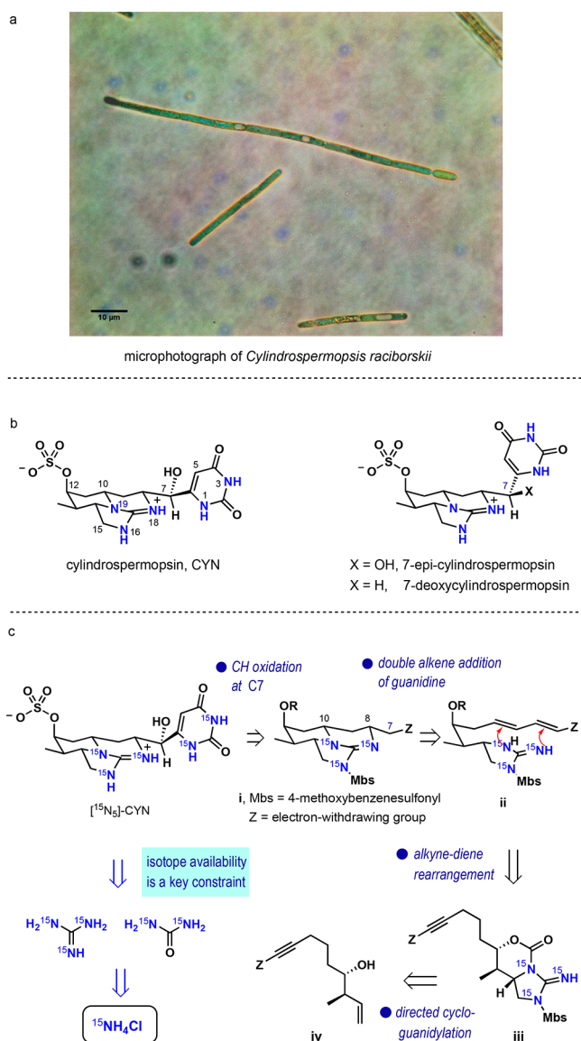
Figure 1. (a) A confocal optical microscopy image of Cyindrospermopsis raciborskii , (b) the structures of cyindrospermopsins, and (c) the outline of the synthetic design for ^{15}\text{N}_3 -CYN.
