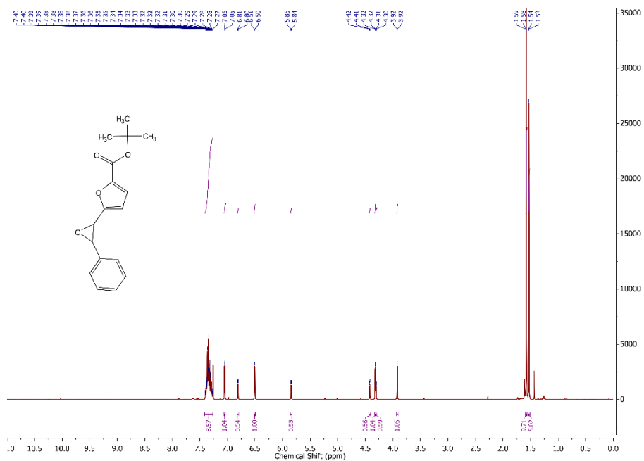
^1\text{H} NMR spectrum of cis - and trans - tert -butyl 5-(3-phenyloxiran-2-yl)furan-2-carboxylate (mixture, cis -29 and trans -29 ) in \text{CDCl}_3
