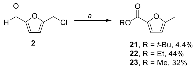
Scheme 2.5 - The NHC-catalyzed synthesis of 5-methylfuran-2-carboxylates. Reagents and conditions: a . 1,3-dimethylimidazolium iodide, DBU, ROH.
