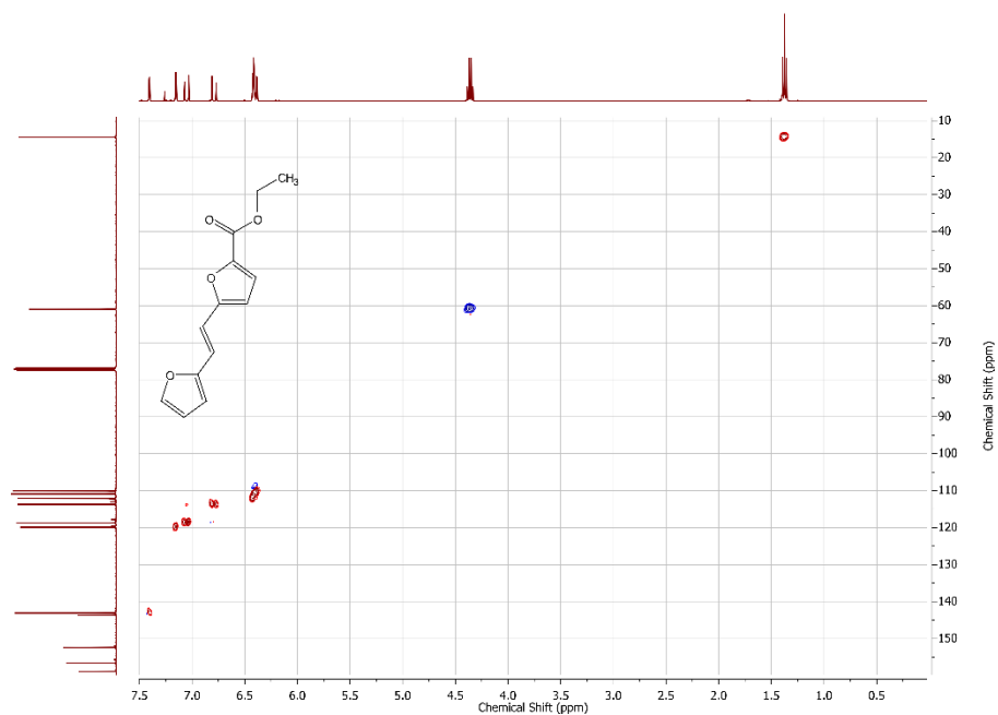
^1\text{H} - ^{13}\text{C} HSQC NMR spectrum of ethyl ( E )-5-(2-(furan-2-yl)vinyl)furan-2-carboxylate 63 in \text{CDCl}_3
