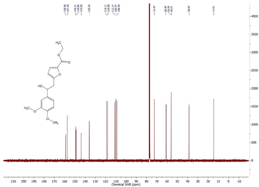
13 C NMR spectrum of ethyl 5-(2-(3,4-dimethoxyphenyl)-2-hydroxyethyl)furan-2-carboxylate 47 in CDCl 3
