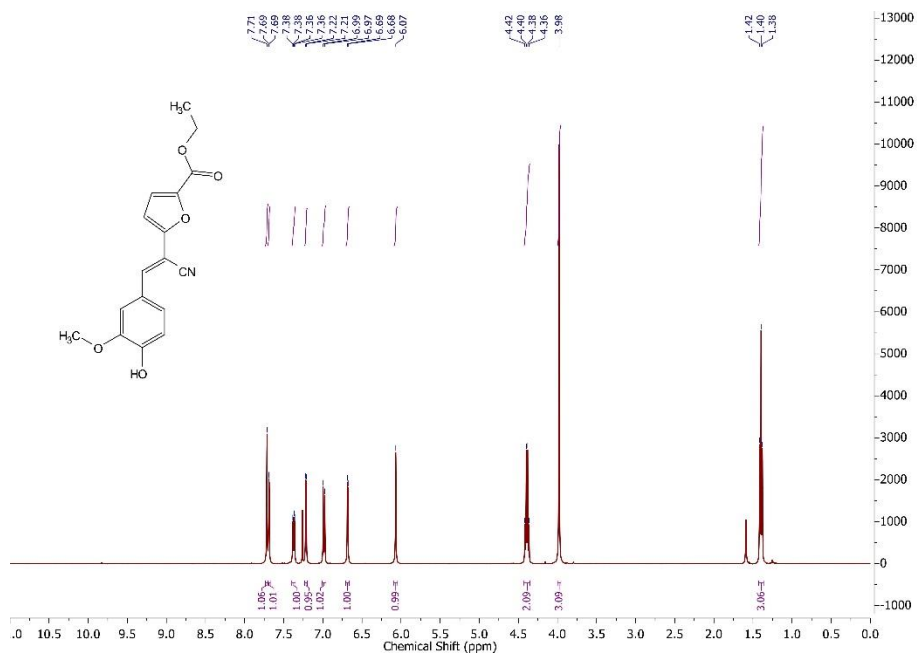
1 H NMR spectrum of ethyl (E)-5-(1-cyano-2-(4-hydroxy-3-methoxyphenyl)vinyl)furan-2-carboxylate 73a in CDCl 3 .
