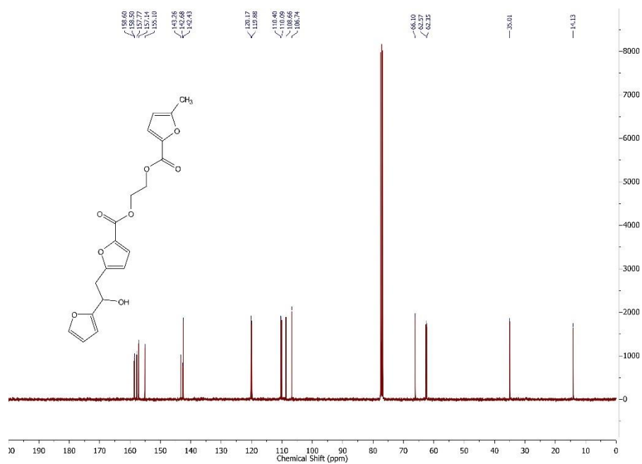
13 C NMR spectrum of 2-((5-(2-(furan-2-yl)-2-hydroxyethyl)furan-2-carbonyl)oxy)ethyl 5-methylfuran-2-carboxylate 59 in CDCl 3
