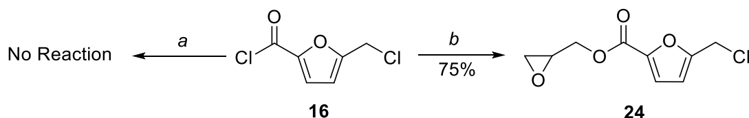
Scheme 2.6 - Synthesis of oxiran-2-ylmethyl 5-(chloromethyl)furan-2-carboxylate 24 . Reagents and conditions: a . glycidol, K 2 CO 3 , THF, rt, 2 h. b . glycidol, Et 3 N, DCM, 0 °C to rt, 3.5 h, 75%.
