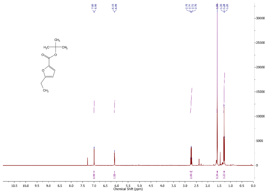
1 H NMR spectrum of tert -butyl 5-ethylfuran-2-carboxylate 31 in CDCl 3
