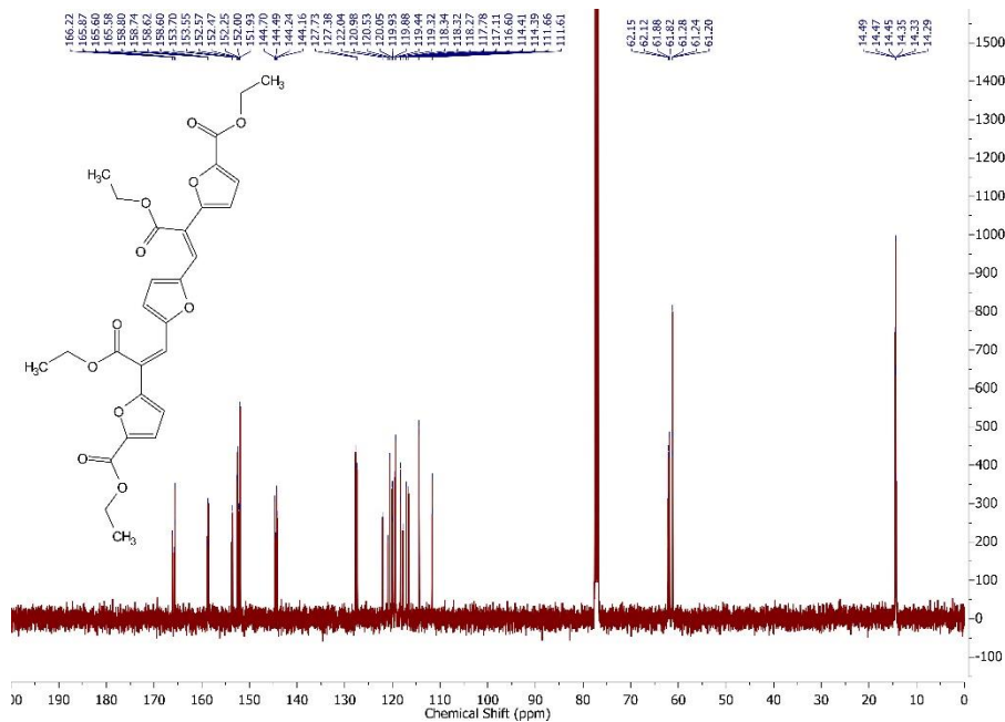
^{13}\text{C} NMR spectrum of mixture of diethyl 5,5'-((1Z,1'Z)-furan-2,5-diylbis(3-ethoxy-3-oxoprop-1-ene-1,2-diyl))bis(furan-2-carboxylate) and stereoisomer 79b in \text{CDCl}_3 .
