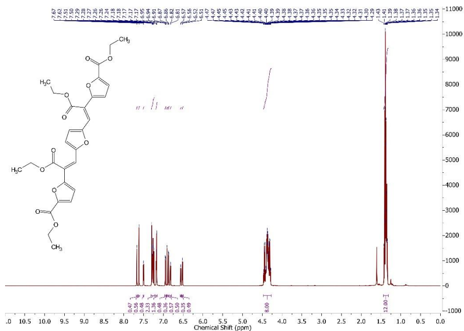
^1\text{H} NMR spectrum of the mixture of diethyl 5,5'-((1Z,1'Z)-furan-2,5-diylbis(3-ethoxy-3-oxoprop-1-ene-1,2-diyl))bis(furan-2-carboxylate) and stereoisomer 79b in \text{CDCl}_3 .
