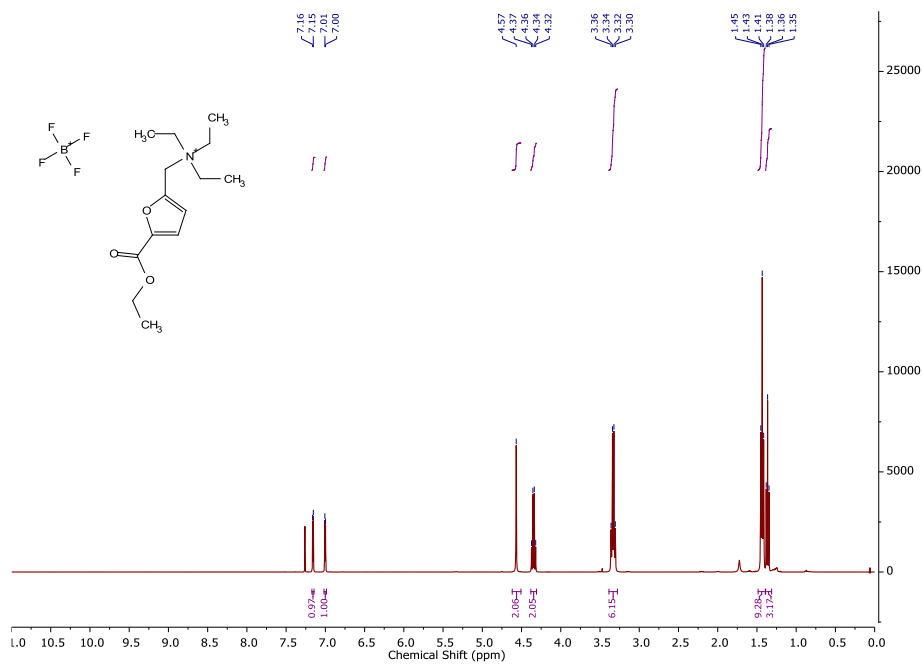
1 H NMR spectrum of N-((5-(ethoxycarbonyl)furan-2-yl)methyl)-N,N-diethylethanaminium tetrafluoroborate 41 in CDCl 3
