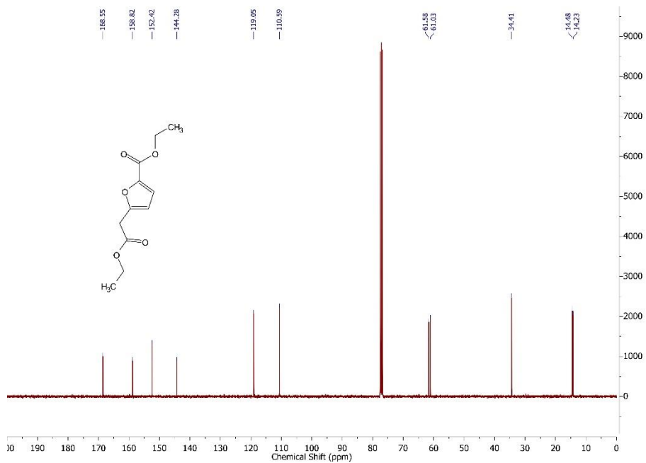
^{13}\text{C} NMR spectrum of ethyl 5-(carboxymethyl)furan-2-carboxylate 69 in \text{CDCl}_3 .
