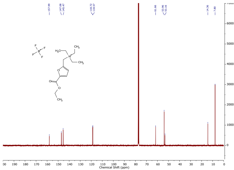
13 C NMR spectrum of N-((5-(ethoxycarbonyl)furan-2-yl)methyl)-N,N-diethylethanaminium tetrafluoroborate 41 in CDCl 3
