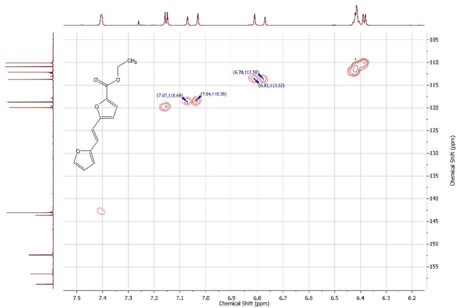
^1\text{H} - ^{13}\text{C} HSQC NMR spectrum of ethyl ( E )-5-(2-(furan-2-yl)vinyl)furan-2-carboxylate 63 in \text{CDCl}_3 (zoom in)
