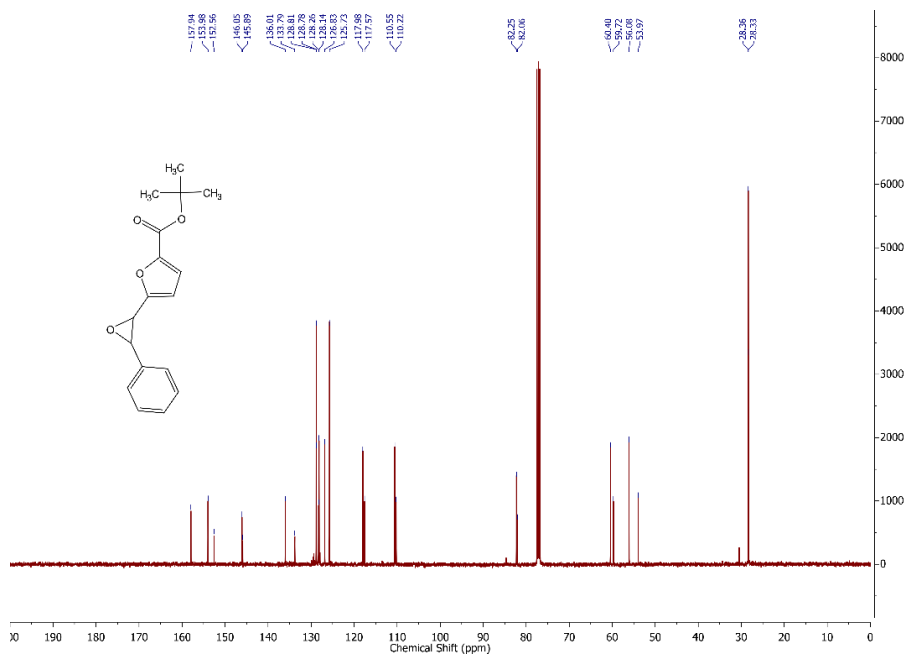
^{13}\text{C} NMR spectrum of cis - and trans - tert -butyl 5-(3-phenyloxiran-2-yl)furan-2-carboxylate (mixture, cis -29 and trans -29 ) in \text{CDCl}_3
