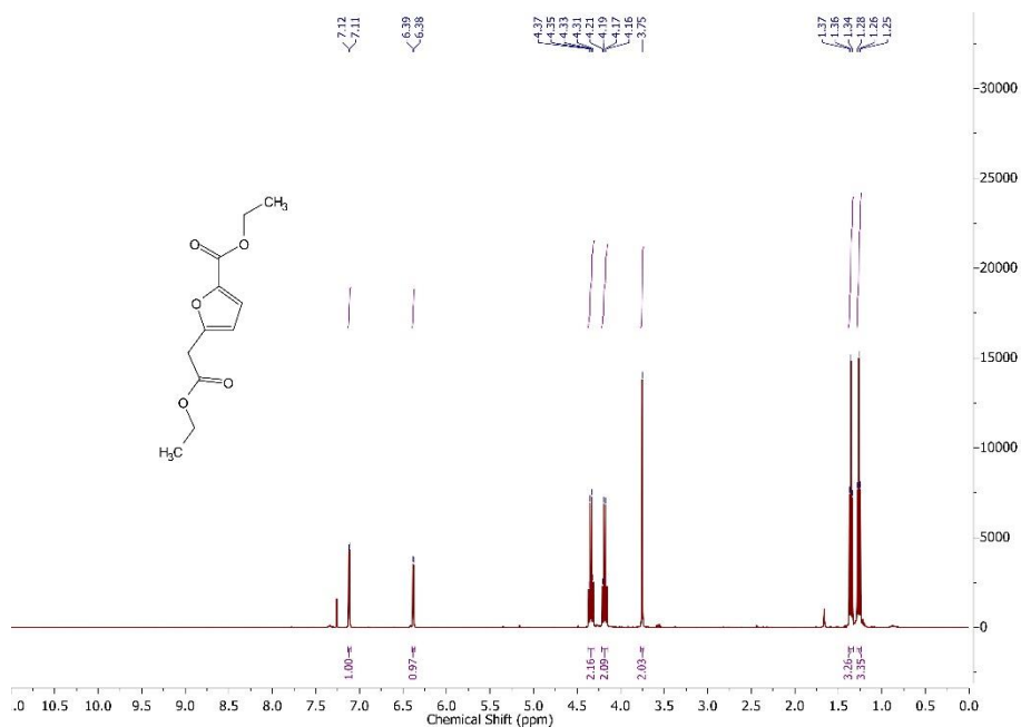
^1\text{H} NMR spectrum of ethyl 5-(carboxymethyl)furan-2-carboxylate 69 in \text{CDCl}_3 .
