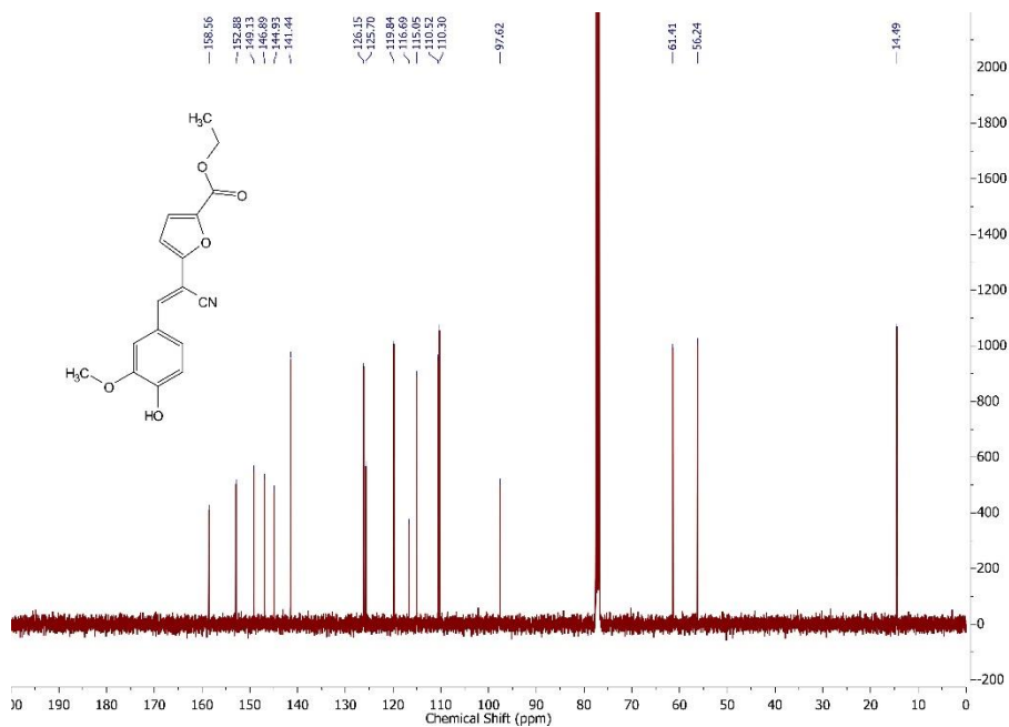
13 C NMR spectrum of ethyl (E)-5-(1-cyano-2-(4-hydroxy-3-methoxyphenyl)vinyl)furan-2-carboxylate 73a in CDCl 3 .
