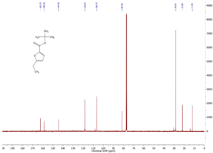
13 C NMR spectrum of tert -butyl 5-ethylfuran-2-carboxylate 31 in CDCl 3
