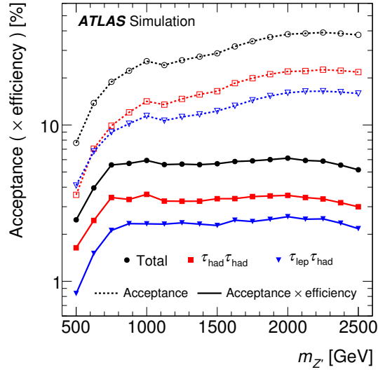
Figure 7. Acceptance (dashed lines with empty markers) and acceptance times efficiency (solid lines with filled markers) for Z'_{SSM} as a function of the Z'_{SSM} mass. Contributions from the individual channels and the full analysis are given.
