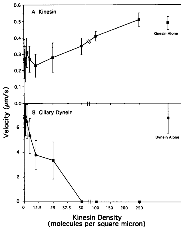
Figure 4. The velocities of kinesin (A) and ciliary dynein (B) motility at different kinesin densities on a ciliary dynein coated surface. The squares indicate the mean and the error bars represent the standard deviations of velocity measurements from between 10 and 40 microtubules. These data were derived from the same experiment shown in Fig. 3. At kinesin densities where bidirectional motion predominated, the plus- and minus-end directed velocities were approximately one-half of those elicited by kinesin or ciliary dynein alone.
