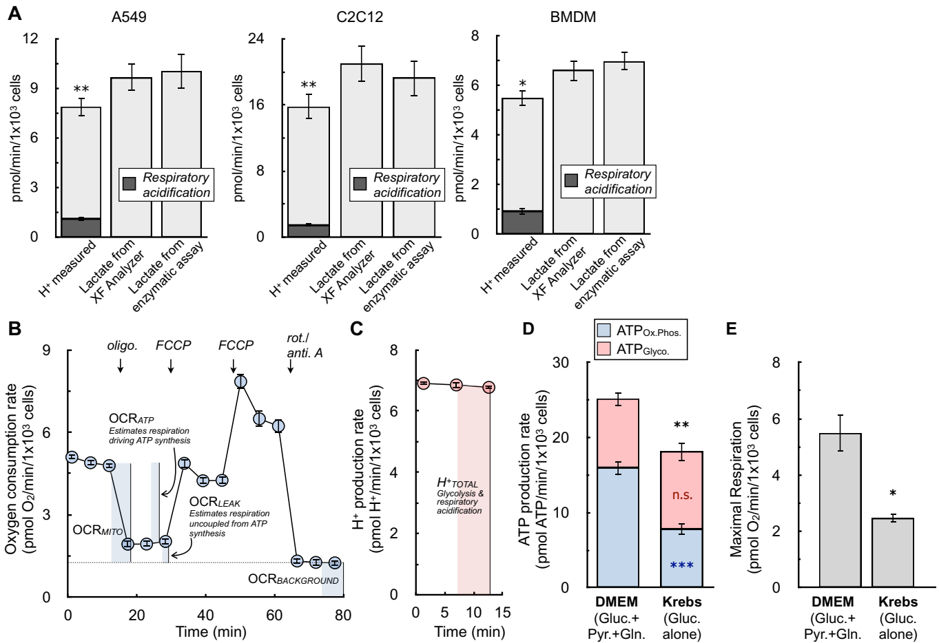
Figure 3. Transformation of ECAR into lactate efflux allows calculation of ATP production rates.
