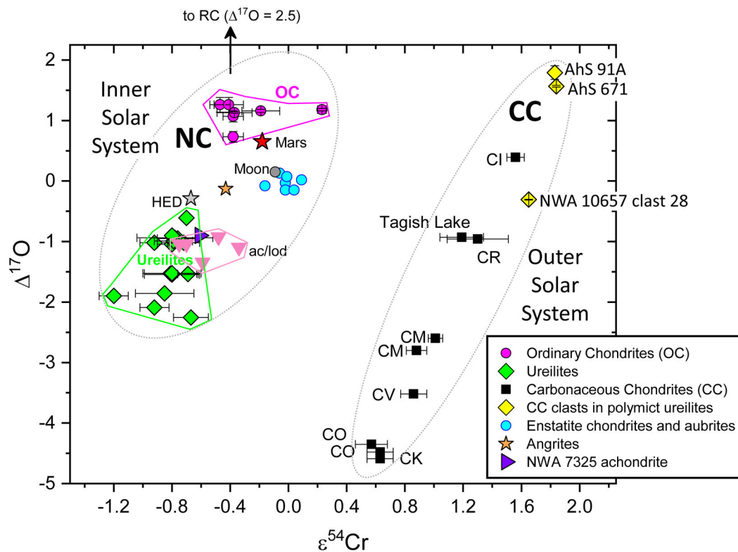
Figure 1. Plot of \epsilon^{54}\text{Cr} vs. \Delta^{17}\text{O} , on which solar system materials show a stark dichotomy between the CC suite consisting mainly of carbonaceous chondrites (plus some differentiated meteorites not shown here) and the NC suite consisting of Earth, Moon, Mars, ordinary chondrites, enstatite chondrites, Rumuruti-type chondrites (RC) and most major groups of achondrites including angrites, acapulcoites and lodranites (ac/lod), and the howardite-eucrite-diogenite (HED) group. The currently prevailing interpretation of these two suites is that they correspond to materials that formed in the outer solar system vs. the inner solar system, respectively (Warren 2011; Kruijer et al. 2017). Polymict ureilites are NC breccias that contain xenoliths of carbonaceous chondrite-like materials. Chromium and oxygen isotope data obtained here for three such xenoliths (yellow diamonds) show that they are derived from the CC isotopic reservoir, providing ground truth evidence for mixing of bulk CC materials into NC asteroidal regoliths. Sources of data (alphabetical order): Clayton & Mayeda (1996, 1999); Clayton et al. (1984, 1991); Dauphas & Schauble (2016); Goodrich et al. (2017a); Jenniskens et al. (2012, 2014); Li et al. (2018); Popova et al. (2013); Qin et al. (2010); Rubin et al. (2002); Shukolyukov & Lugmair (2006); Trinquier et al. (2007); Ueda et al. (2006); Yamakawa et al. (2010).
