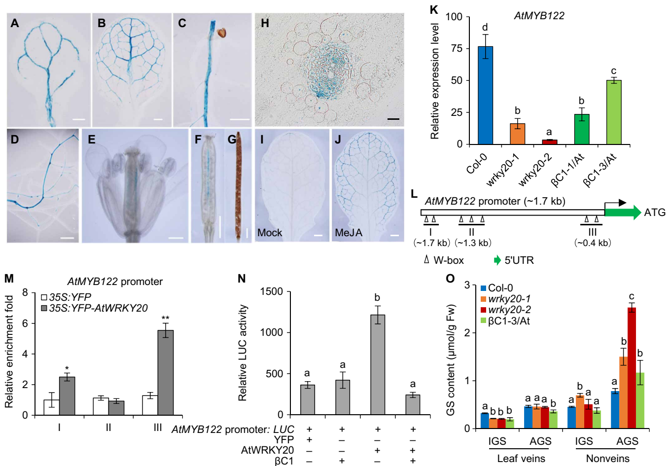
Fig. 4. \beta C1 regulates WRKY20-mediated GS biosynthesis in a vascular-specific manner. (A to G) AtWRKY20 promoter activity in a cotyledon (A), first rosette leaf (B), roots (C and D), inflorescence (E), and siliques (F and G). Scale bars, 1 mm. (H) Resin root slice of the AtWRKY20 promoter: GUS lines. Scale bars, 20 \mu m. (I and J) GUS staining of the leaves of 6-week-old plants before (I) and after (J) MeJA treatment in AtWRKY20 promoter: GUS lines. Scale bars, 2 mm. (K) Relative expression level of AtMYB122 in 6-week-old Arabidopsis plants after 6 hours MeJA treatment. Bars represent means \pm SD ( n = 3 ). (L) Schematic diagram of the AtMYB122 promoter. The small hollow triangles represent W-box motifs in the schematic diagram of the promoters. ATG indicates the coding initiation site of a gene. Three lines under triangles represent various DNA fragments were amplified in ChIP assay. (M) Fold enrichment of YFP- AtWRKY20 associated with DNA fragments of the AtMYB122 promoter in a ChIP assay. Enrichments are referred to the 35S:YFP- AtWRKY20 or 35S:YFP against wild-type Col-0 seedlings. Bars represent means \pm SD ( n = 4 ) (* P < 0.05 and ** P < 0.01 , Student's t test). (N) Effects of \beta C1 on the transactivation activity of AtWRKY20 on the AtMYB122 promoter. Bars represent means \pm SD ( n = 8 ). (O) Contents of AGS and IGS in leaf veins and nonveins, respectively, of 6-week-old Arabidopsis plants after 6 hours of MeJA treatment. Bars represent means \pm SD ( n = 4 ). (K, N, and O) Means with different letters (a, b, c, and d) are significantly different ( P < 0.05 , one-way ANOVA along with Duncan's multiple range test). Photo credit: Pingzhi Zhao, Chinese Academy of Sciences.
