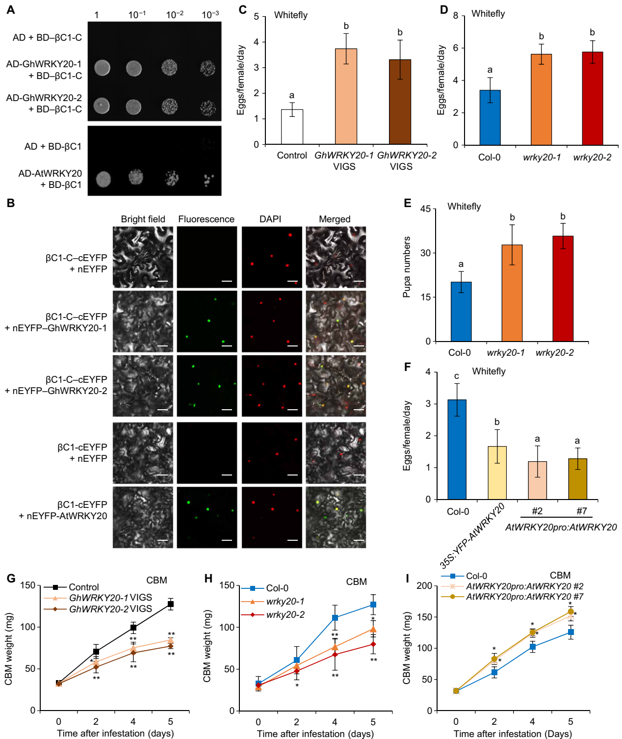
Fig. 2. Begomovirus-encoded βC1 proteins interact with plant WRKY20 proteins for differentiated resistance against herbivores. (A) Interaction of CLCuMuV βC1 (βC1-C) with GhWRKY20 homologs (GhWRKY20-1 and GhWRKY20-2) and TYLCCNV βC1 with AtWRKY20 in a yeast two-hybrid system. (B) BiFC analysis of βC1 proteins interaction with WRKY20 homologous proteins. Scale bars, 50 μm. (C and D) Daily number of eggs laid per female whitefly on vector control cotton and VIGS cotton silenced for GhWRKY20 (C) or on Arabidopsis Col-0 and wrky20 mutant plants (D). (E) Pupa numbers of whiteflies present on Arabidopsis Col-0 and wrky20 mutant plants. (F) Daily number of eggs laid per female whitefly on Arabidopsis Col-0 and overexpressing AtWRKY20 plants. (G to I) Larval weight of CBM reared on vector control cotton and GhWRKY20 VIGS cotton (G) on Col-0 and wrky20 mutant plants (H) or on Col-0 and plants overexpressing AtWRKY20 (I). (C to F) Bars represent means ± SD ( n = 8). Means with different letters (a, b, and c) are significantly different [ P < 0.05, one-way analysis of variance (ANOVA) along with Duncan's multiple range test]. (G to I) Bars represent means ± SD ( n = 10) (* P < 0.05 and ** P < 0.01, Student's t test).
